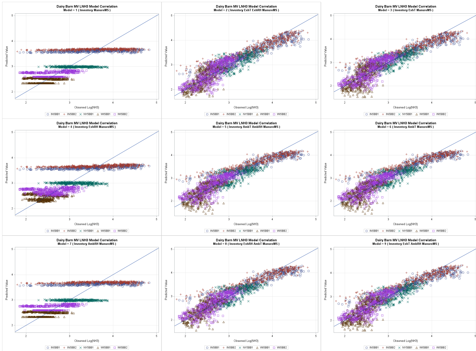
Figure G-1. Dairy mechanically ventilated barn NH 3 one-to-one plots models 1 through 9, log transformed.
