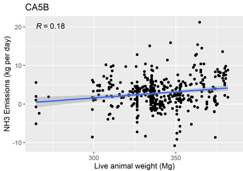
Figure F-91. Scatter plot of naturally ventilated barns NH 3 emissions versus live animal weight and scatter plot with regression.
