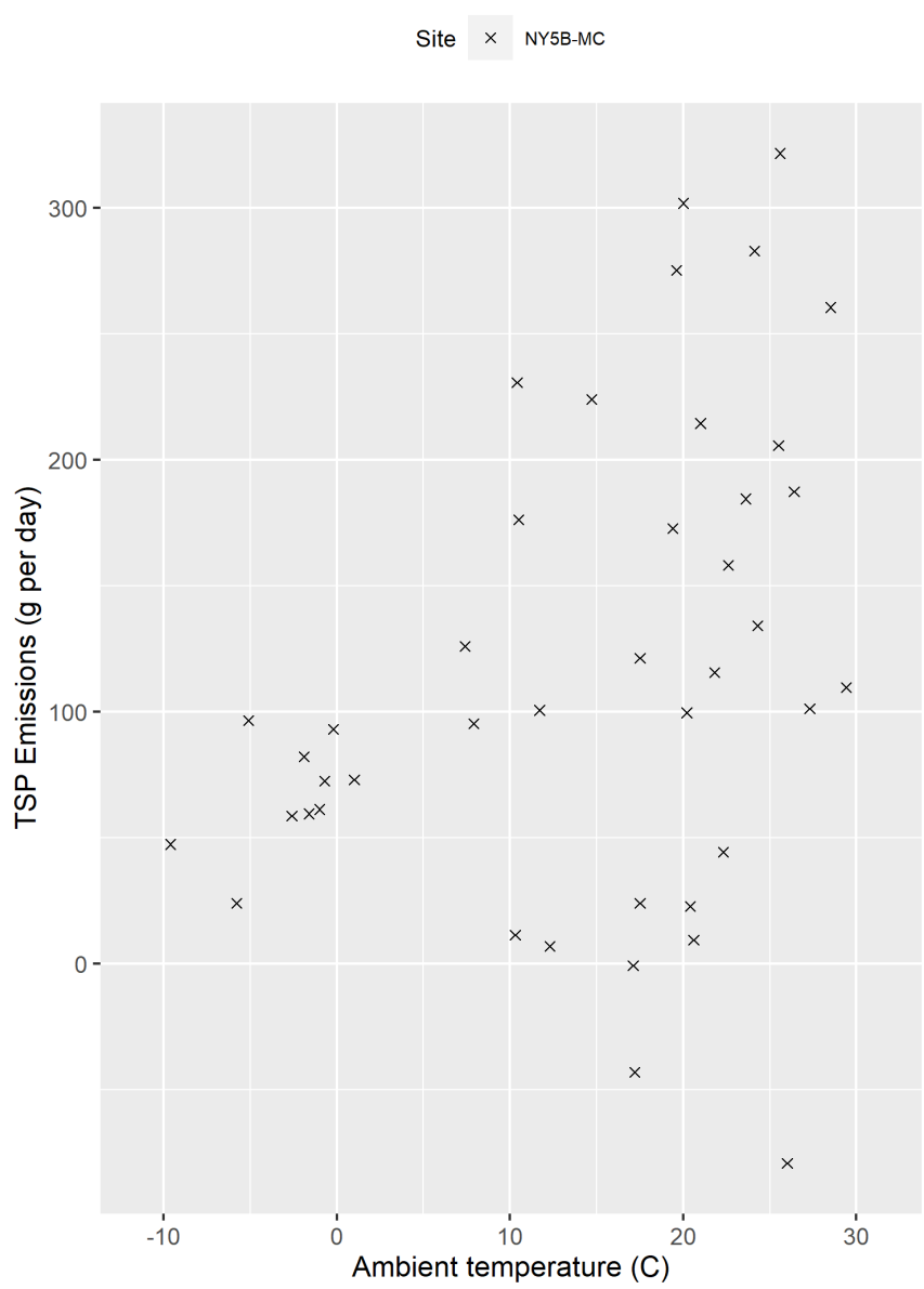
Figure F-75. Scatter plot of milking center TSP emissions versus ambient temperature and scatter plot with regression.
