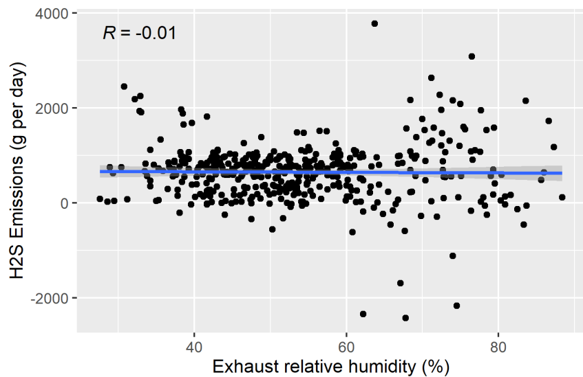
Figure F-102. Scatter plot of naturally ventilated barns H 2 S emissions versus exhaust relative humidity and scatter plot with regression.
