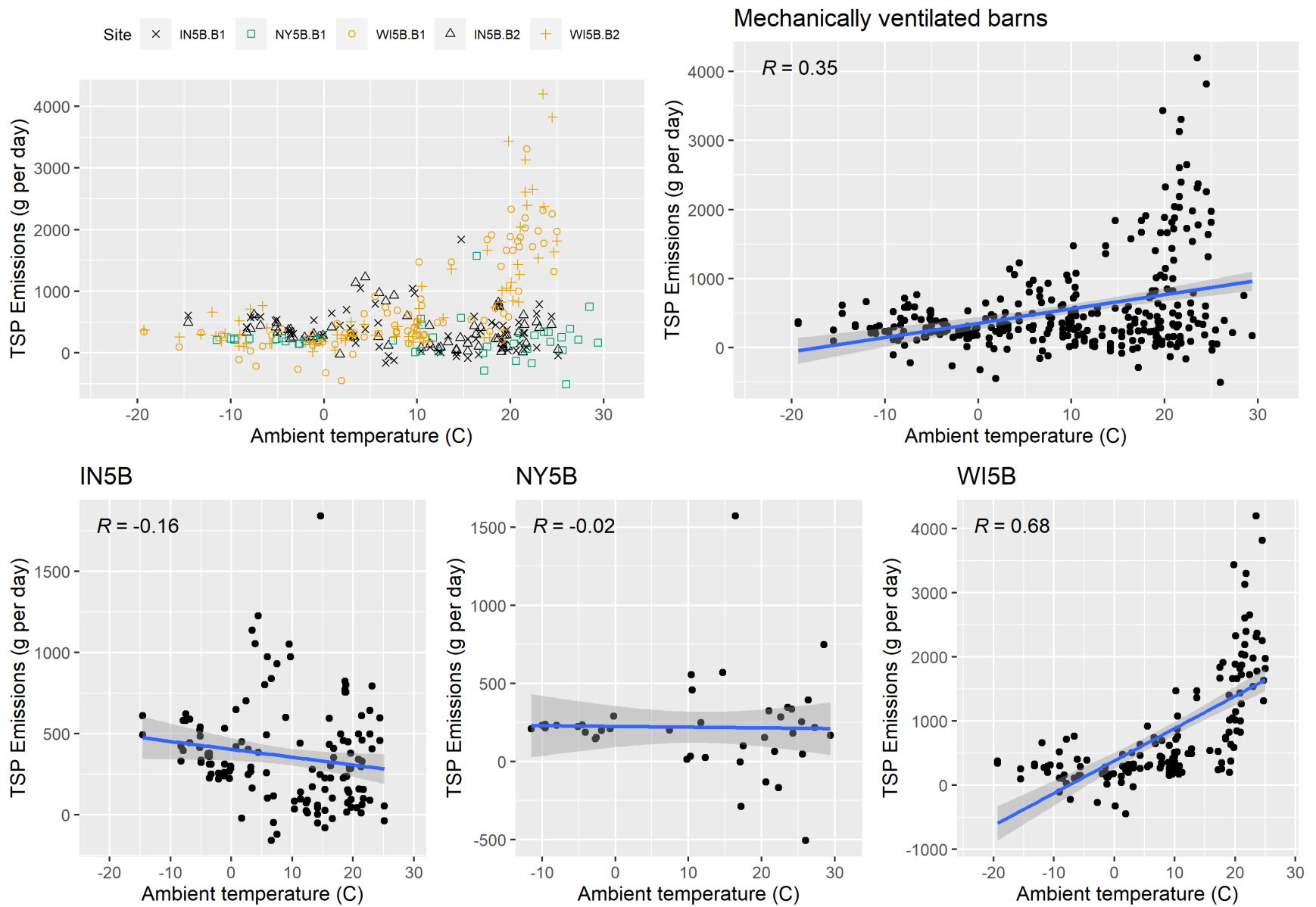
Figure F-35. Scatter plot of mechanically ventilated TSP emissions versus ambient temperature and scatter plot with regression.
