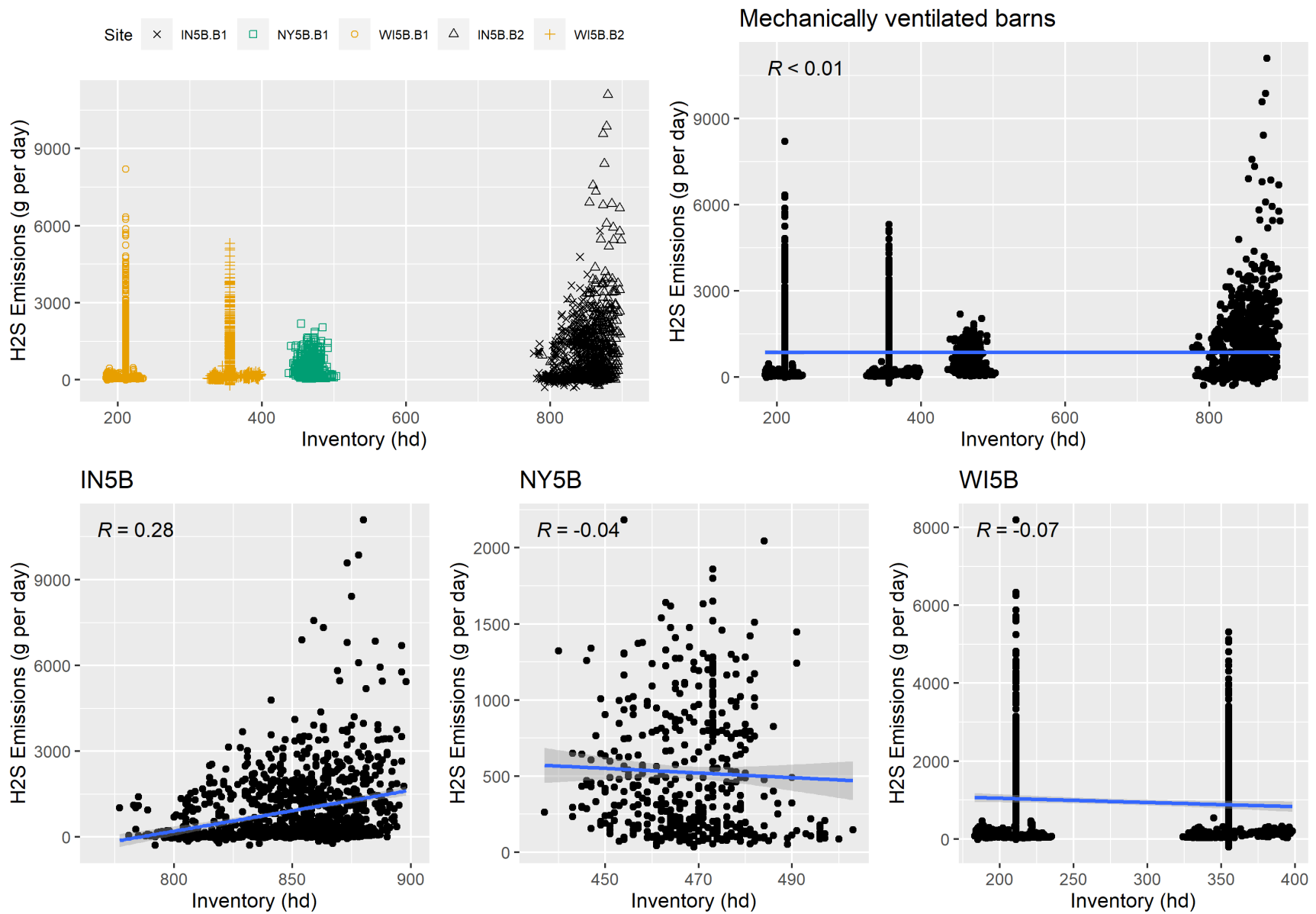
Figure F-2. Scatter plot of mechanically ventilated H 2 S emissions versus inventory and scatter plot with regression.
