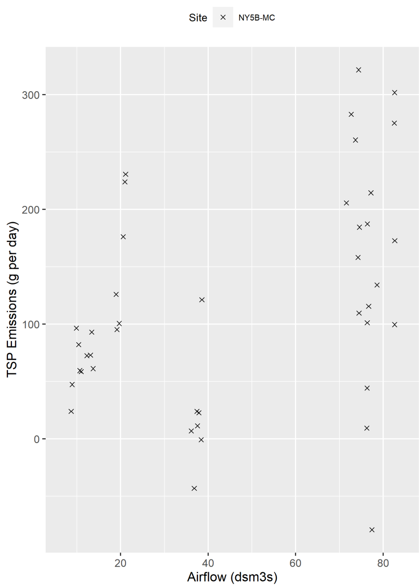
Figure F-70. Scatter plot of milking center TSP emissions versus airflow and scatter plot with regression.
