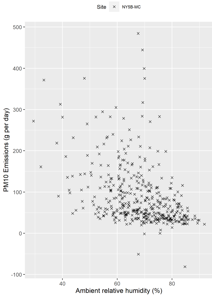
Figure F-78. Scatter plot of milking center PM 10 emissions versus ambient relative humidity and scatter plot with regression.
