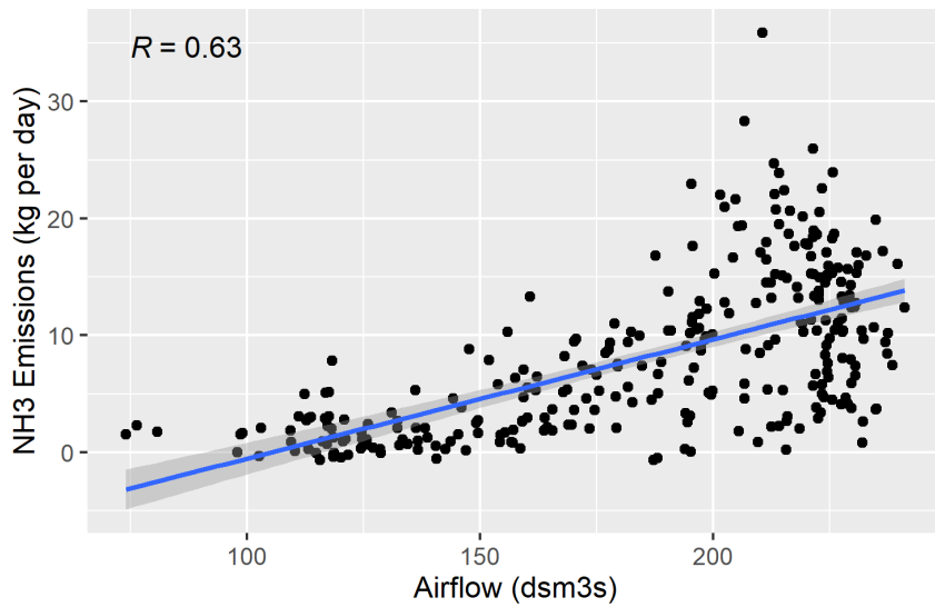
Figure F-66. Scatter plot of milking center NH 3 emissions versus airflow and scatter plot with regression.
