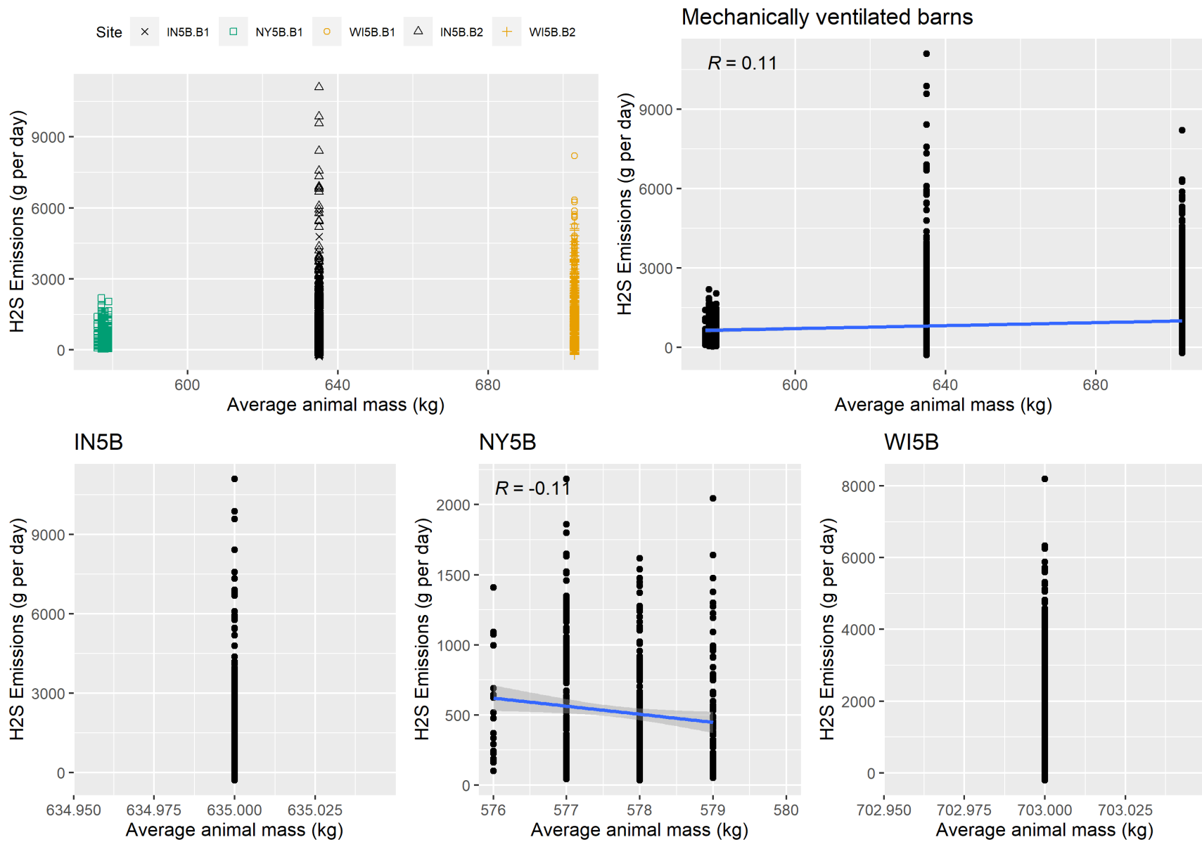
Figure F-7. Scatter plot of mechanically ventilated H 2 S emissions versus average animal mass and scatter plot with regression.
