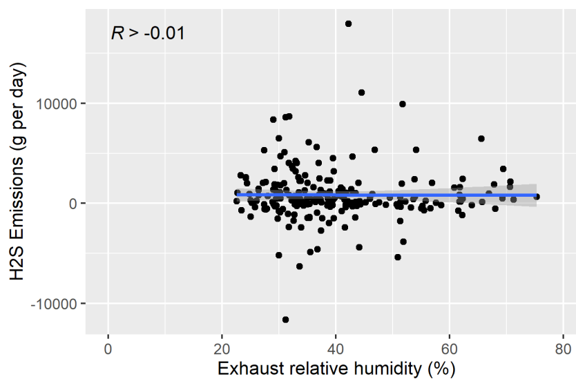
Figure F-102. Scatter plot of naturally ventilated barns H 2 S emissions versus exhaust relative humidity and scatter plot with regression.
