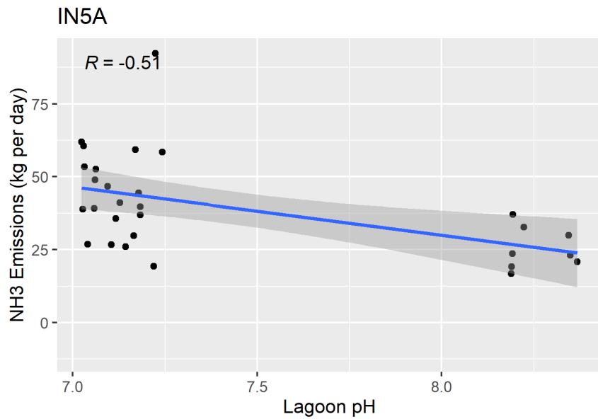
Figure F-128. Scatter plot of lagoon/basin NH 3 emissions versus lagoon pH and scatter plot with regression.
