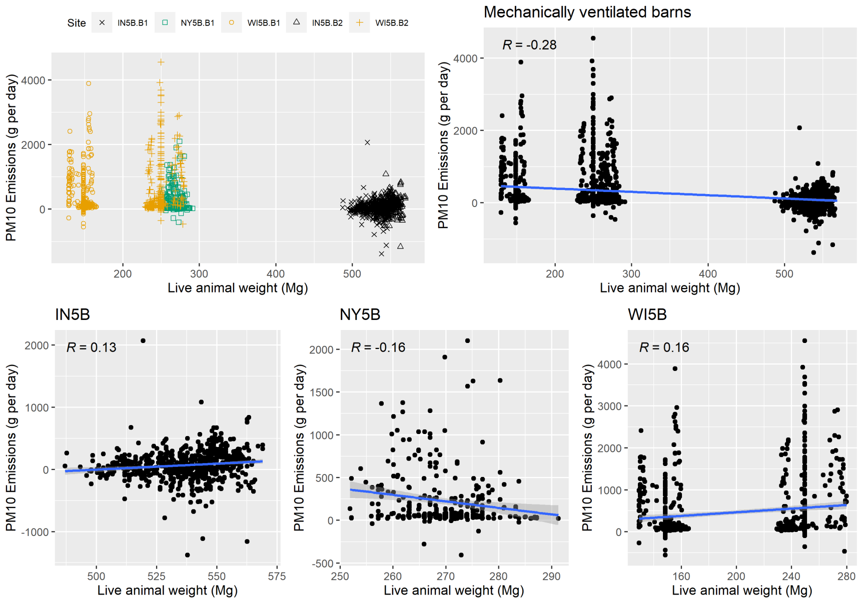
Figure F-13. Scatter plot of mechanically ventilated PM 10 emissions versus live animal weight and scatter plot with regression.
