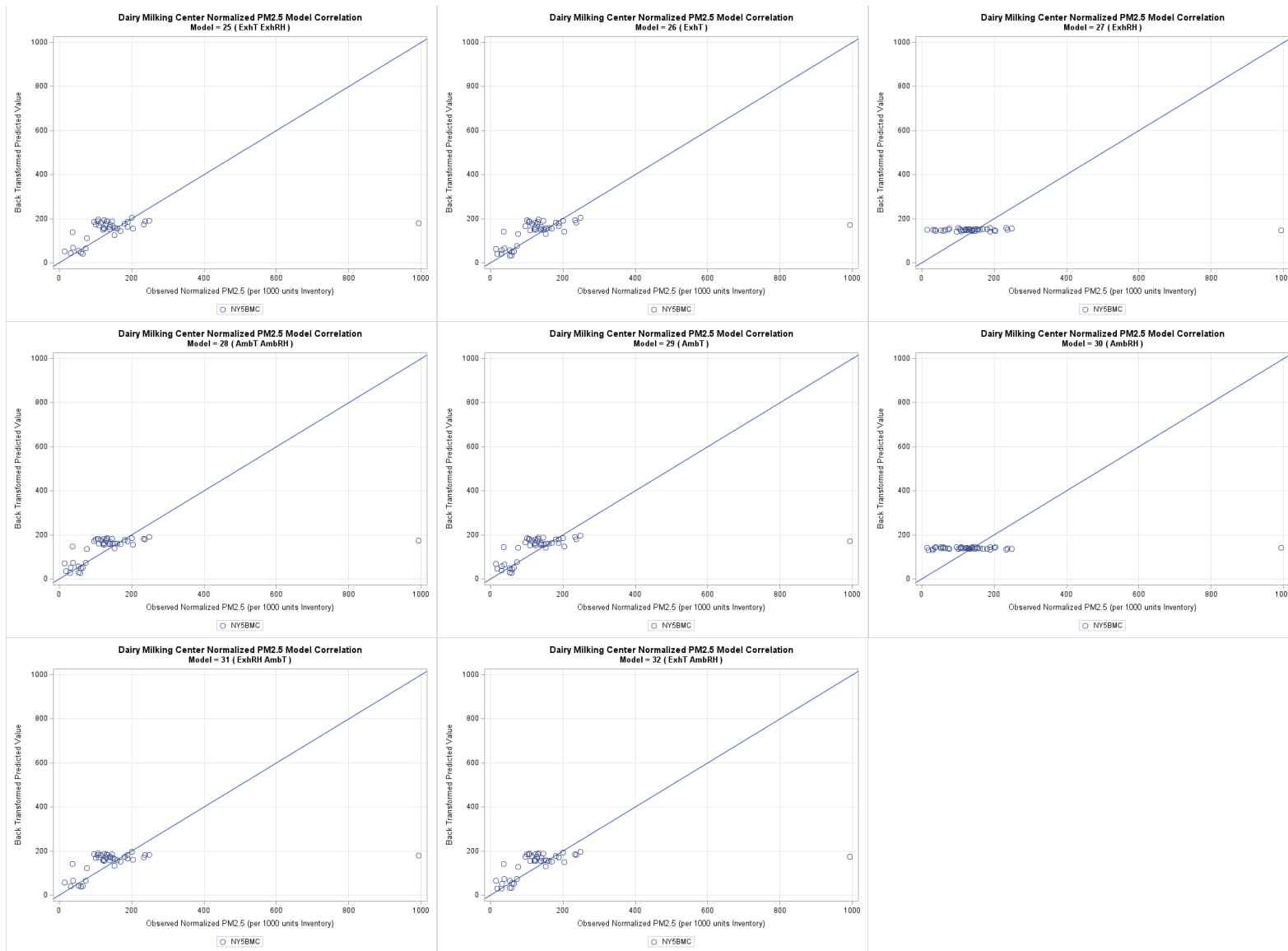
Figure G-48. Dairy milking center PM 2.5 one-to-one plots models 25 through 32, back transformed.
