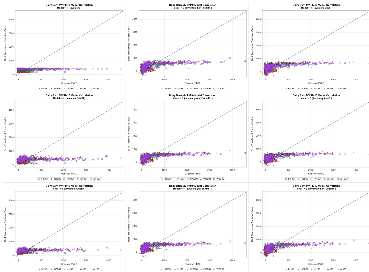
Figure G-7. Dairy mechanically ventilated barn PM 10 one-to-one plots models 1 through 9, back transformed.
