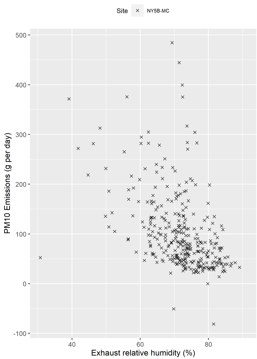
Figure F-63. Scatter plot of milking center PM 10 emissions versus exhaust relative humidity and scatter plot with regression.
