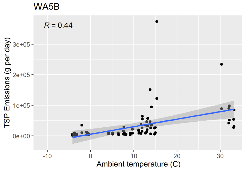
Figure F-115. Scatter plot of naturally ventilated barns TSP emissions versus ambient temperature and scatter plot with regression.
