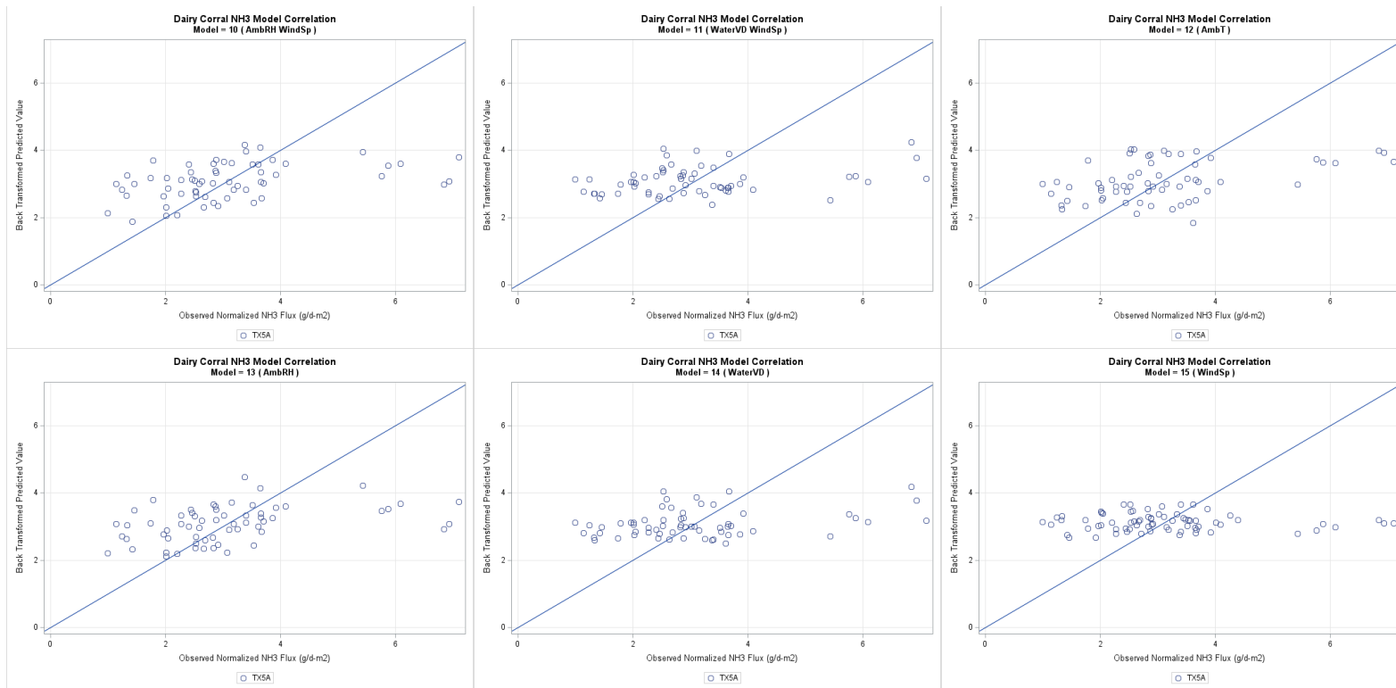
Figure G-80. Dairy corral NH 3 one-to-one plots models 10a through 15a, back transformed.
