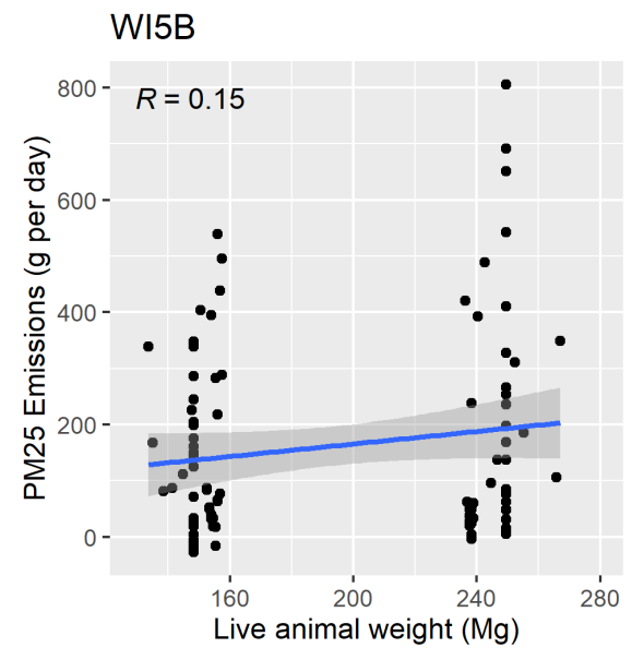
Figure F-14. Scatter plot of mechanically ventilated PM2.5 emissions versus live animal weight and scatter plot with regression.
