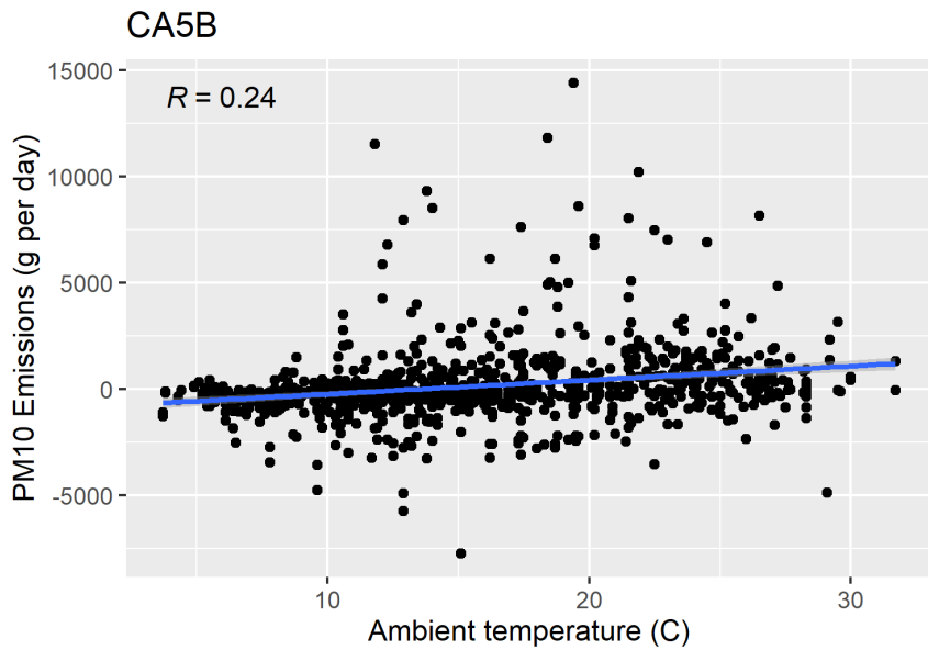
Figure F-113. Scatter plot of naturally ventilated barns PM 10 emissions versus ambient temperature and scatter plot with regression.
