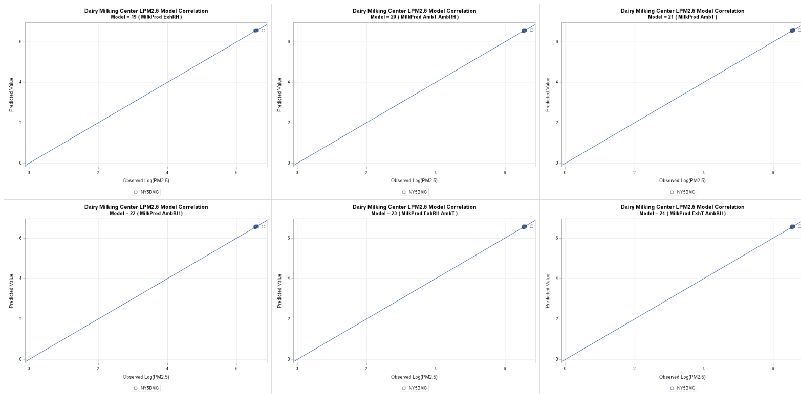
Figure G-43. Dairy milking center PM 2.5 one-to-one plots models 19 through 24, log transformed.
