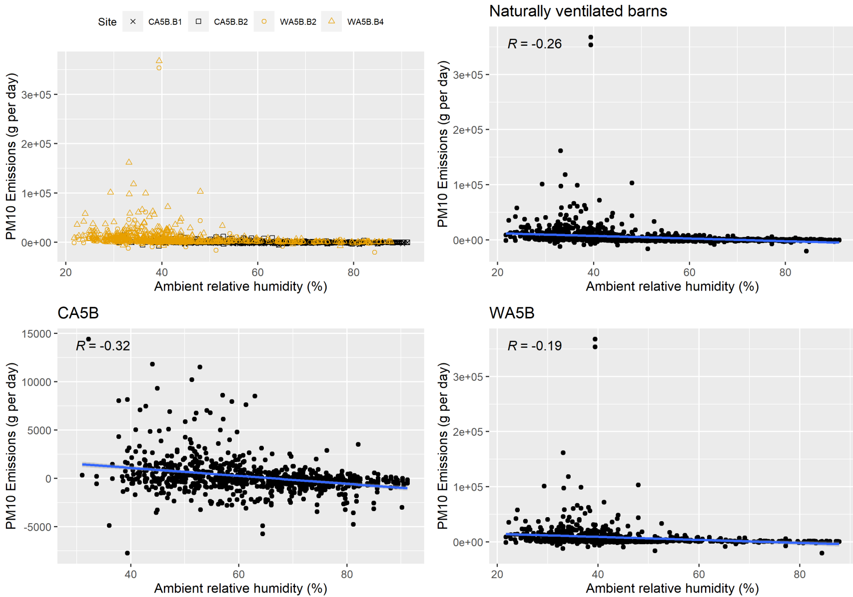
Figure F-118. Scatter plot of naturally ventilated barns PM 10 emissions versus ambient relative humidity and scatter plot with regression.
