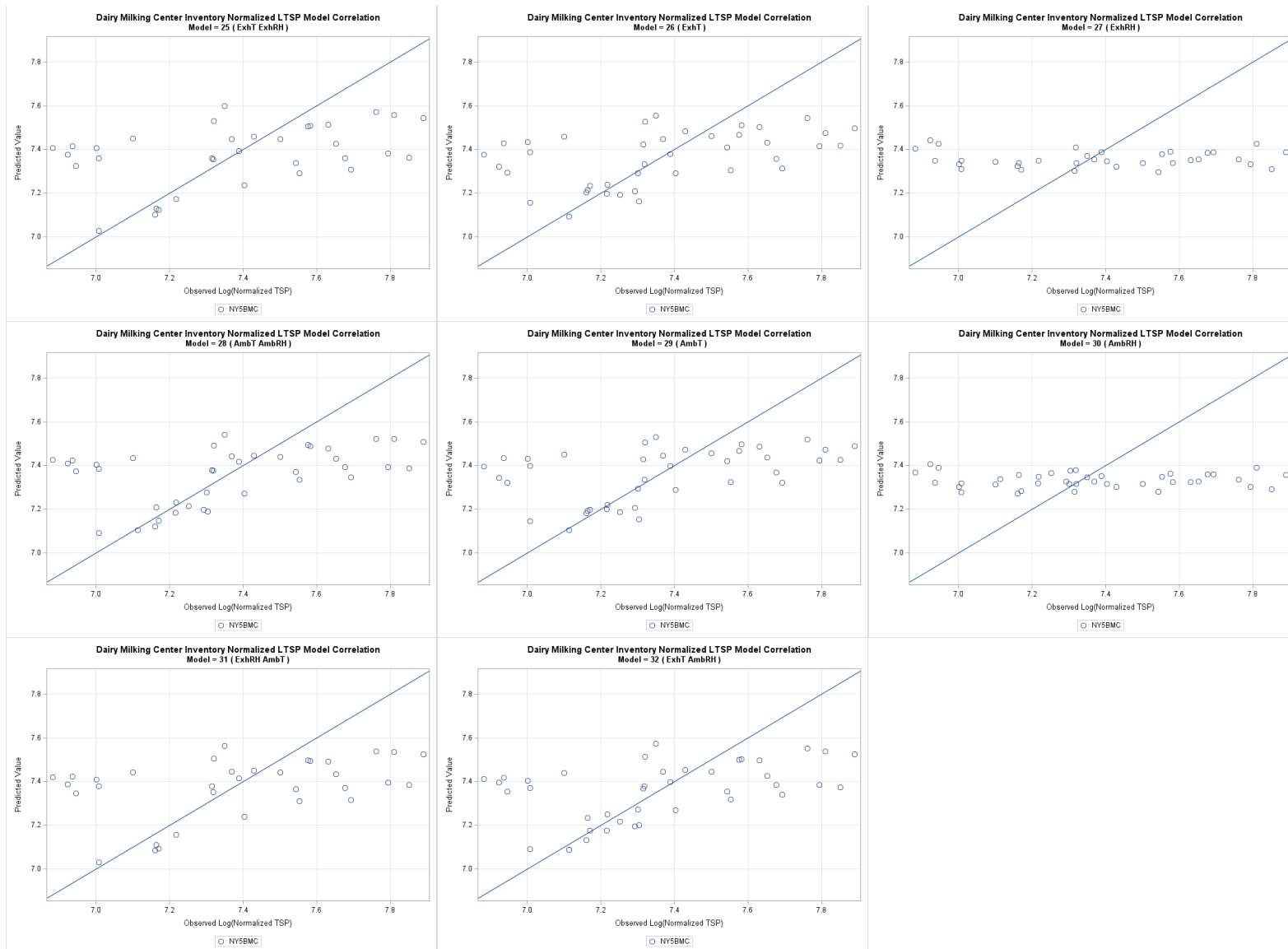
Figure G-52. Dairy milking center TSP one-to-one plots models 25 through 32, log transformed.
