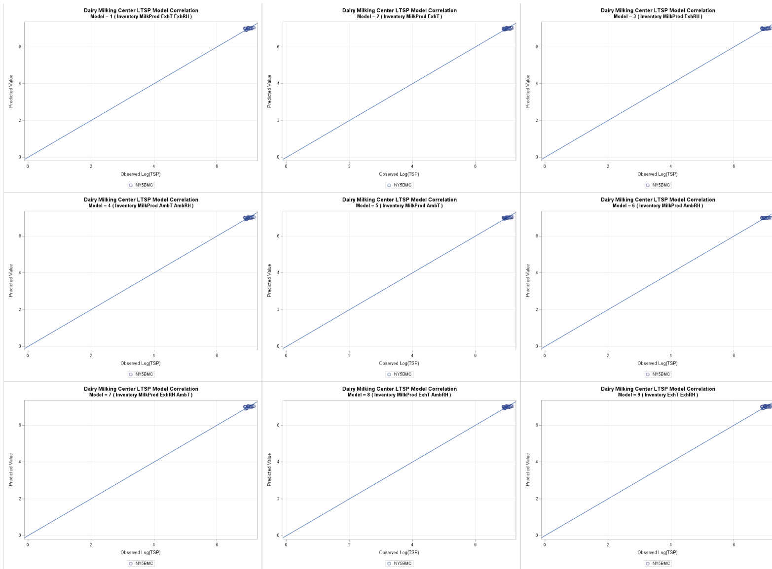
Figure G-49. Dairy milking center TSP one-to-one plots models 1 through 9, log transformed.
