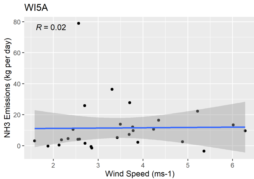
Figure F-134. Scatter plot of lagoon/basin NH 3 emissions versus wind speed and scatter plot with regression.
