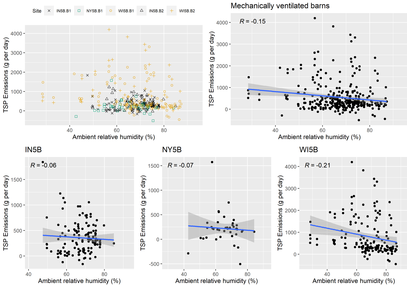
Figure F-40. Scatter plot of mechanically ventilated TSP emissions versus ambient relative humidity and scatter plot with regression.
