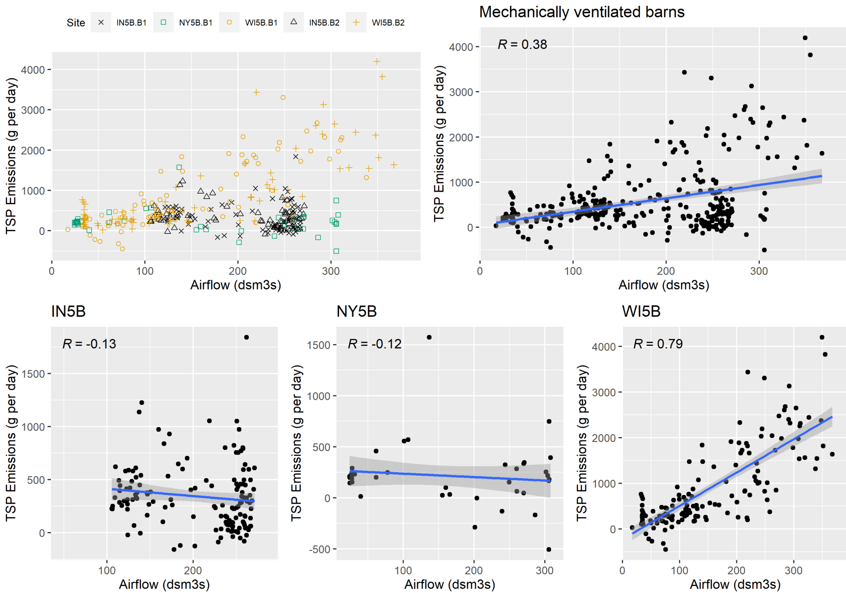
Figure F-30. Scatter plot of mechanically ventilated TSP emissions versus airflow and scatter plot with regression.
