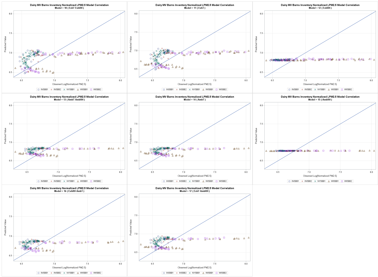
Figure G-10. Dairy mechanically ventilated barn PM 2.5 one-to-one plots models 10 through 17, log transformed.
