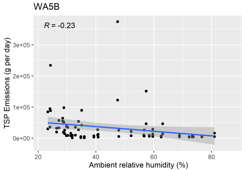
Figure F-120. Scatter plot of naturally ventilated barns TSP emissions versus ambient relative humidity and scatter plot with regression.
