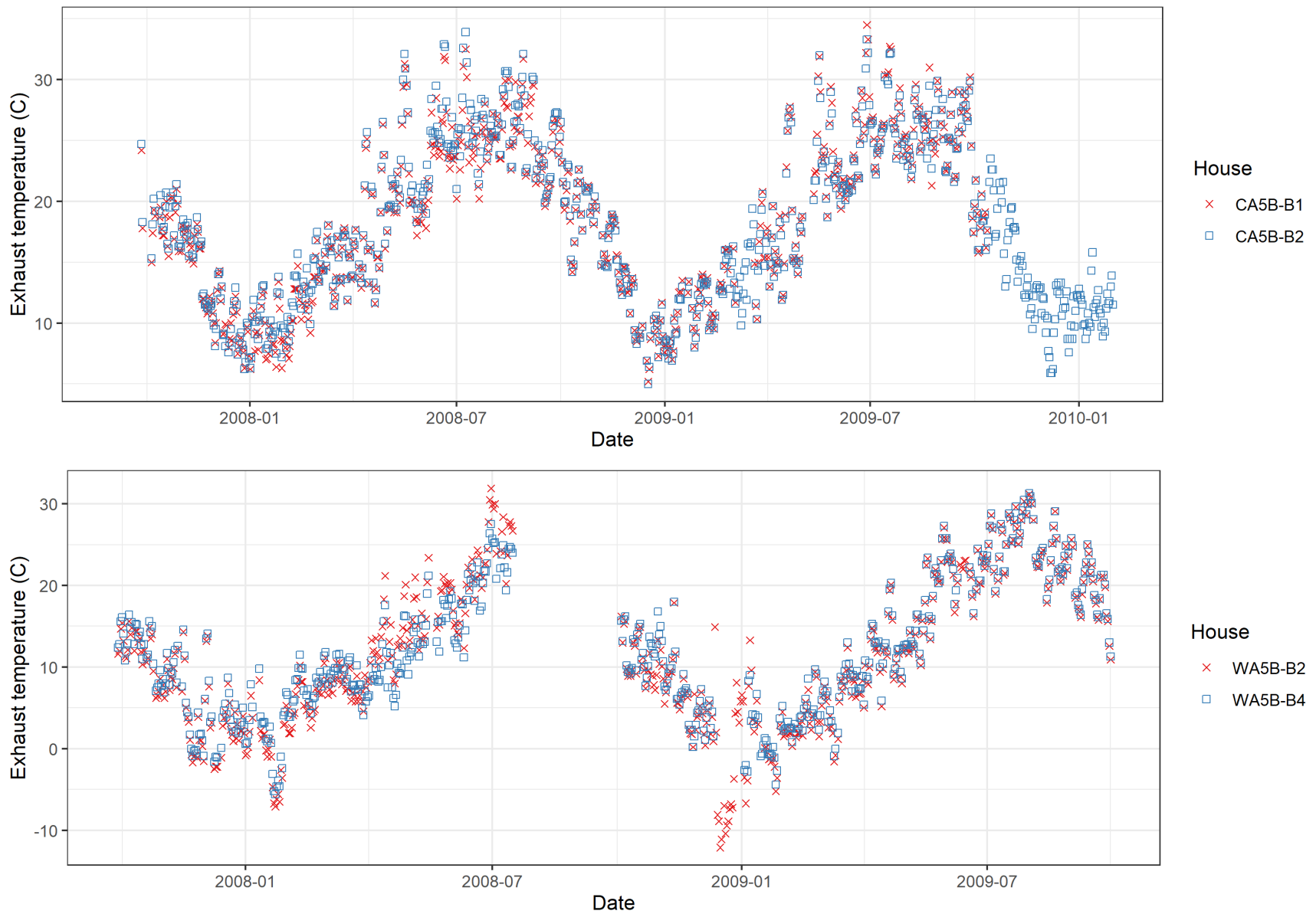
Figure E-37. Trends in exhaust temperature at naturally ventilated barns, by site, during the NAEMS monitoring period.
