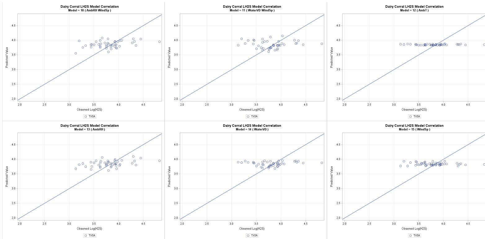
Figure G-84. Dairy corral H 2 S one-to-one plots models 10a through 15a, log transformed.
