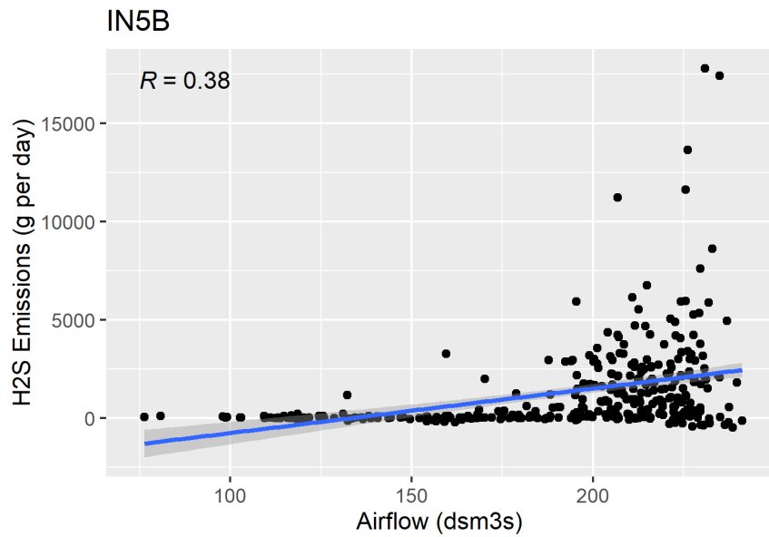
Figure F-67. Scatter plot of milking center H 2 S emissions versus airflow and scatter plot with regression.
