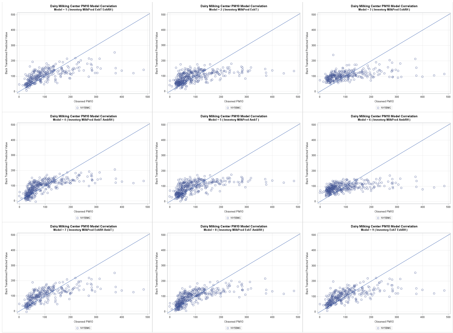
Figure G-37. Dairy milking center PM 10 one-to-one plots models 1 through 9, back transformed.
