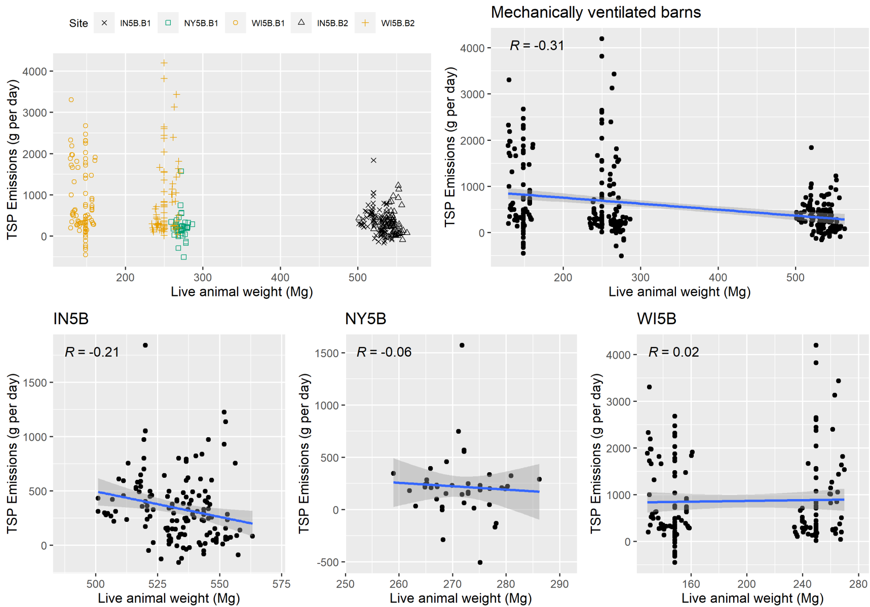
Figure F-15. Scatter plot of mechanically ventilated TSP emissions versus live animal weight and scatter plot with regression.
