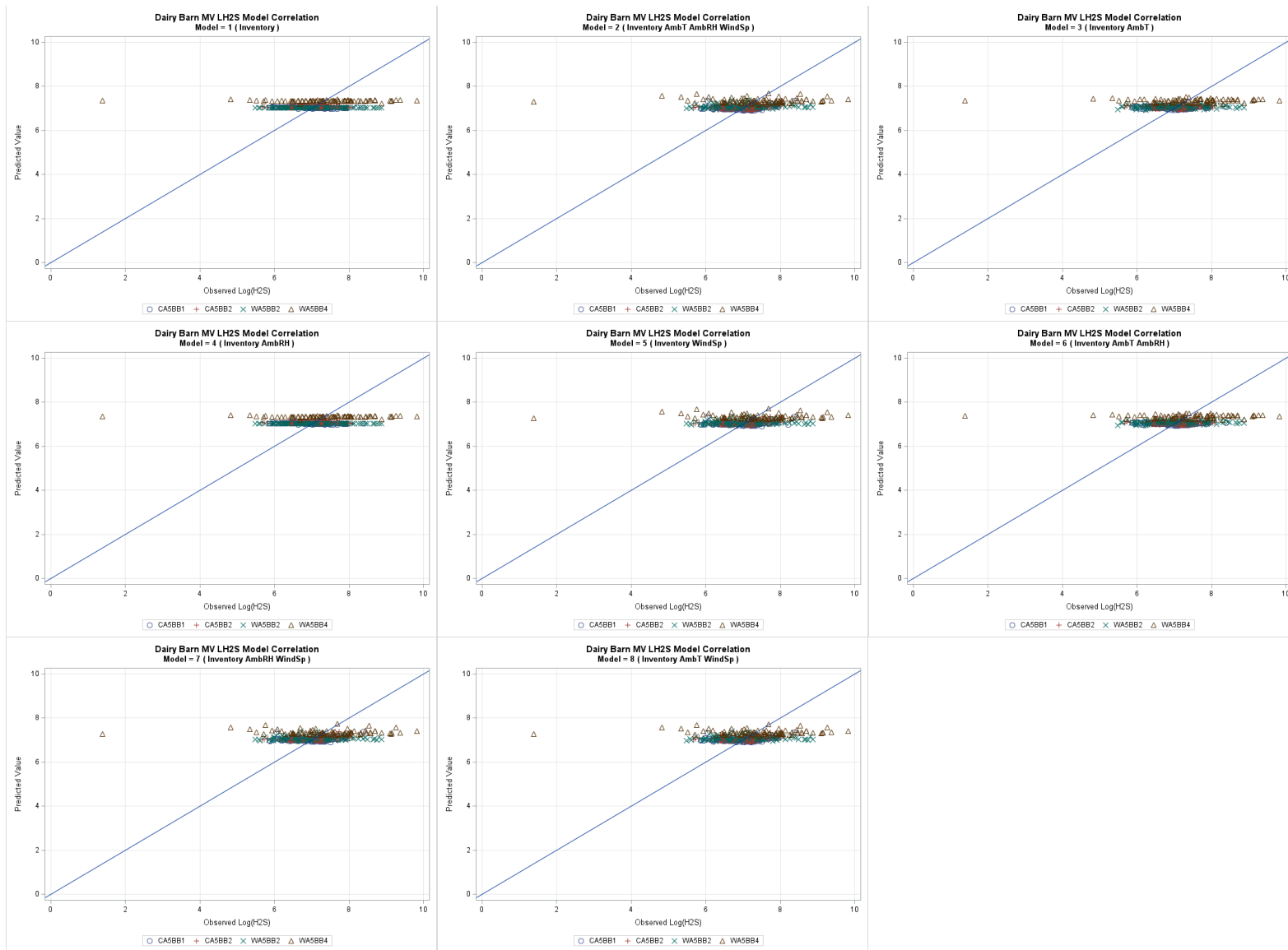
Figure G-59. Dairy naturally ventilated barn H 2 S one-to-one plots models 1 through 8, log transformed.
