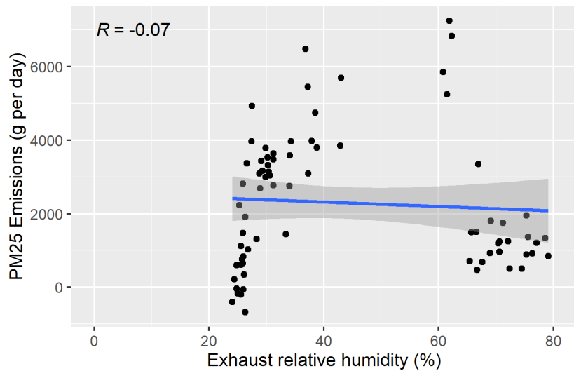
Figure F-104. Scatter plot of naturally ventilated barns PM 2.5 emissions versus exhaust relative humidity and scatter plot with regression.
