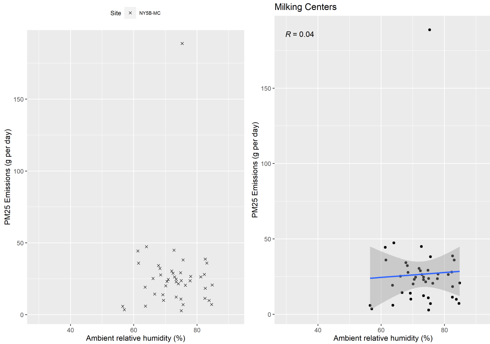
Figure F-79. Scatter plot of milking center PM 2.5 emissions versus ambient relative humidity and scatter plot with regression.
