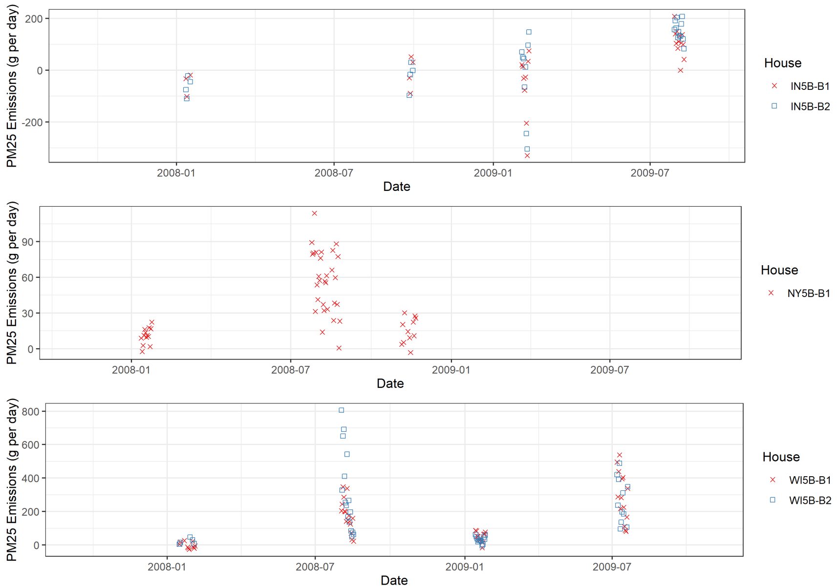
Figure E-4. Trends in PM 2.5 emissions at mechanically ventilated barns, by site, during the NAEMS monitoring period.
