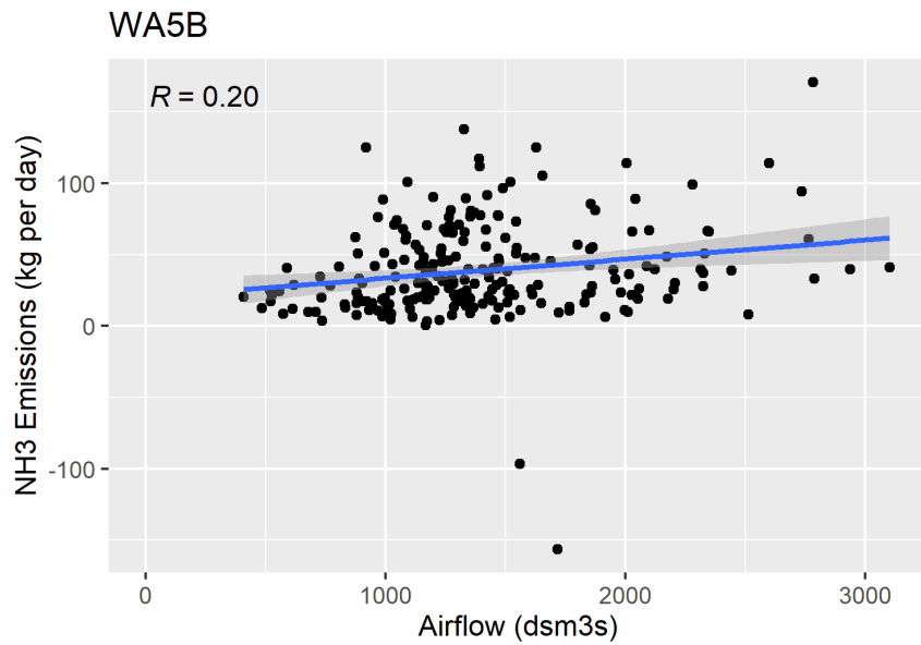
Figure F-106. Scatter plot of naturally ventilated barns NH 3 emissions versus airflow and scatter plot with regression.
