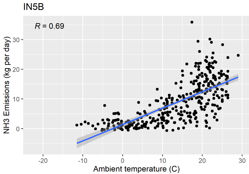
Figure F-71. Scatter plot of milking center NH 3 emissions versus ambient temperature and scatter plot with regression.
