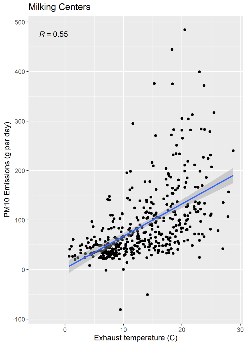
Figure F-58. Scatter plot of milking center PM 10 emissions versus exhaust temperature and scatter plot with regression.
