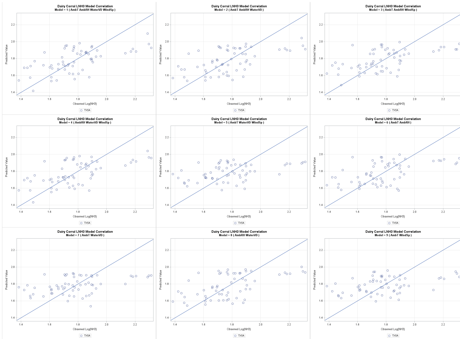
Figure G-75. Dairy corral NH 3 one-to-one plots models 1a through 9a, log transformed.
