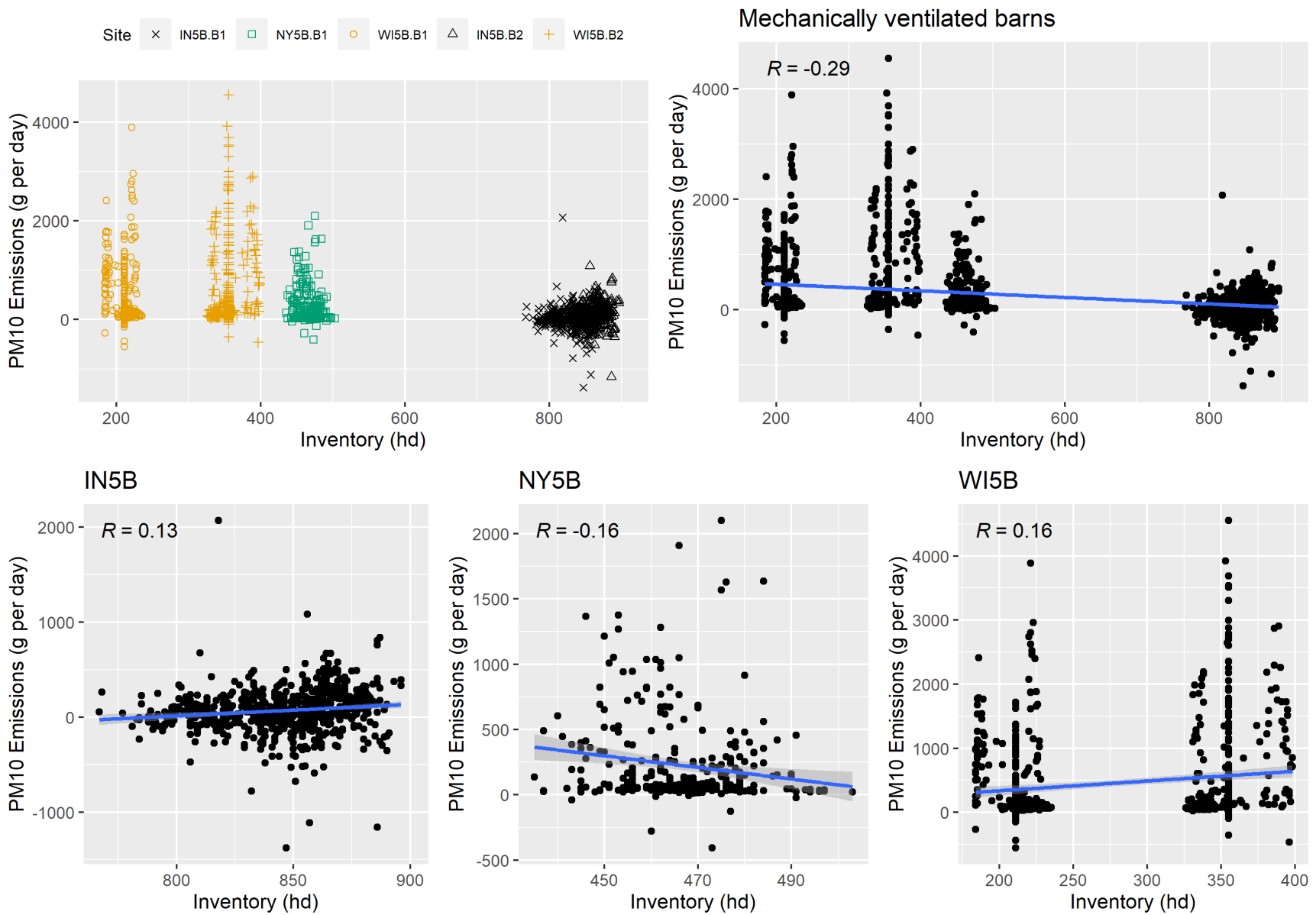
Figure F-3. Scatter plot of mechanically ventilated PM 10 emissions versus inventory and scatter plot with regression.
