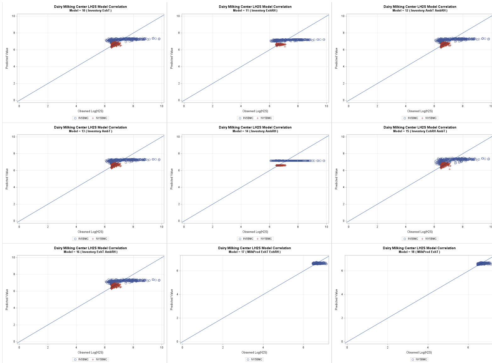
Figure G-26. Dairy milking center H 2 S one-to-one plots models 10 through 18, log transformed.
