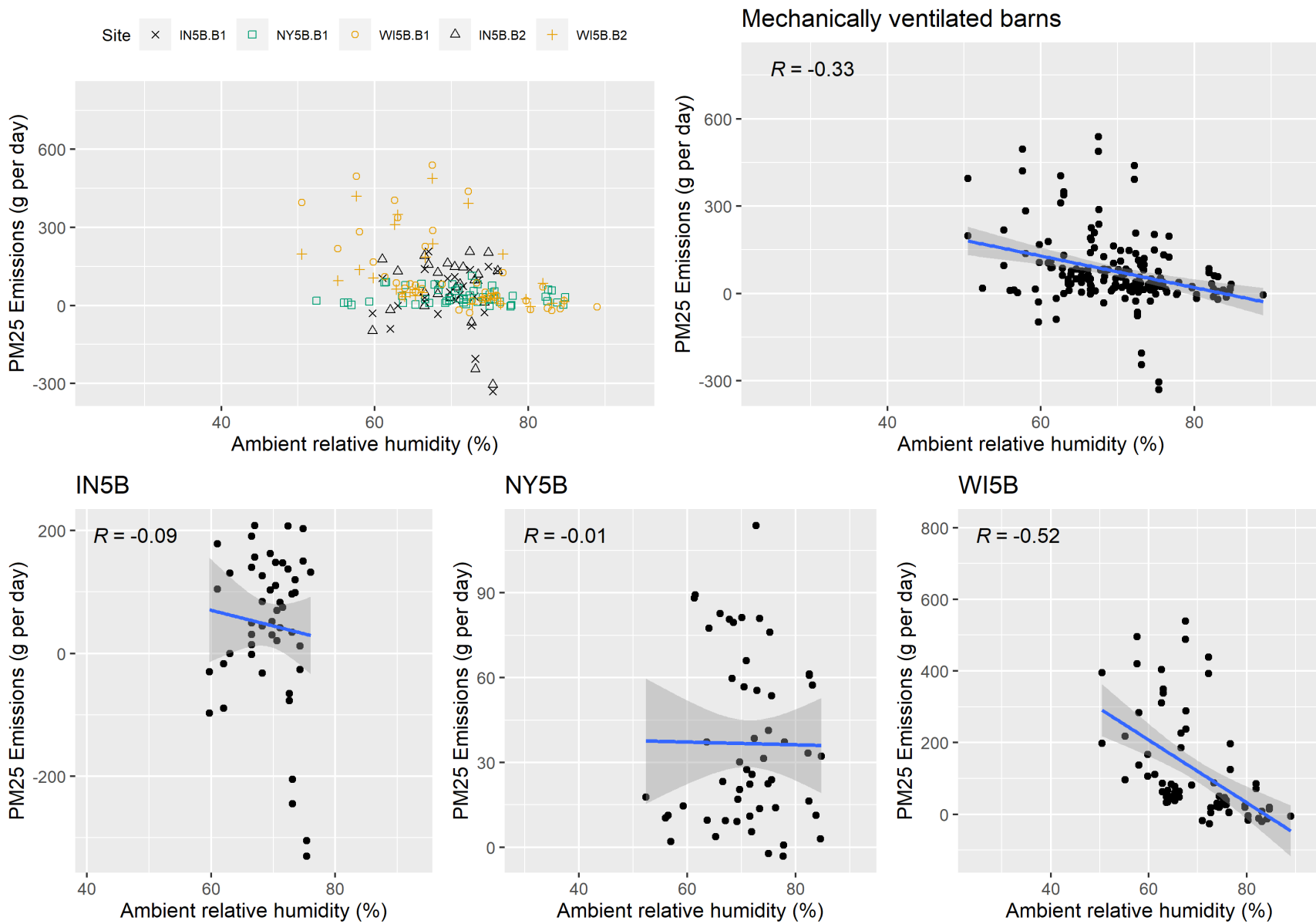
Figure F-39. Scatter plot of mechanically ventilated PM 2.5 emissions versus ambient relative humidity and scatter plot with regression.
