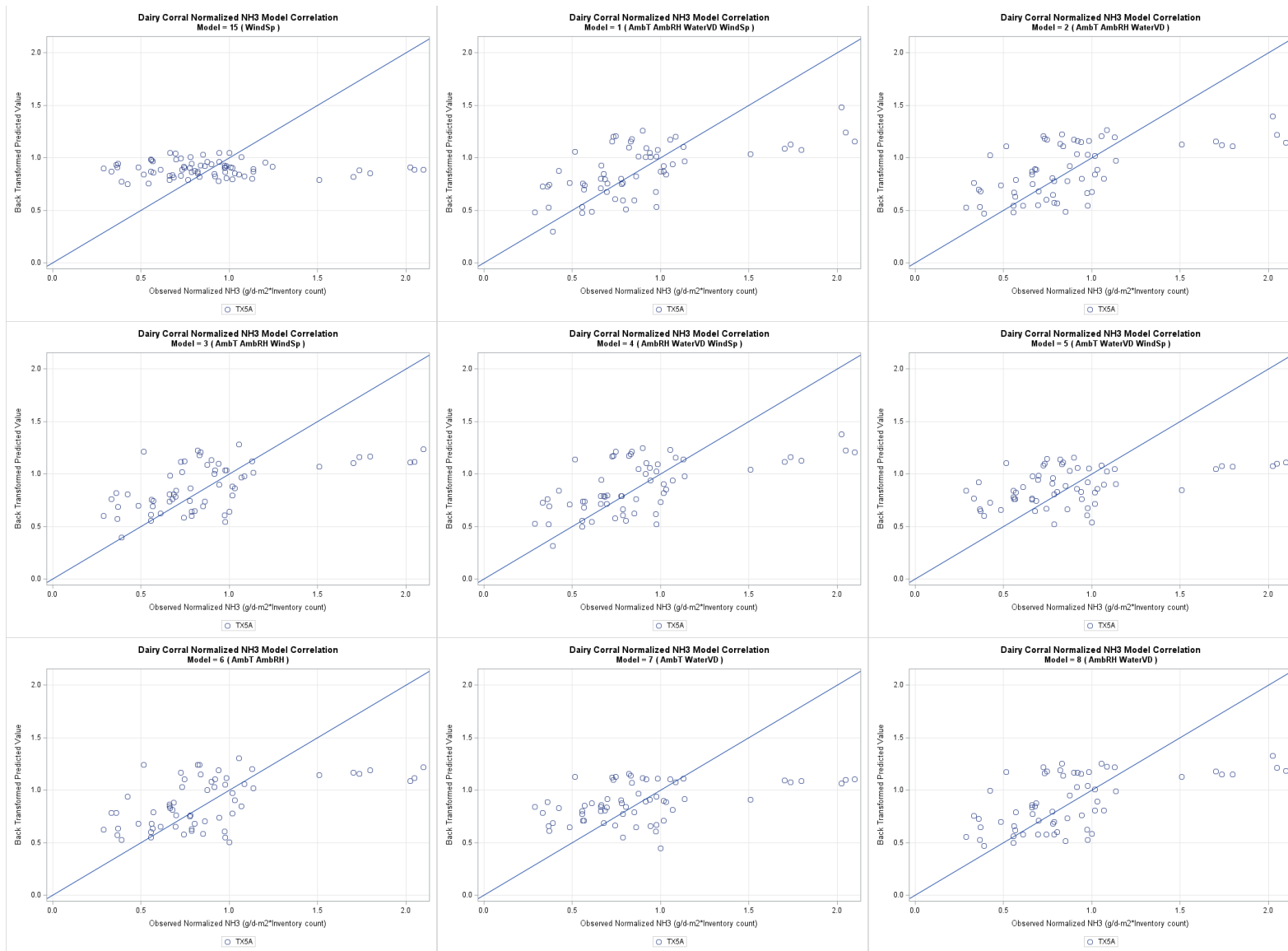
Figure G-81. Dairy corral NH 3 one-to-one plots models 1b through 9b, back transformed.
