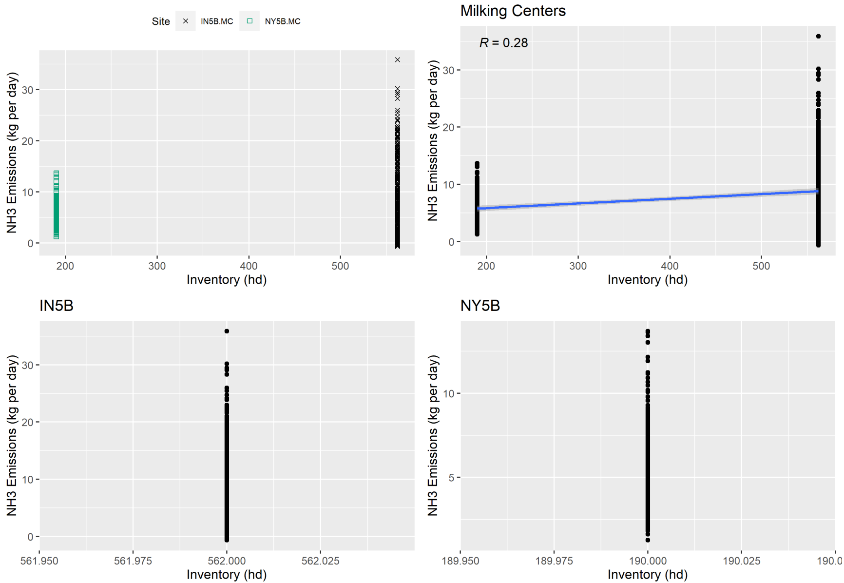
Figure F-41. Scatter plot of milking center NH 3 emissions versus inventory and scatter plot with regression.
