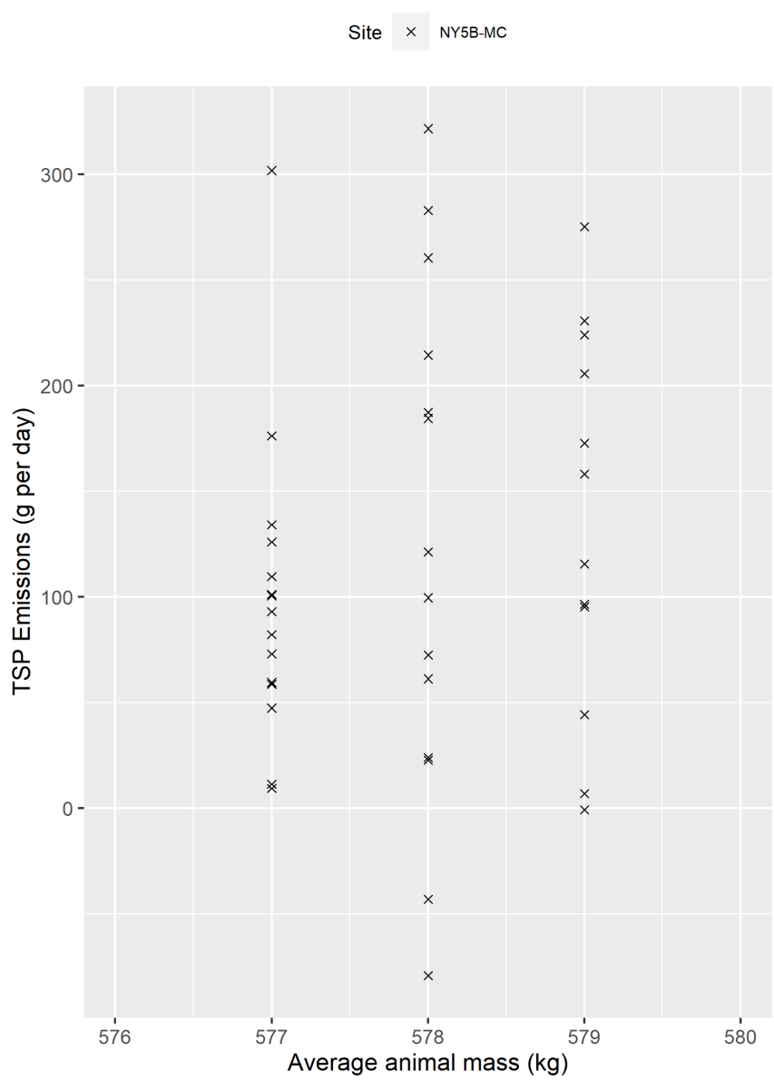
Figure F-50. Scatter plot of milking center TSP emissions versus average animal mass and scatter plot with regression.
