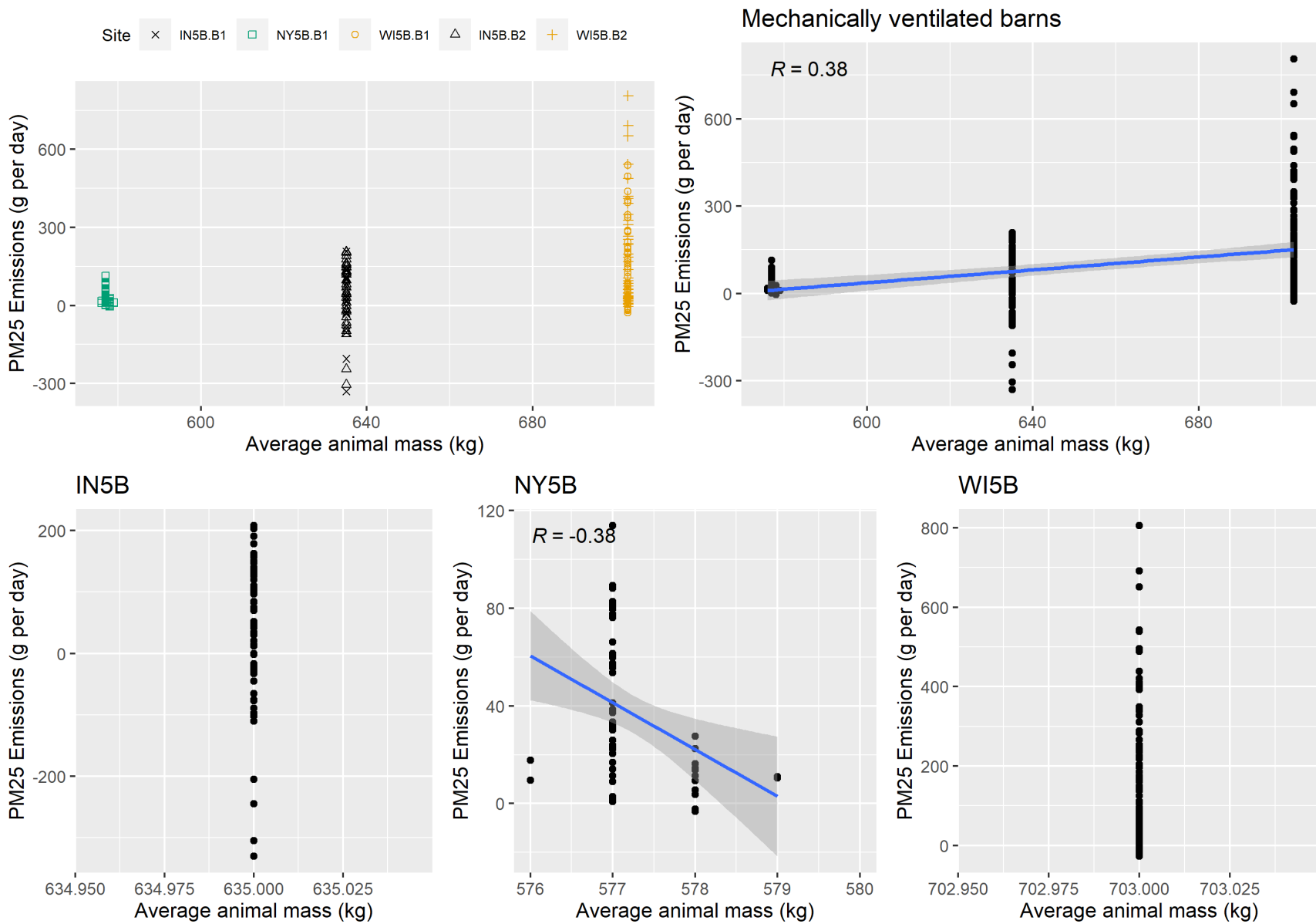
Figure F-9. Scatter plot of mechanically ventilated PM2.5 emissions versus average animal mass and scatter plot with regression.
