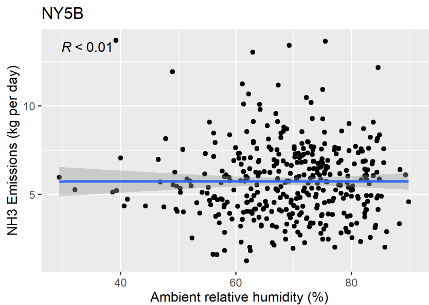
Figure F-76. Scatter plot of milking center NH 3 emissions versus ambient relative humidity and scatter plot with regression.
