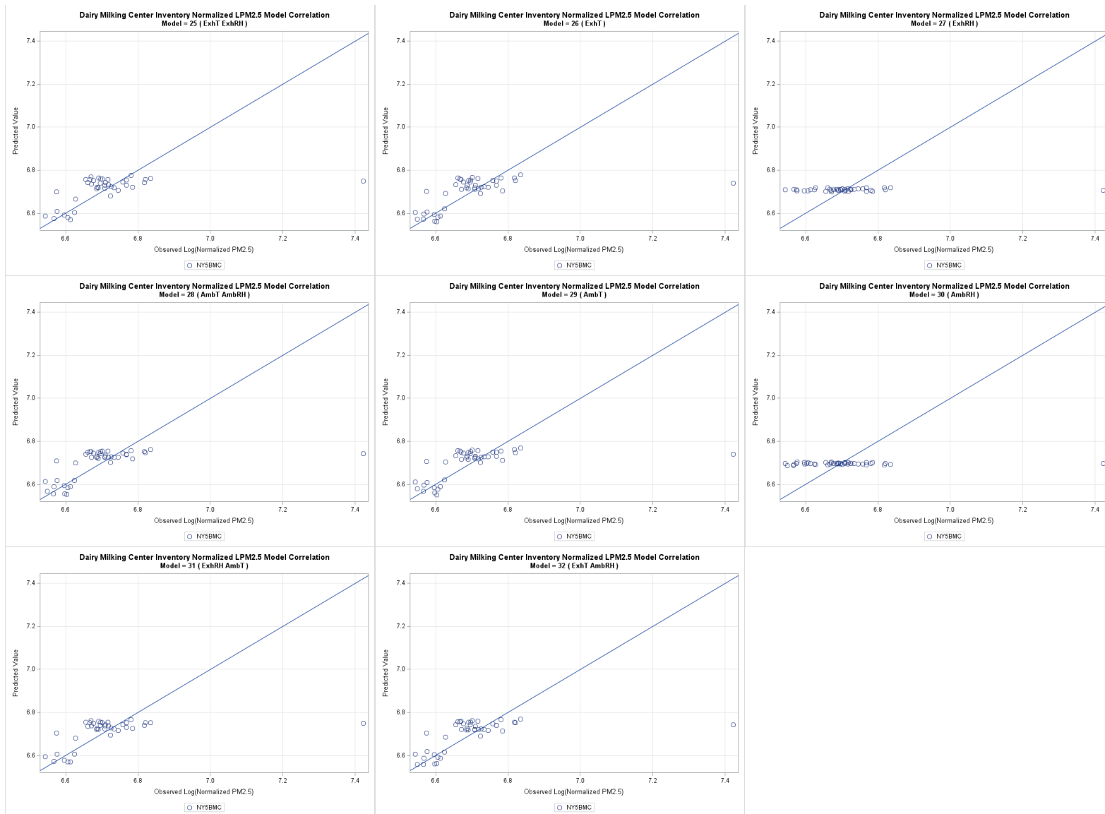
Figure G-44. Dairy milking center PM 2.5 one-to-one plots models 25 through 32, log transformed.
