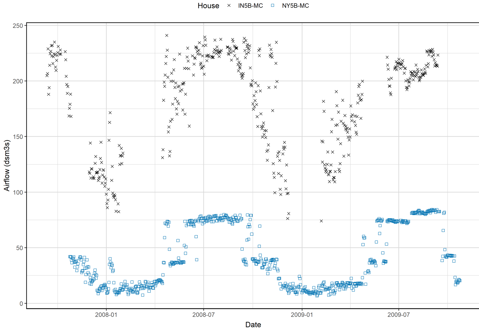
Figure E-24. Trends in ventilation rate at milking centers, by site, during the NAEMS monitoring period.
