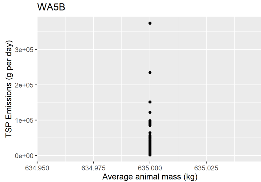
Figure F-90. Scatter plot of naturally ventilated barns TSP emissions versus average animal mass and scatter plot with regression.
