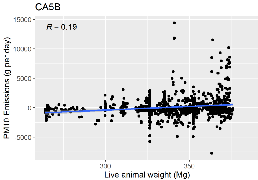
Figure F-93. Scatter plot of naturally ventilated barns PM 10 emissions versus live animal weight and scatter plot with regression.
