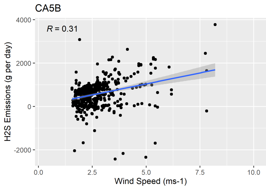
Figure F-122. Scatter plot of naturally ventilated barns H 2 S emissions versus wind speed and scatter plot with regression.
