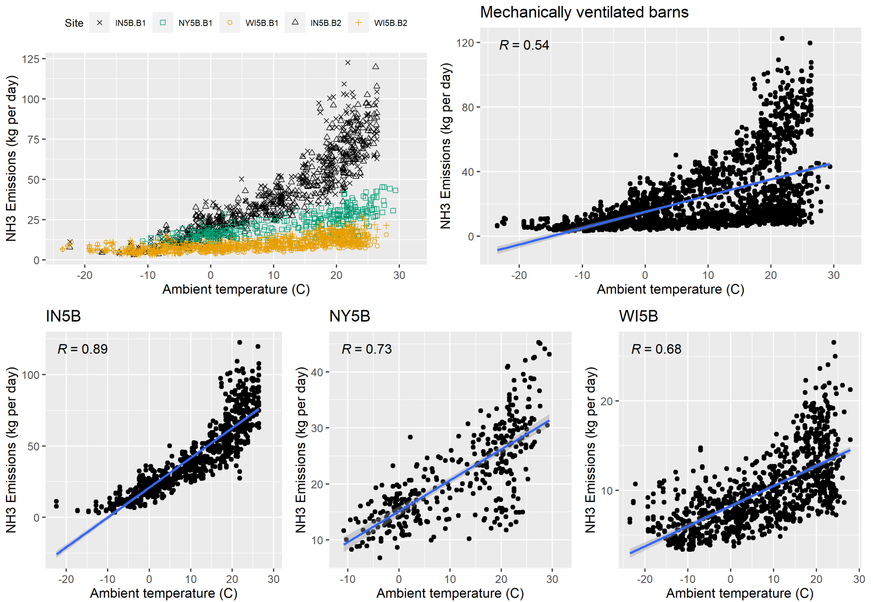
Figure F-31. Scatter plot of mechanically ventilated NH 3 emissions versus ambient temperature and scatter plot with regression.
