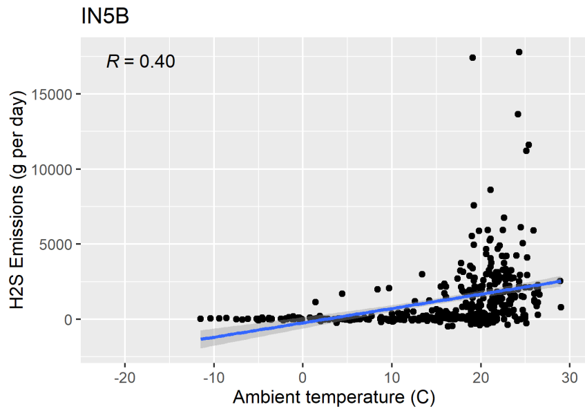
Figure F-72. Scatter plot of milking center H 2 S emissions versus ambient temperature and scatter plot with regression.
