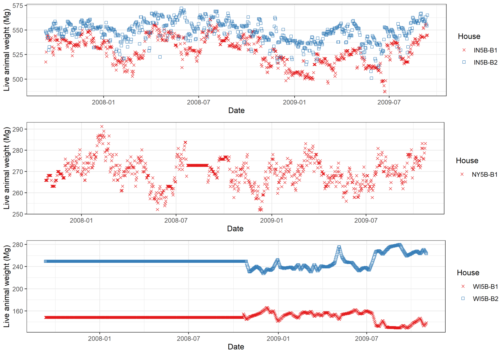
Figure E-8. Trends in live animal weight at mechanically ventilated barns, by site, during the NAEMS monitoring period.
