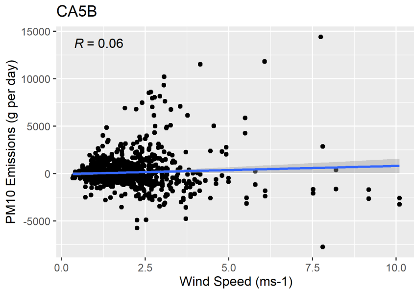
Figure F-123. Scatter plot of naturally ventilated barns PM 10 emissions versus wind speed and scatter plot with regression.
