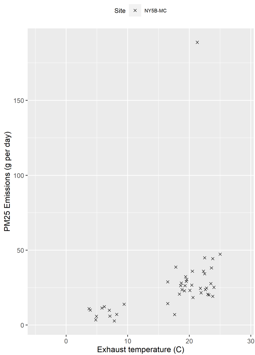
Figure F-59. Scatter plot of milking center PM 2.5 emissions versus exhaust temperature and scatter plot with regression.
