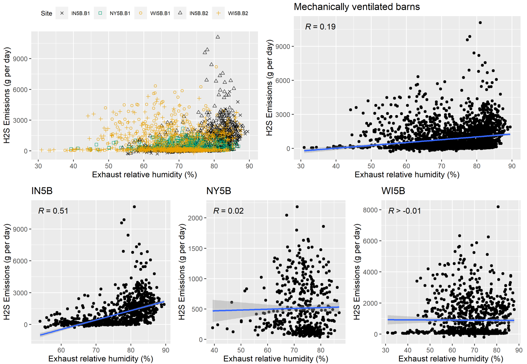
Figure F-22. Scatter plot of mechanically ventilated H 2 S emissions versus exhaust relative humidity and scatter plot with regression.
