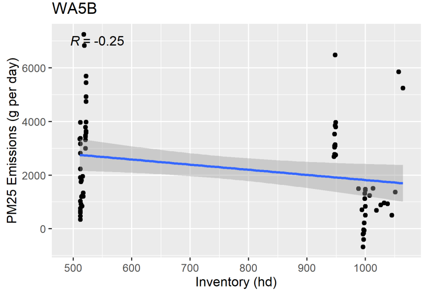
Figure F-84. Scatter plot of naturally ventilated barns PM 2.5 emissions versus inventory and scatter plot with regression.
