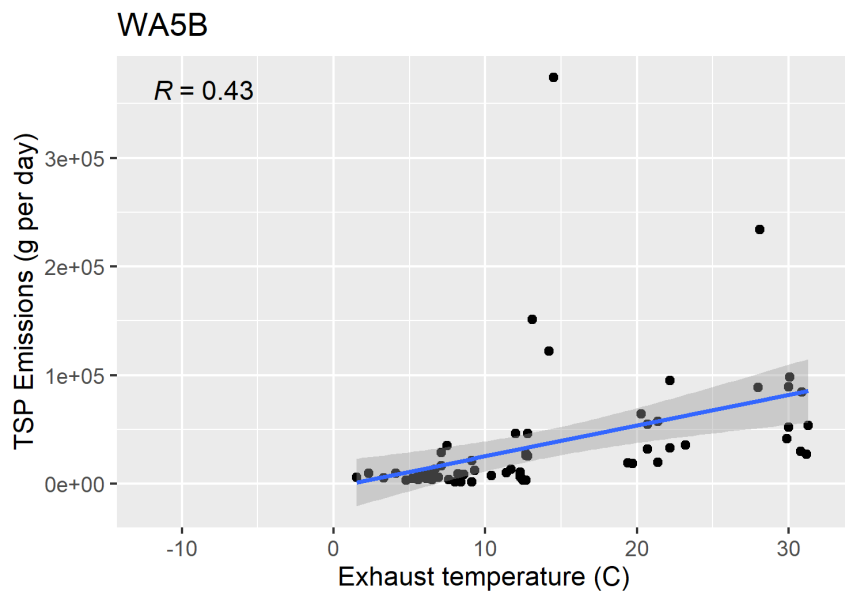
Figure F-100. Scatter plot of naturally ventilated barns TSP emissions versus exhaust temperature and scatter plot with regression.
