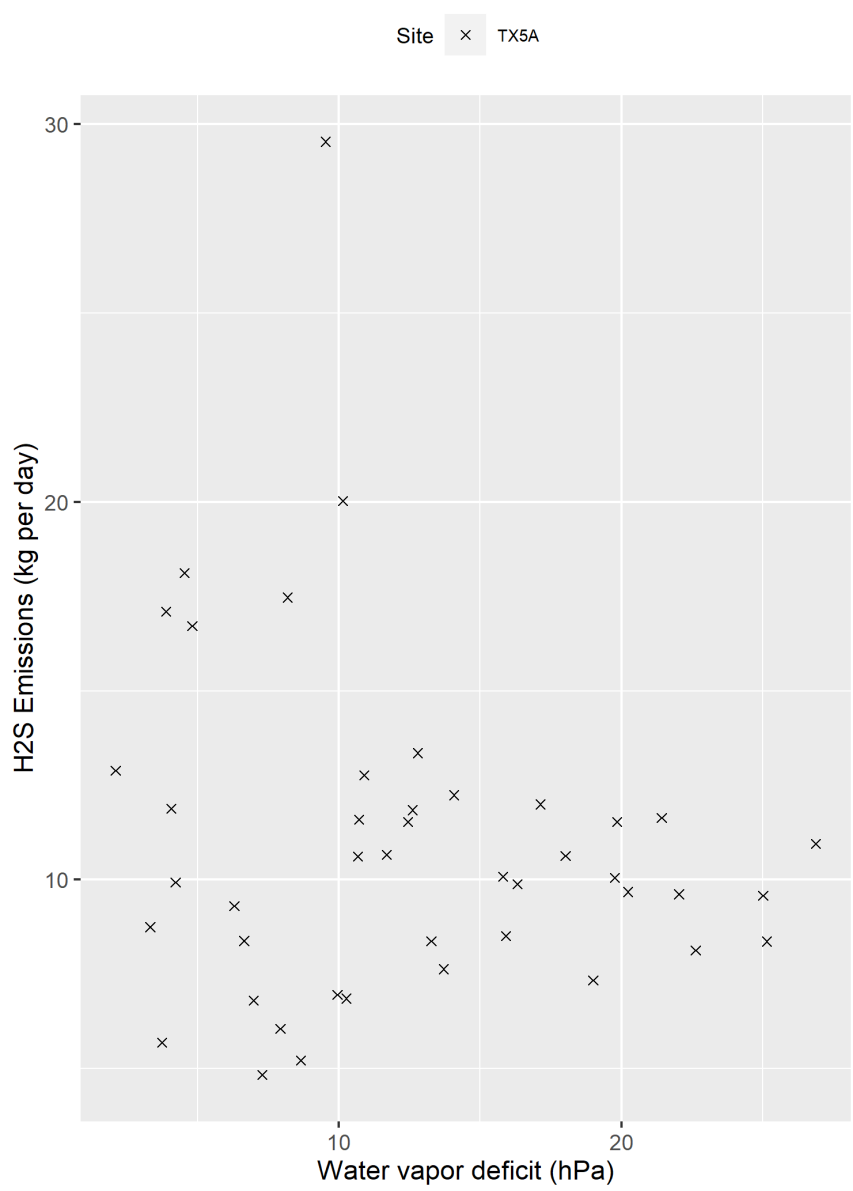
Figure F-143. Scatter plot of corral H 2 S emissions versus water vapor deficit and scatter plot with regression.
