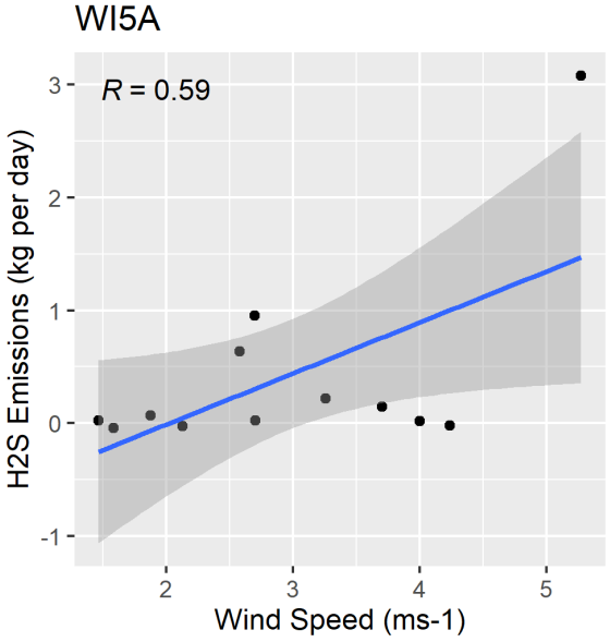
Figure F-135. Scatter plot of lagoon/basin H 2 S emissions versus wind speed and scatter plot with regression.
