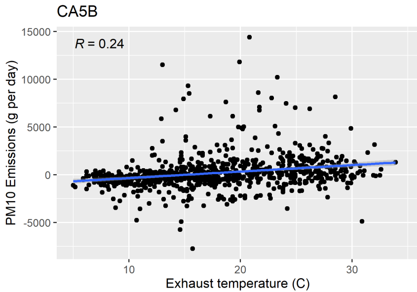
Figure F-98. Scatter plot of naturally ventilated barns PM 10 emissions versus exhaust temperature and scatter plot with regression.
