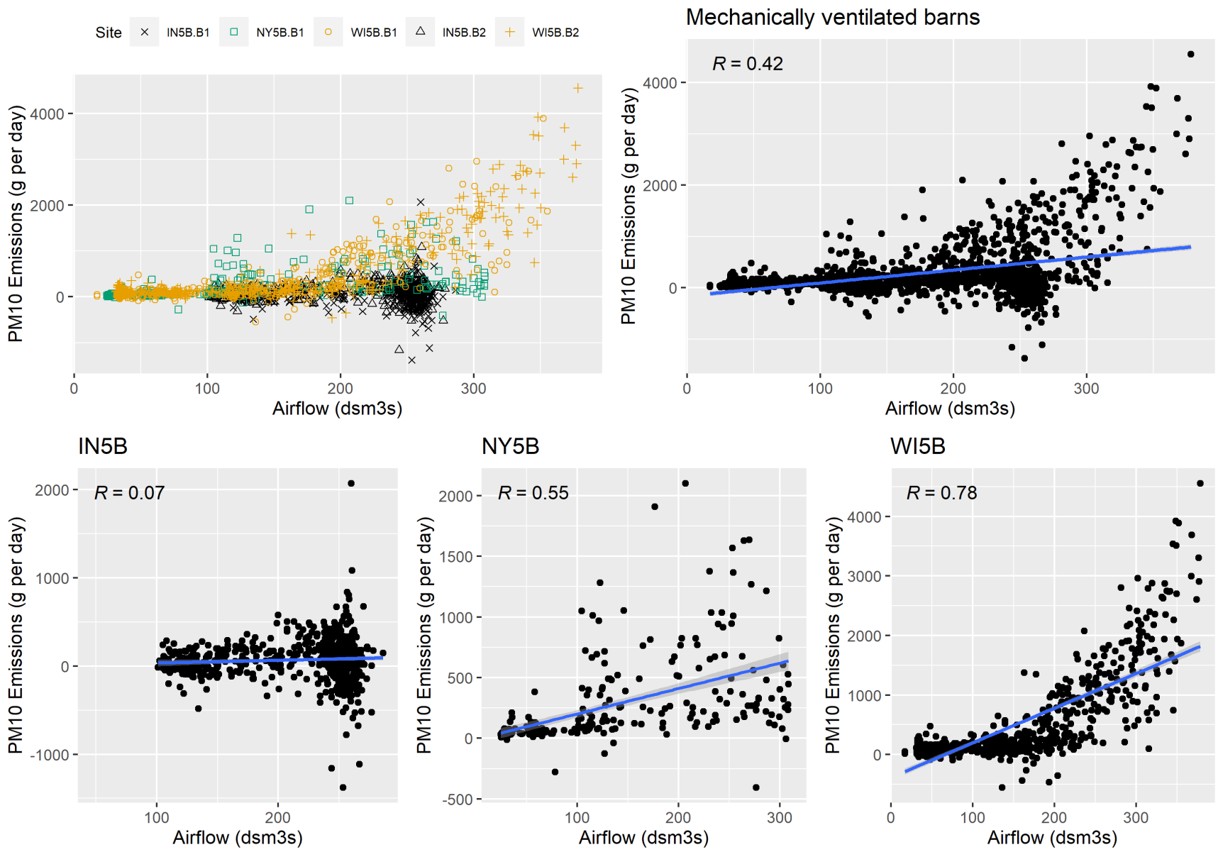
Figure F-28. Scatter plot of mechanically ventilated PM 10 emissions versus airflow and scatter plot with regression.
