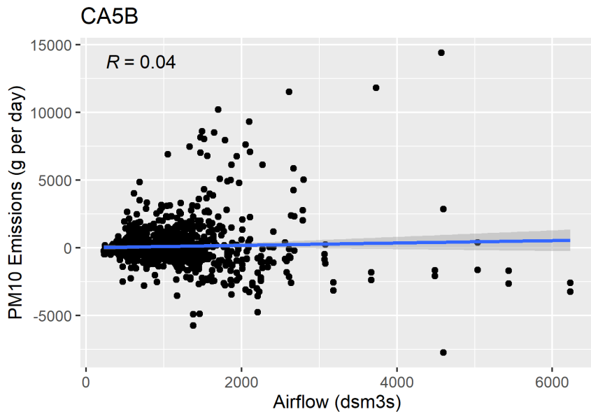
Figure F-108. Scatter plot of naturally ventilated barns PM 10 emissions versus airflow and scatter plot with regression.
