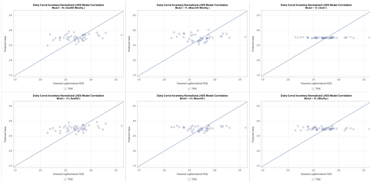
Figure G-86. Dairy corral H 2 S one-to-one plots models 10b through 15b, log transformed.
