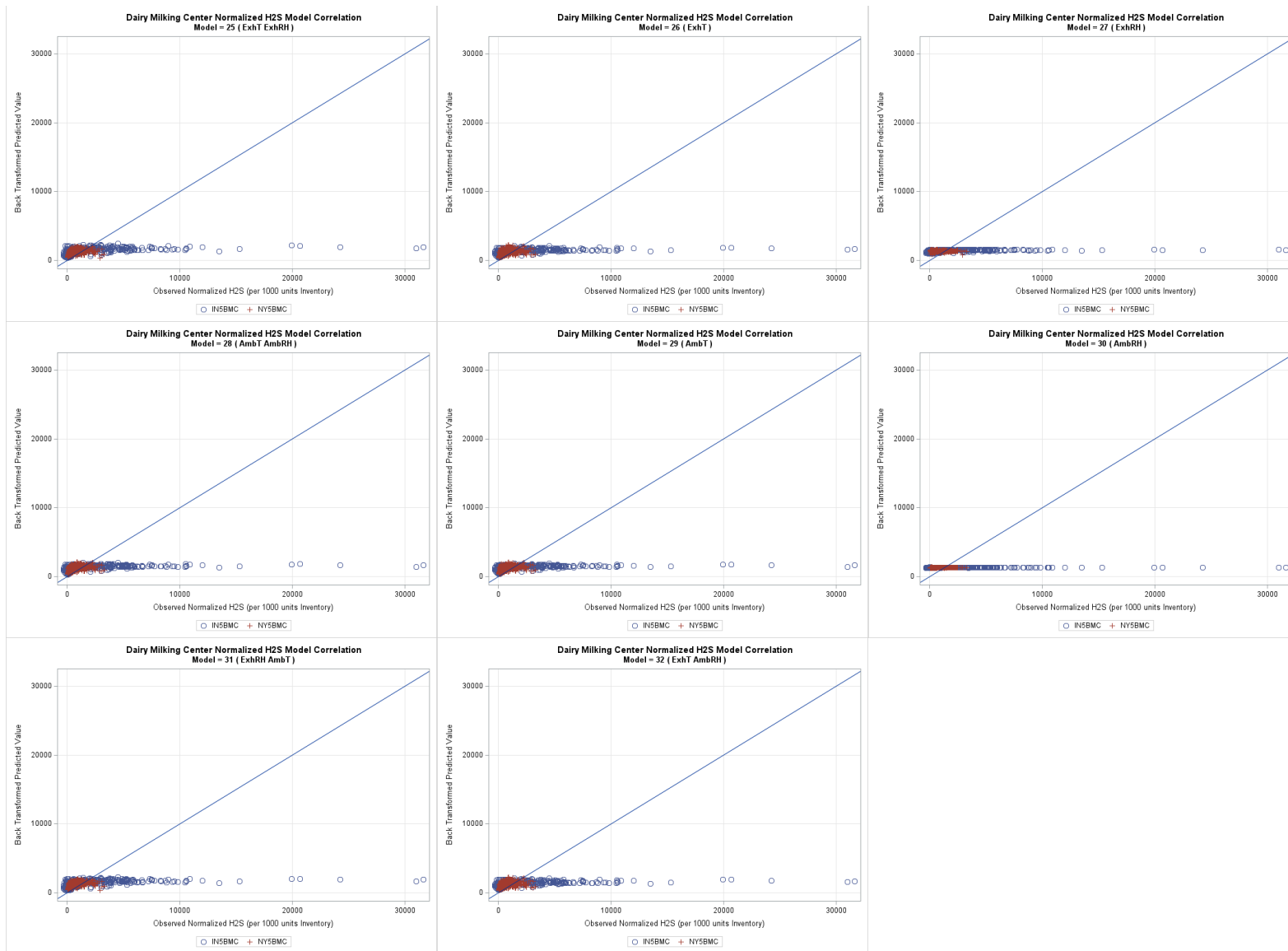
Figure G-32. Dairy milking center H 2 S one-to-one plots models 25 through 32, back transformed.
