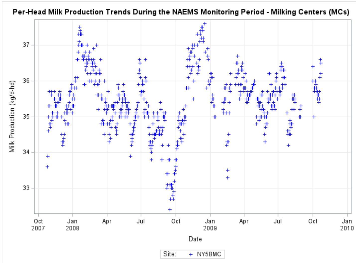
Figure E-26. Trends in milk production (kg per day per head) at milking centers, by site, during the NAEMS monitoring period.
