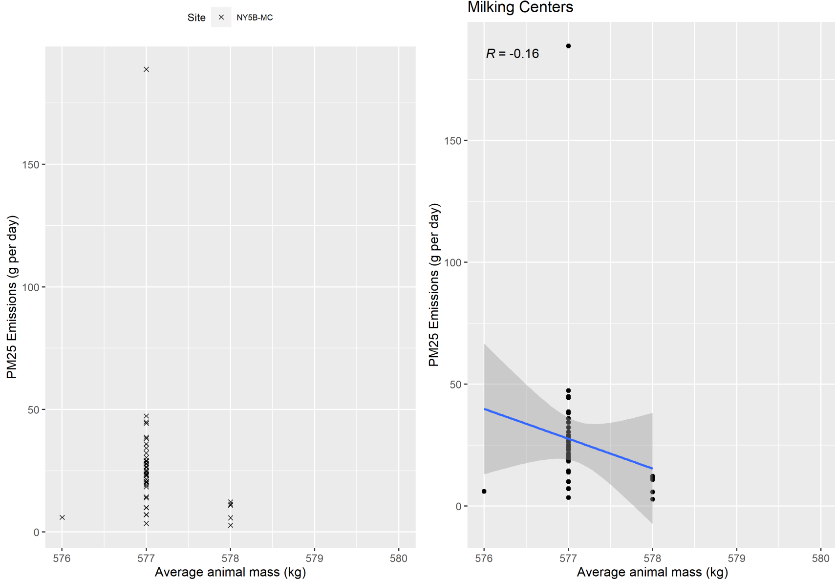
Figure F-49. Scatter plot of milking center PM 2.5 emissions versus average animal mass and scatter plot with regression.
