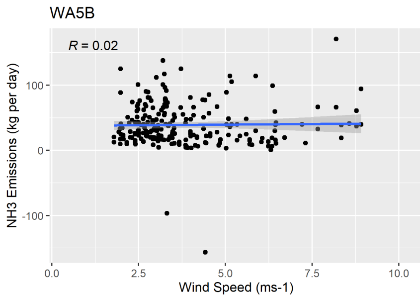
Figure F-121. Scatter plot of naturally ventilated barns NH 3 emissions versus wind speed and scatter plot with regression.
