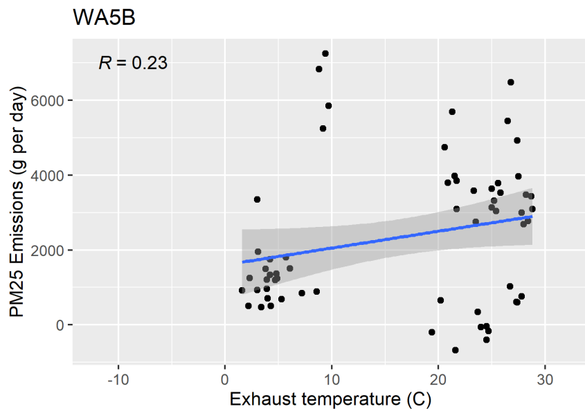
Figure F-99. Scatter plot of naturally ventilated barns PM 2.5 emissions versus exhaust temperature and scatter plot with regression.
