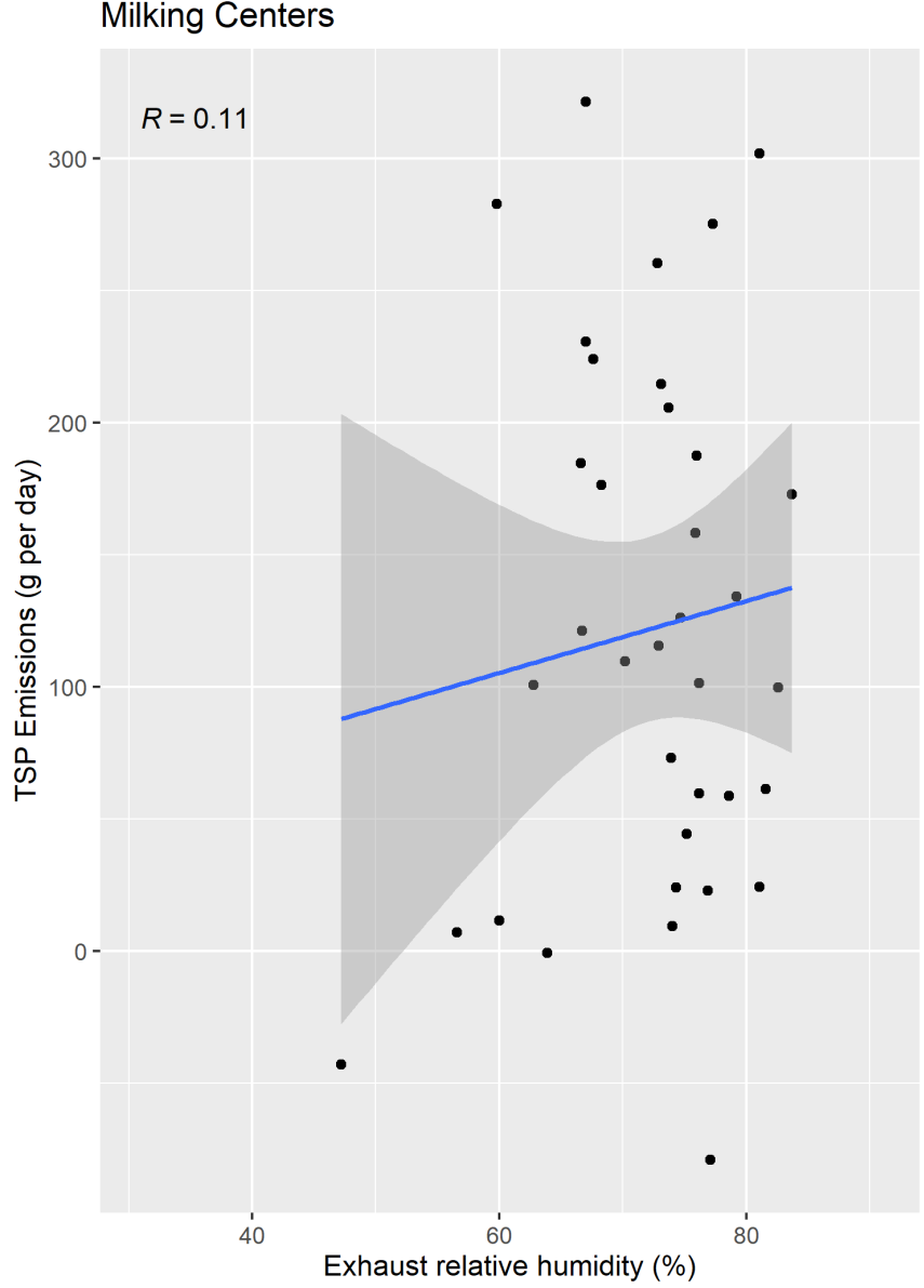
Figure F-65. Scatter plot of milking center TSP emissions versus exhaust relative humidity and scatter plot with regression.
