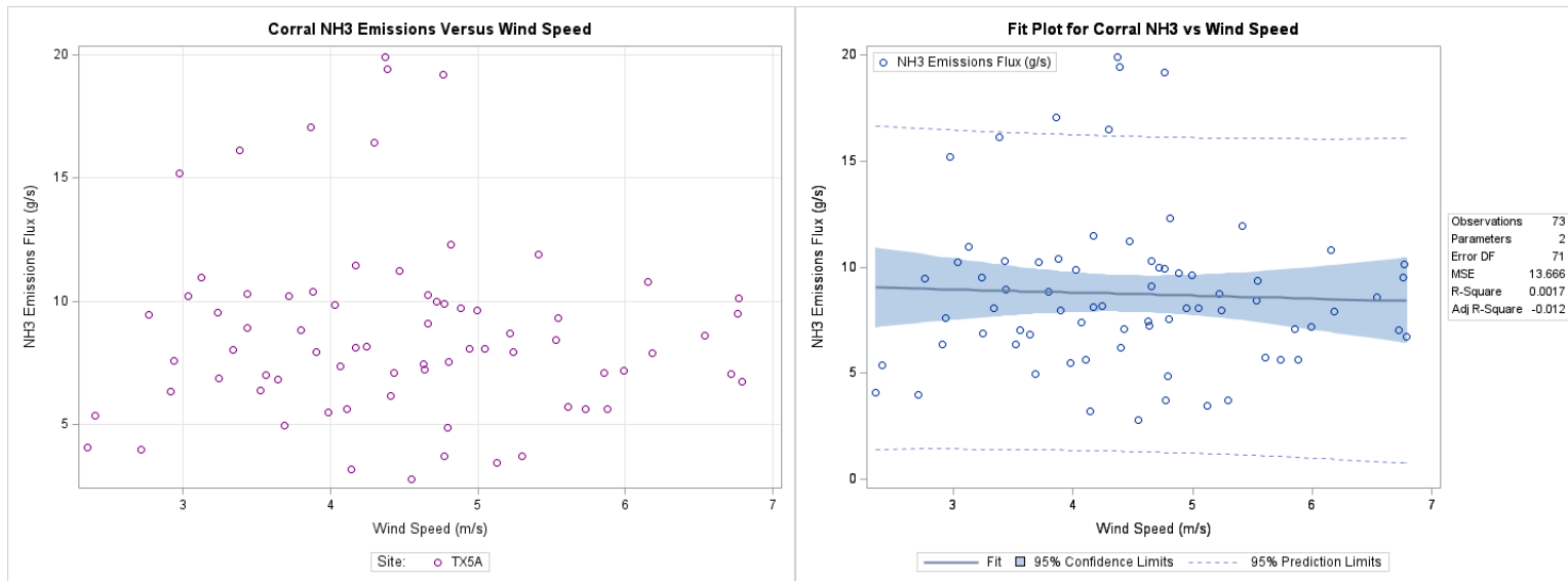
Figure F-140. Scatter plot of corral NH 3 emissions versus wind speed and scatter plot with regression.
