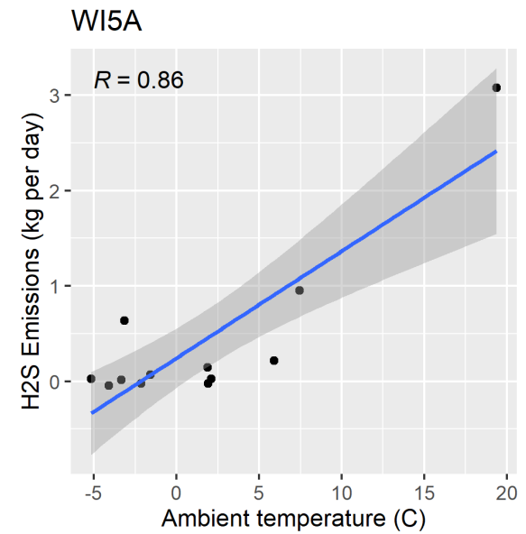
Figure F-131. Scatter plot of lagoon/basin H 2 S emissions versus ambient temperature and scatter plot with regression.
