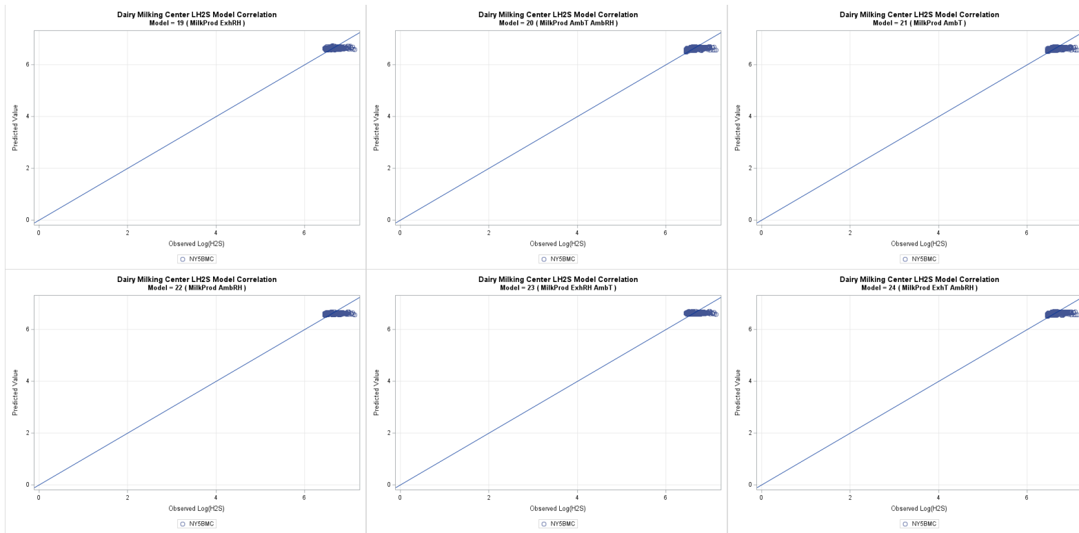
Figure G-27. Dairy milking center H 2 S one-to-one plots models 19 through 24, log transformed.
