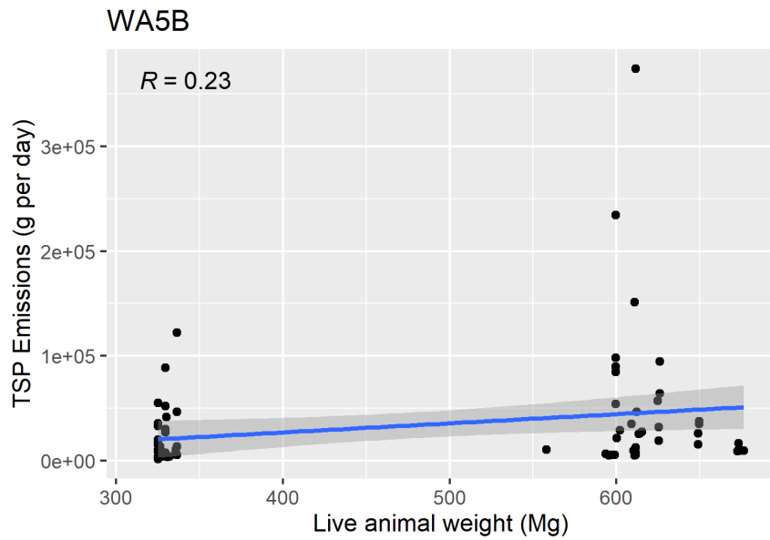
Figure F-95. Scatter plot of naturally ventilated barns TSP emissions versus live animal weight and scatter plot with regression.
