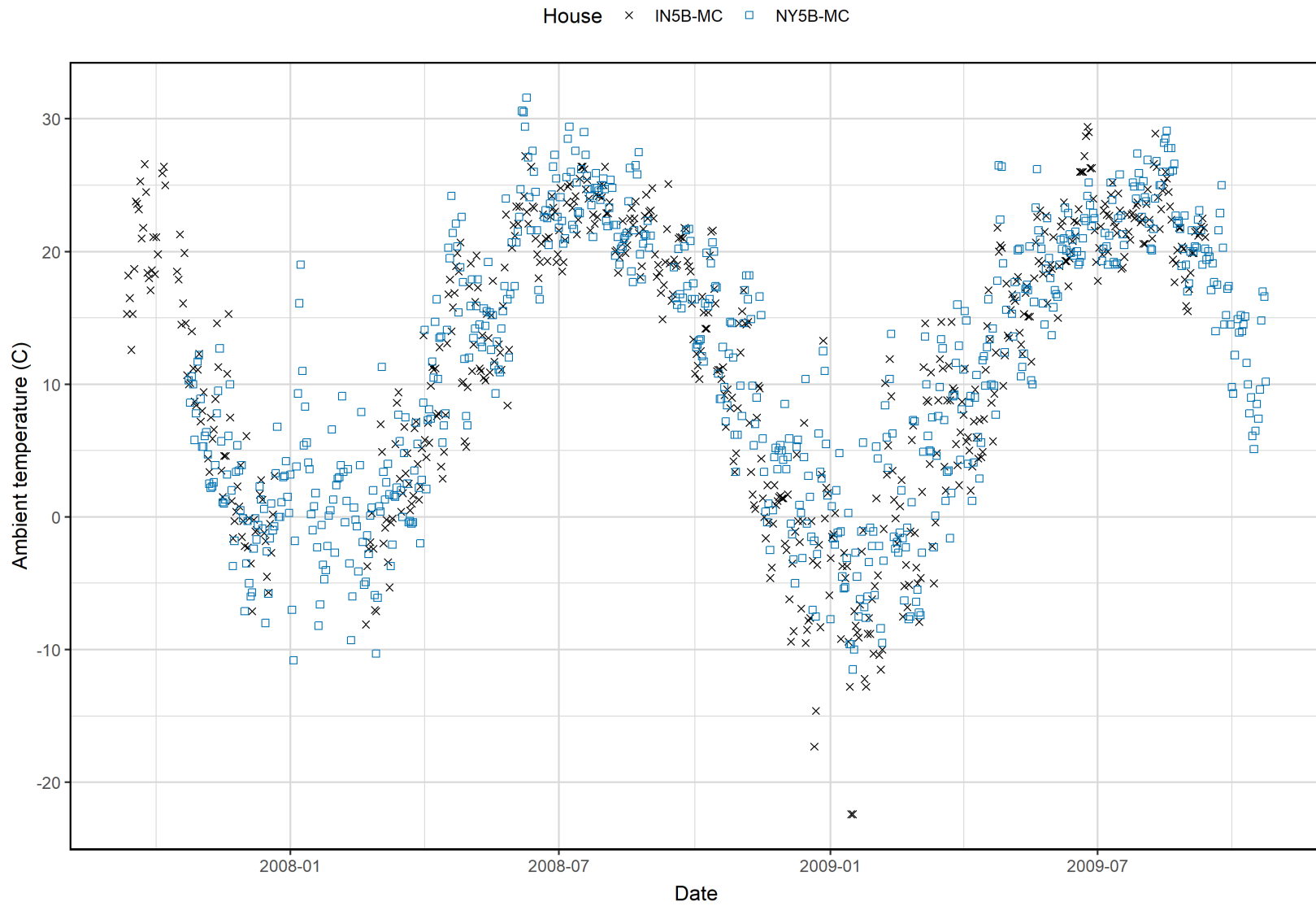
Figure E-27. Trends in ambient temperature at milking centers, by site, during the NAEMS monitoring period.
