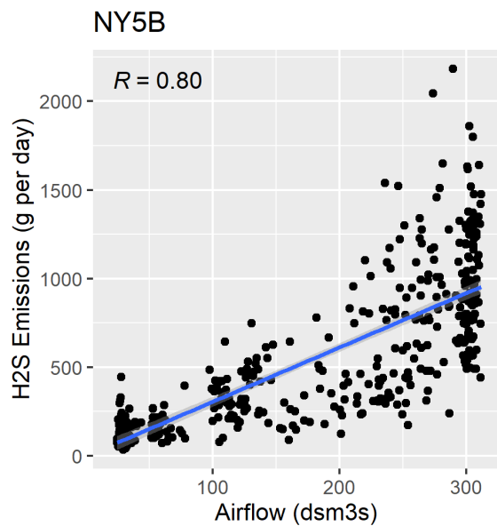
Figure F-27. Scatter plot of mechanically ventilated H 2 S emissions versus airflow and scatter plot with regression.
