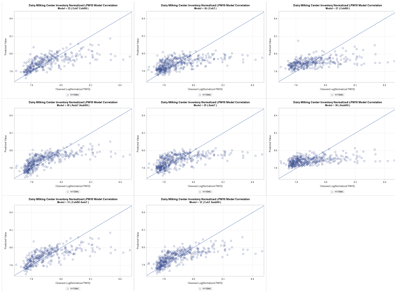
Figure G-36. Dairy milking center PM 10 one-to-one plots models 25 through 32, log transformed.
