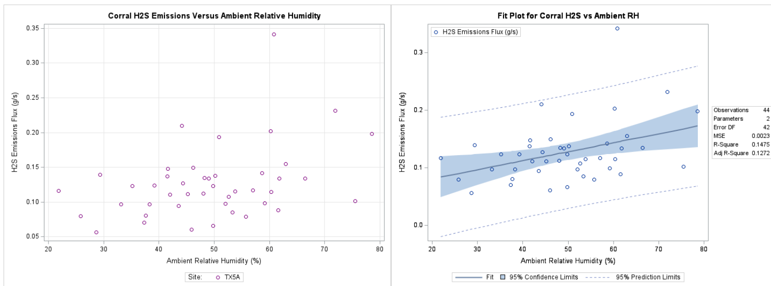
Figure F-139. Scatter plot of corral H 2 S emissions versus ambient relative humidity and scatter plot with regression.
