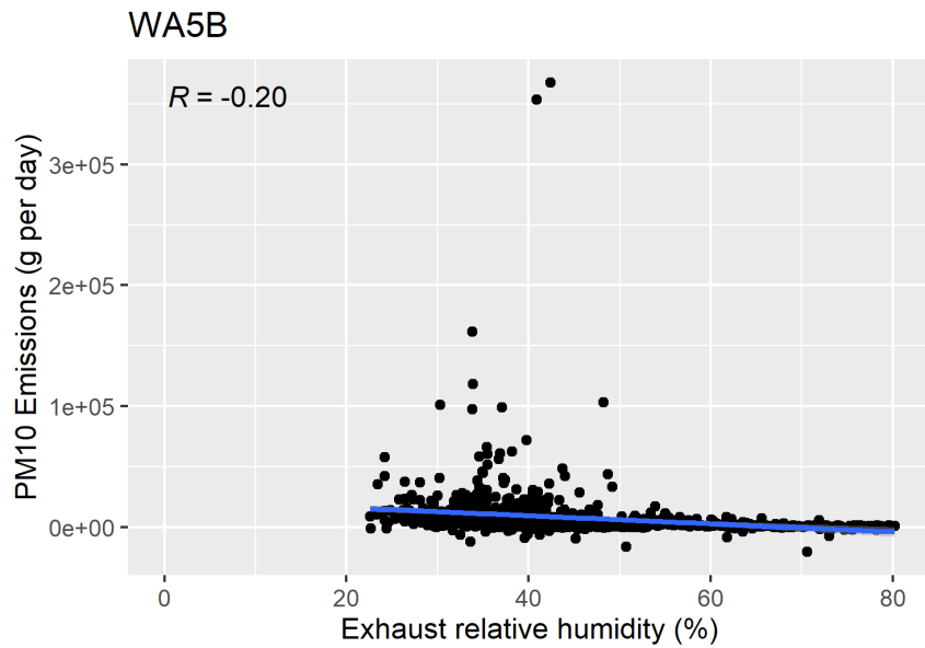
Figure F-103. Scatter plot of naturally ventilated barns PM 10 emissions versus exhaust relative humidity and scatter plot with regression.
