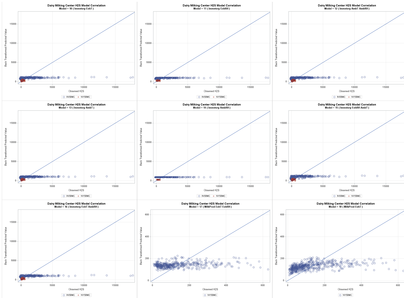
Figure G-30. Dairy milking center H 2 S one-to-one plots models 10 through 18, back transformed.
