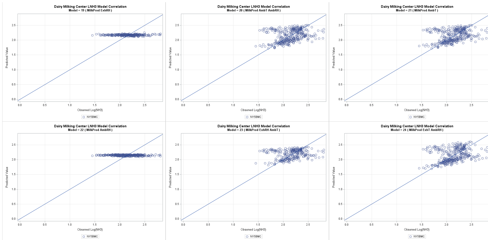
Figure G-19. Dairy milking center NH 3 one-to-one plots models 19 through 24, log transformed.
