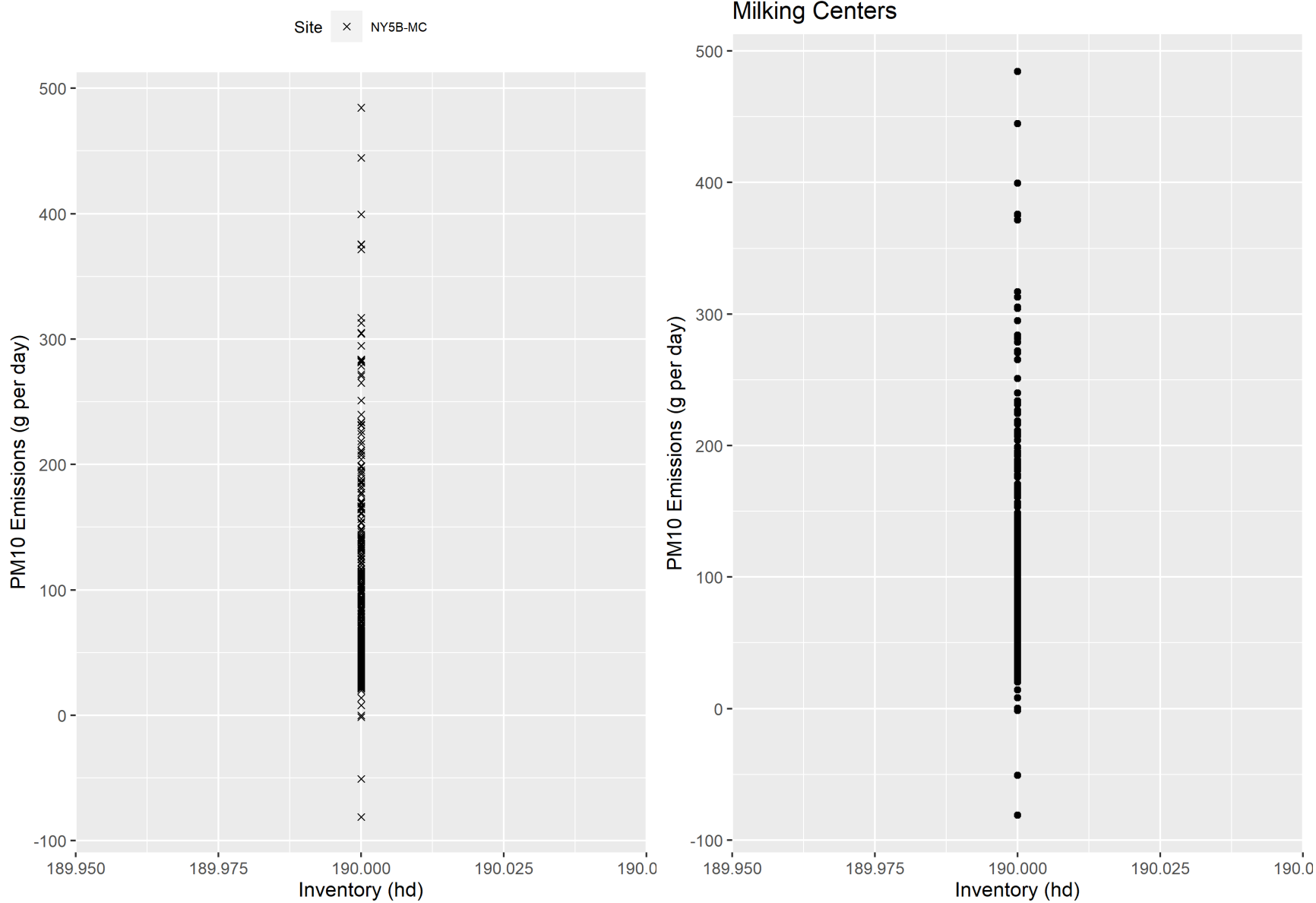
Figure F-43. Scatter plot of milking center PM 10 emissions versus inventory and scatter plot with regression.
