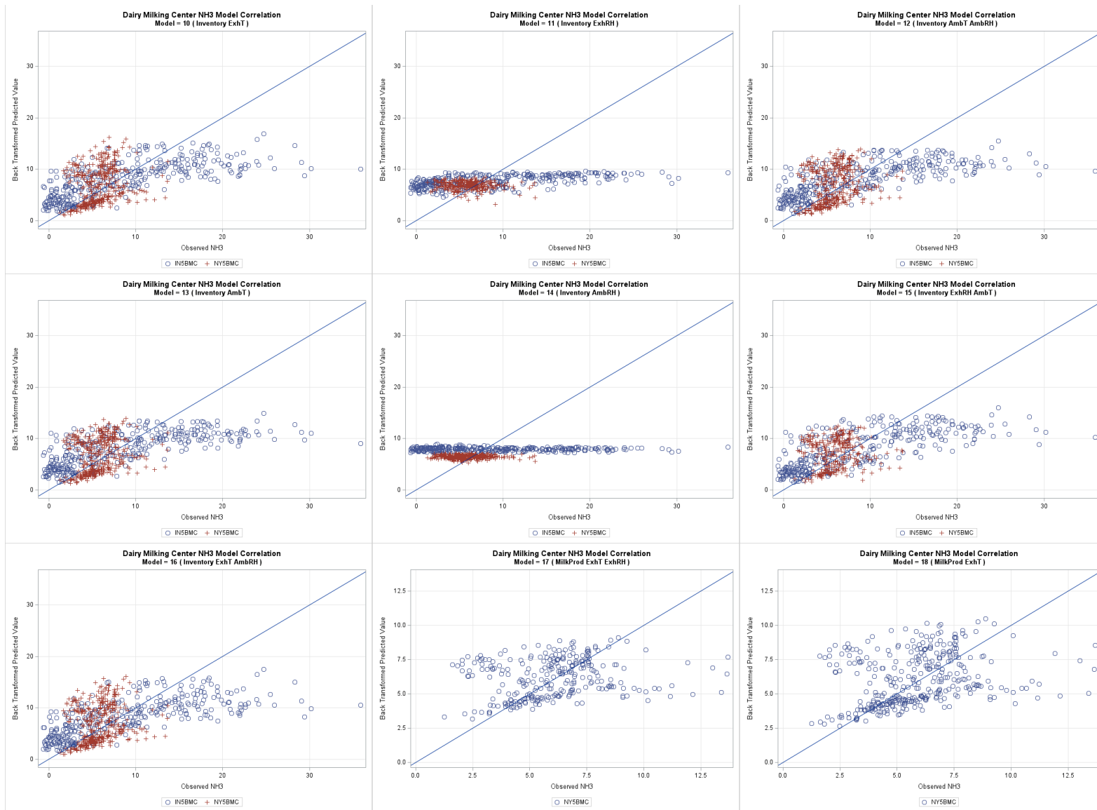
Figure G-22 Dairy milking center NH 3 one-to-one plots models 10 through 18, back transformed.
