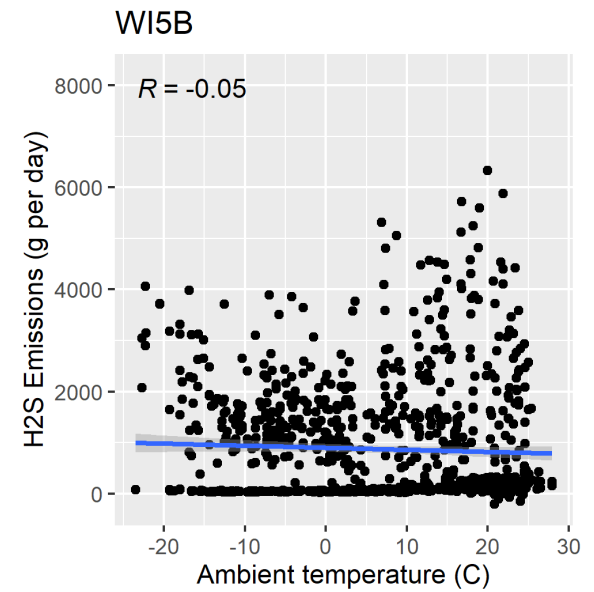
Figure F-32. Scatter plot of mechanically ventilated H 2 S emissions versus ambient temperature and scatter plot with regression.
