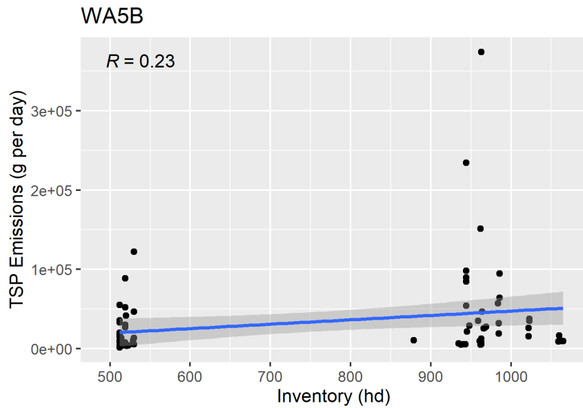
Figure F-85. Scatter plot of naturally ventilated barns TSP emissions versus inventory and scatter plot with regression.
