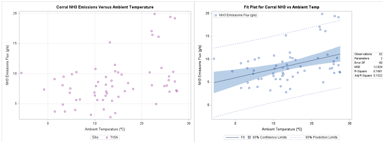
Figure F-136. Scatter plot of corral NH 3 emissions versus ambient temperature and scatter plot with regression.
