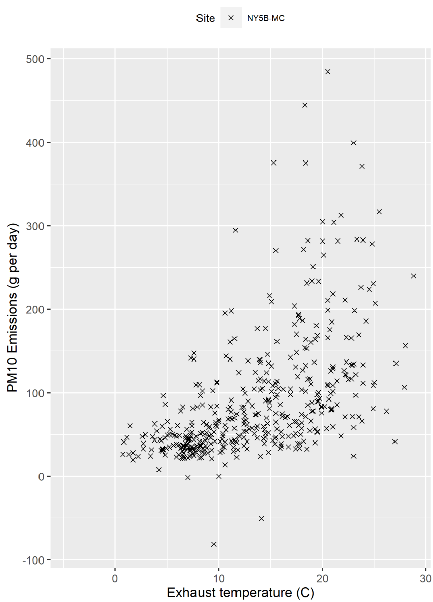
Figure F-58. Scatter plot of milking center PM 10 emissions versus exhaust temperature and scatter plot with regression.
