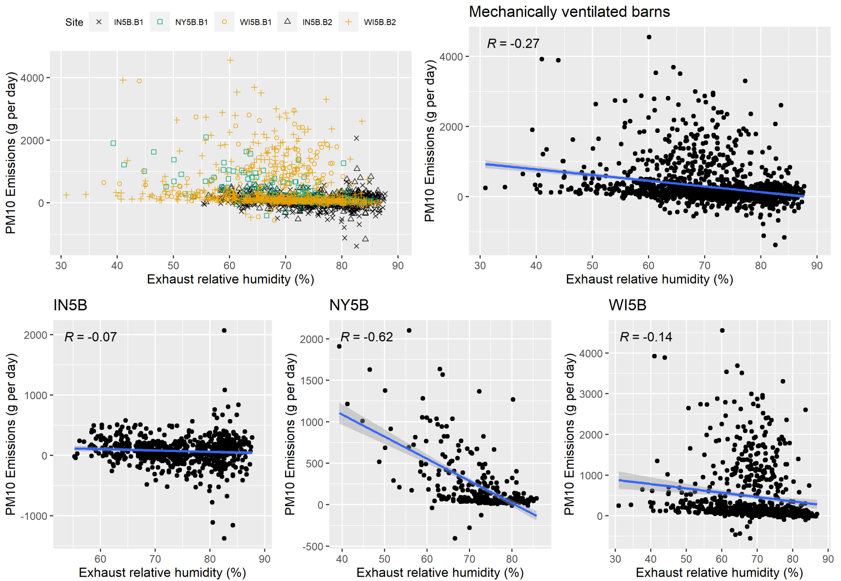
Figure F-23. Scatter plot of mechanically ventilated PM 10 emissions versus exhaust relative humidity and scatter plot with regression.
