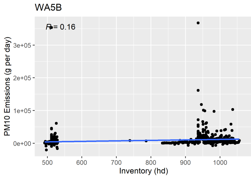
Figure F-83. Scatter plot of naturally ventilated barns PM 10 emissions versus inventory and scatter plot with regression.
