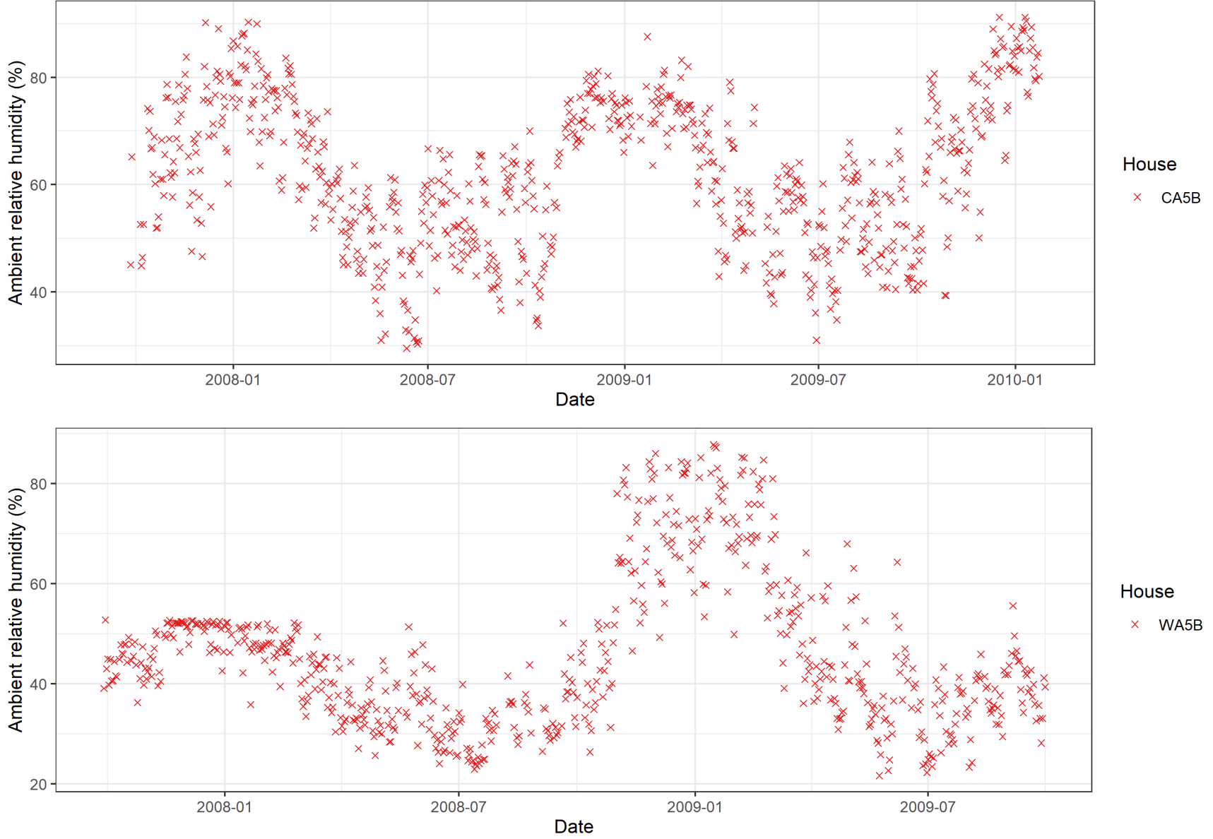
Figure E-41. Trends in ambient relative humidity at naturally ventilated barns, by site, during the NAEMS monitoring period.
