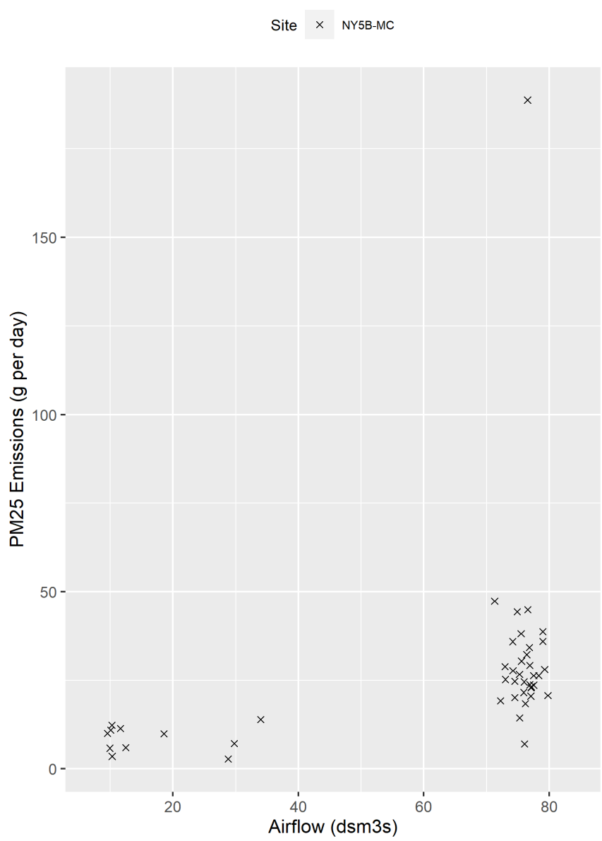
Figure F-69. Scatter plot of milking center PM 2.5 emissions versus airflow and scatter plot with regression.
