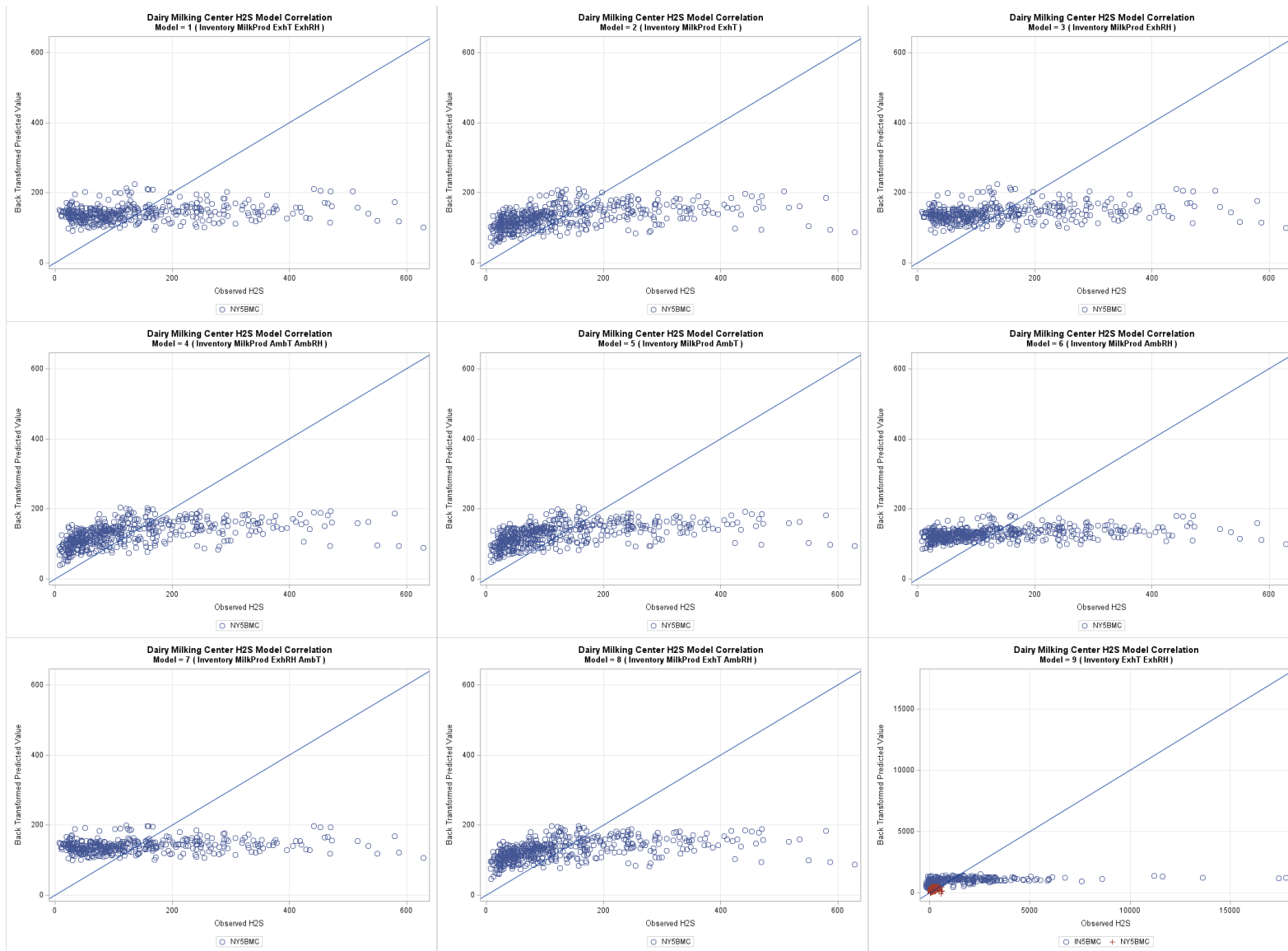
Figure G-29. Dairy milking center H 2 S one-to-one plots models 1 through 9, back transformed.
