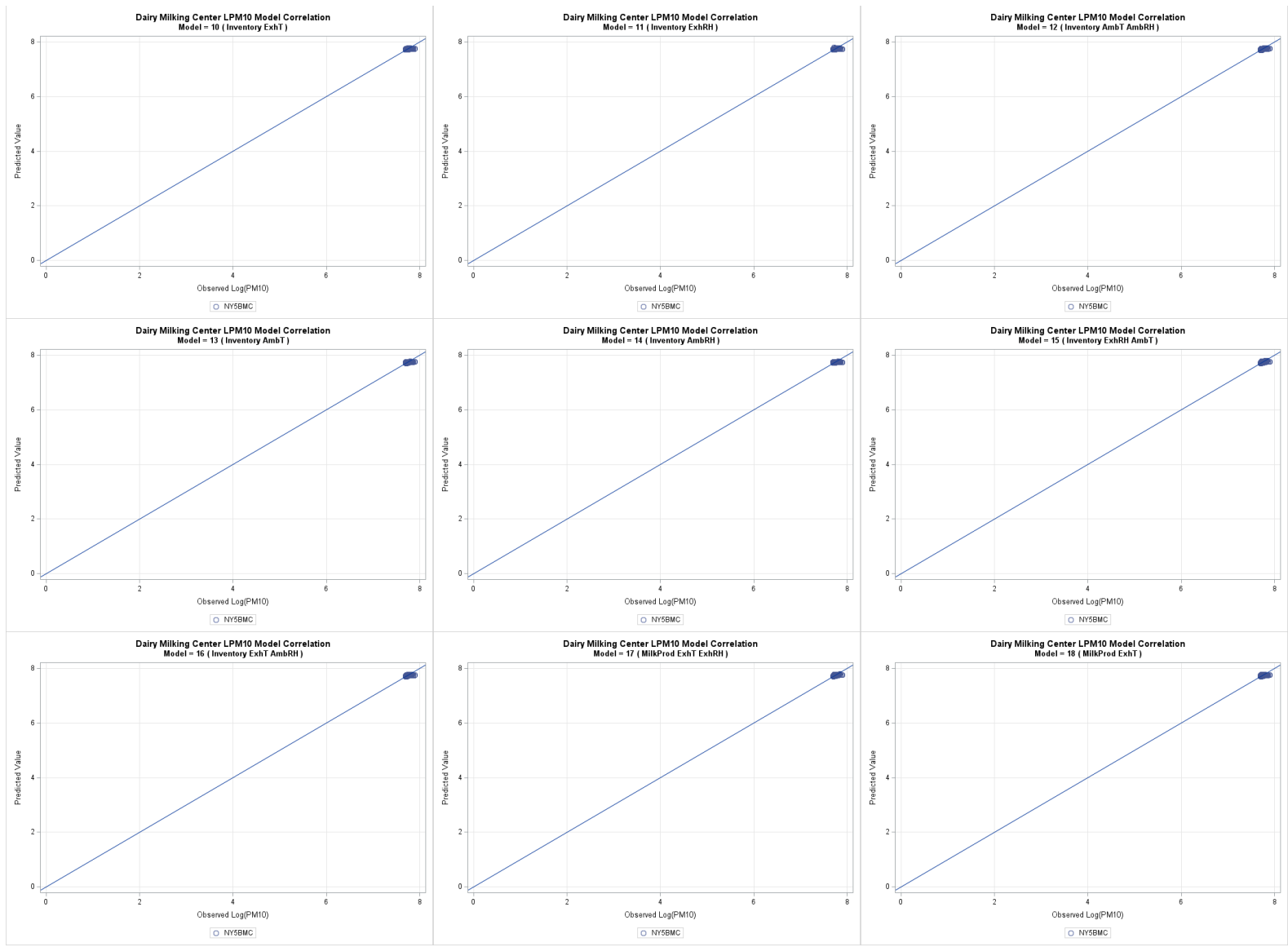
Figure G-34. Dairy milking center PM 10 one-to-one plots models 10 through 18, log transformed.
