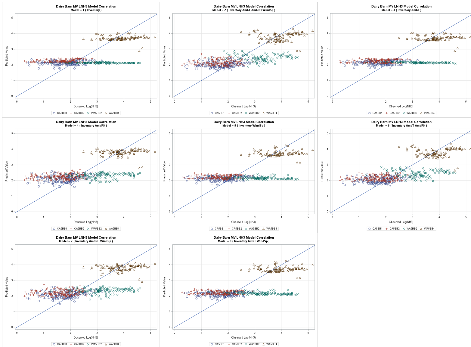
Figure G-57. Dairy naturally ventilated barn NH 3 one-to-one plots models 1 through 8, log transformed.
