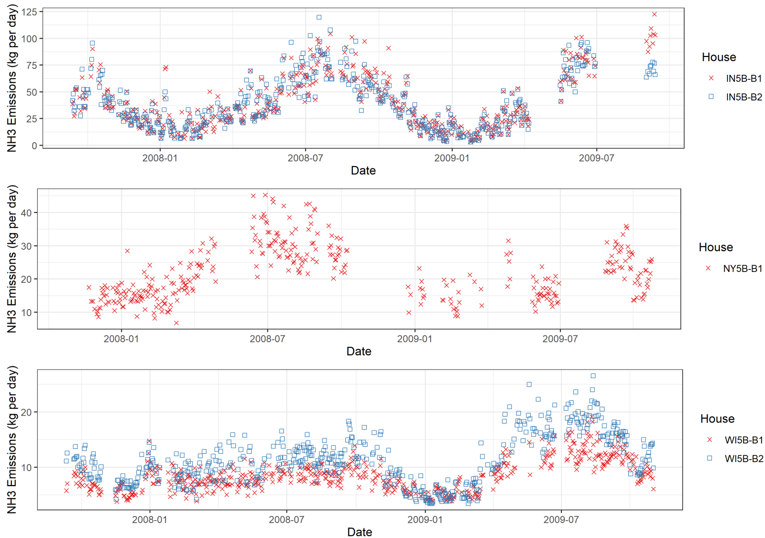
Figure E-1. Trends in NH 3 emissions at mechanically ventilated barns, by site, during the NAEMS monitoring period.
