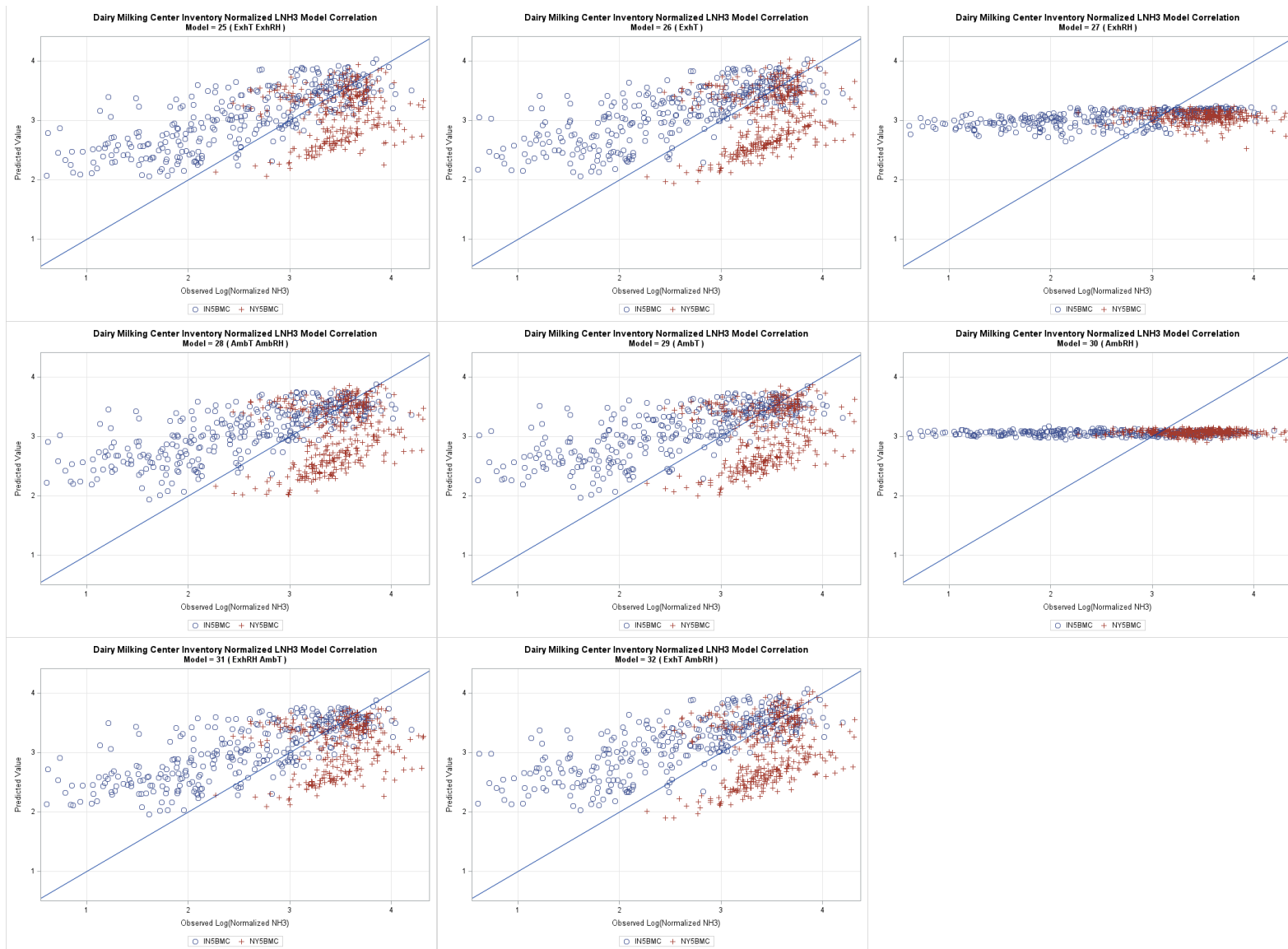
Figure G-20. Dairy milking center NH 3 one-to-one plots models 25 through 32, log transformed.
