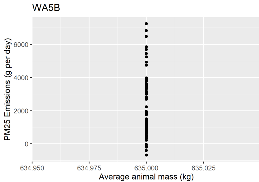
Figure F-89. Scatter plot of naturally ventilated barns PM 2.5 emissions versus average animal mass and scatter plot with regression.
