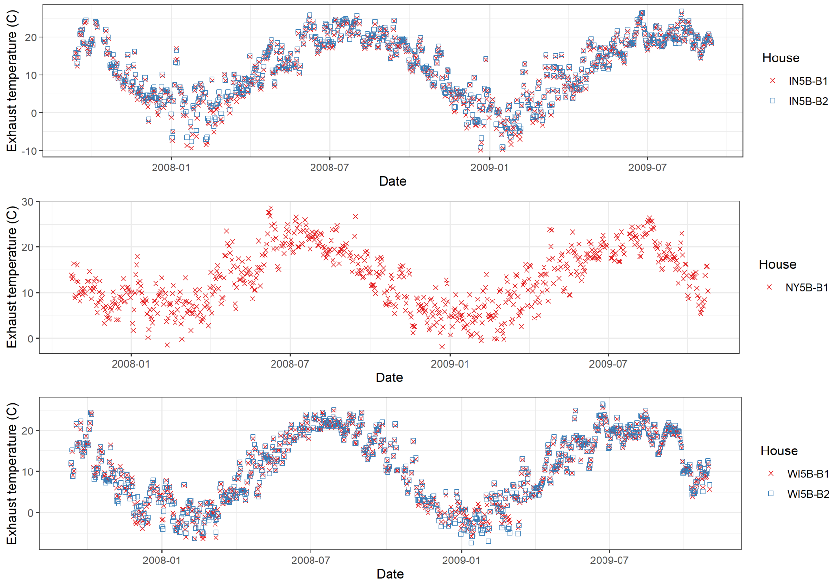
Figure E-9. Trends in exhaust temperature at mechanically ventilated barns, by site, during the NAEMS monitoring period.
