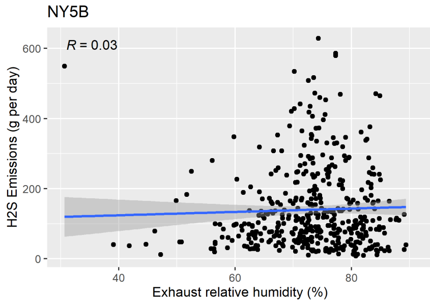
Figure F-62. Scatter plot of milking center H 2 S emissions versus exhaust relative humidity and scatter plot with regression.
