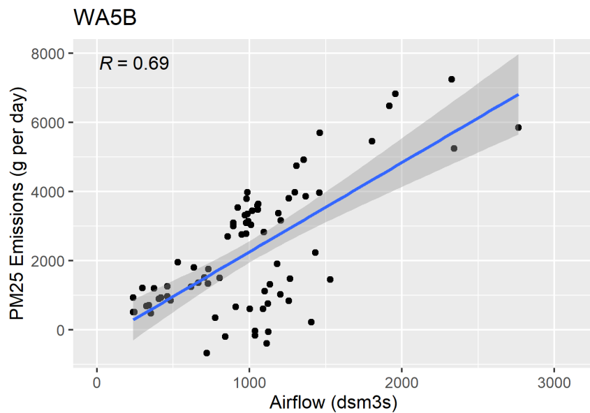
Figure F-109. Scatter plot of naturally ventilated barns PM 2.5 emissions versus airflow and scatter plot with regression.
