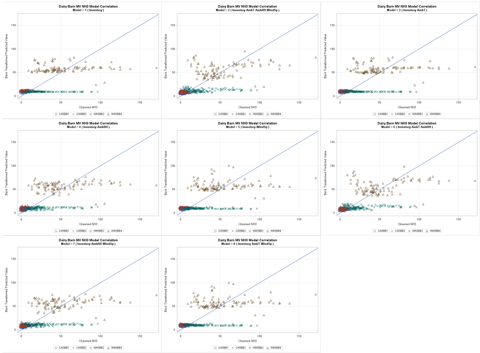
Figure G-58. Dairy naturally ventilated barn NH 3 one-to-one plots models 1 through 8, back transformed.
