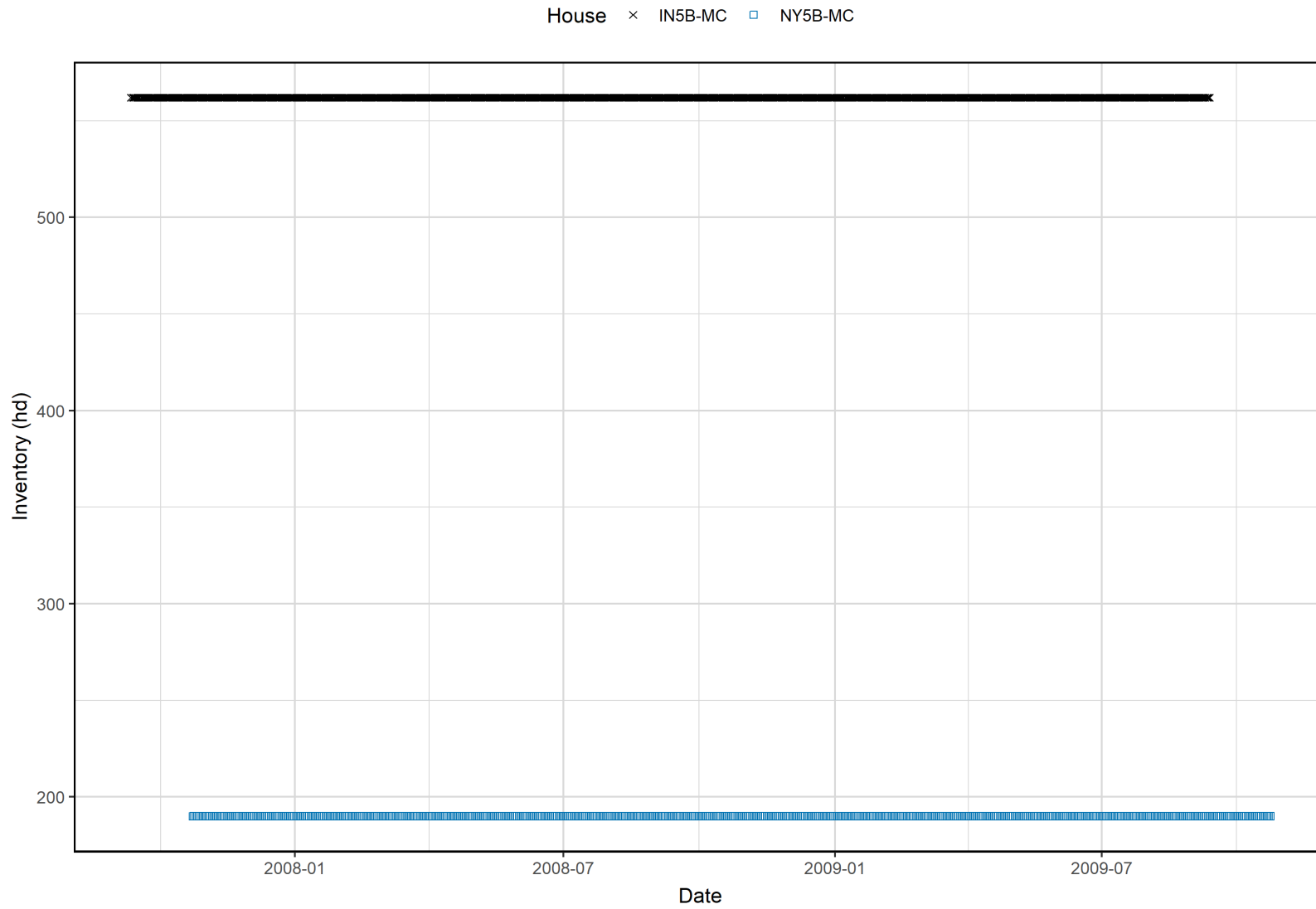
Figure E-19. Trends in inventory at milking centers, by site, during the NAEMS monitoring period.
