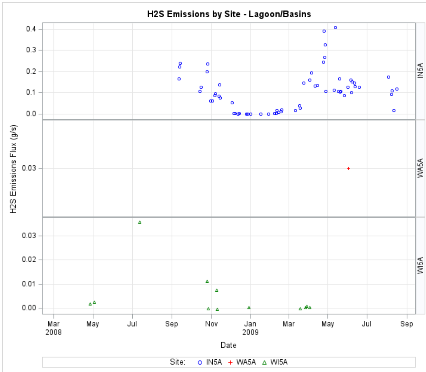
Figure E-44. Trends in H 2 S emissions at dairy lagoons, by site, during the NAEMS monitoring period.
