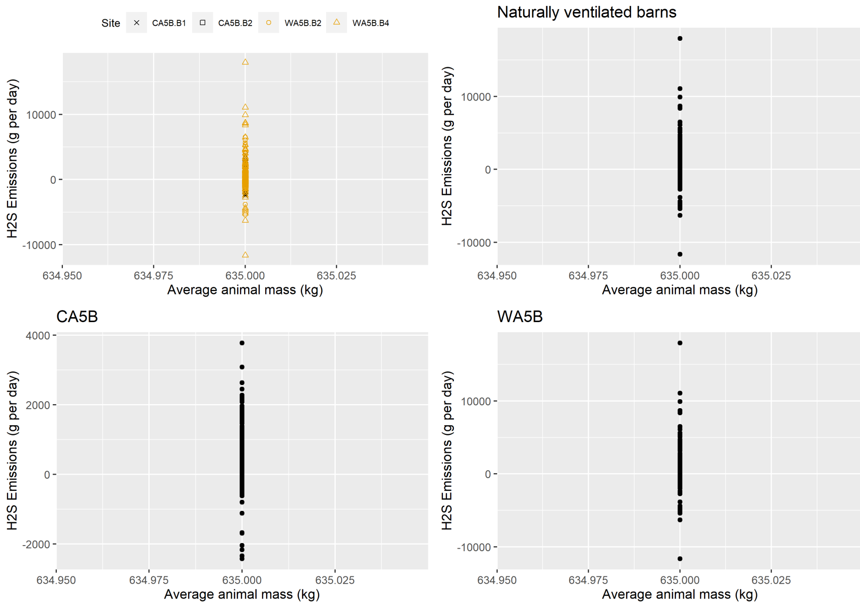
Figure F-87. Scatter plot of naturally ventilated barns H 2 S emissions versus average animal mass and scatter plot with regression.
