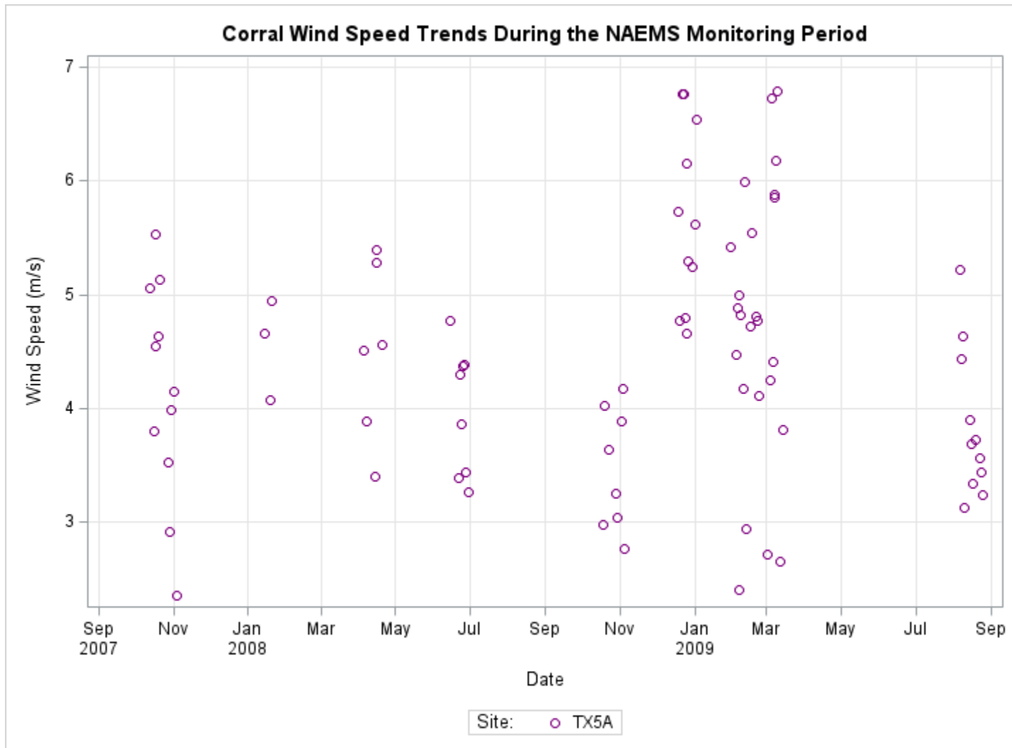
Figure E-56. Trends in corral wind speed, during the NAEMS monitoring period.
