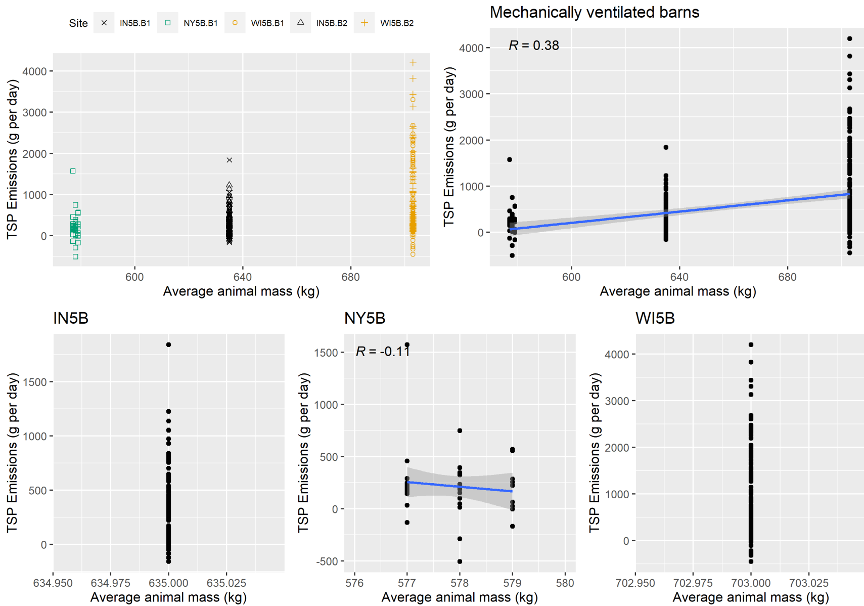
Figure F-10. Scatter plot of mechanically ventilated TSP emissions versus average animal mass and scatter plot with regression.
