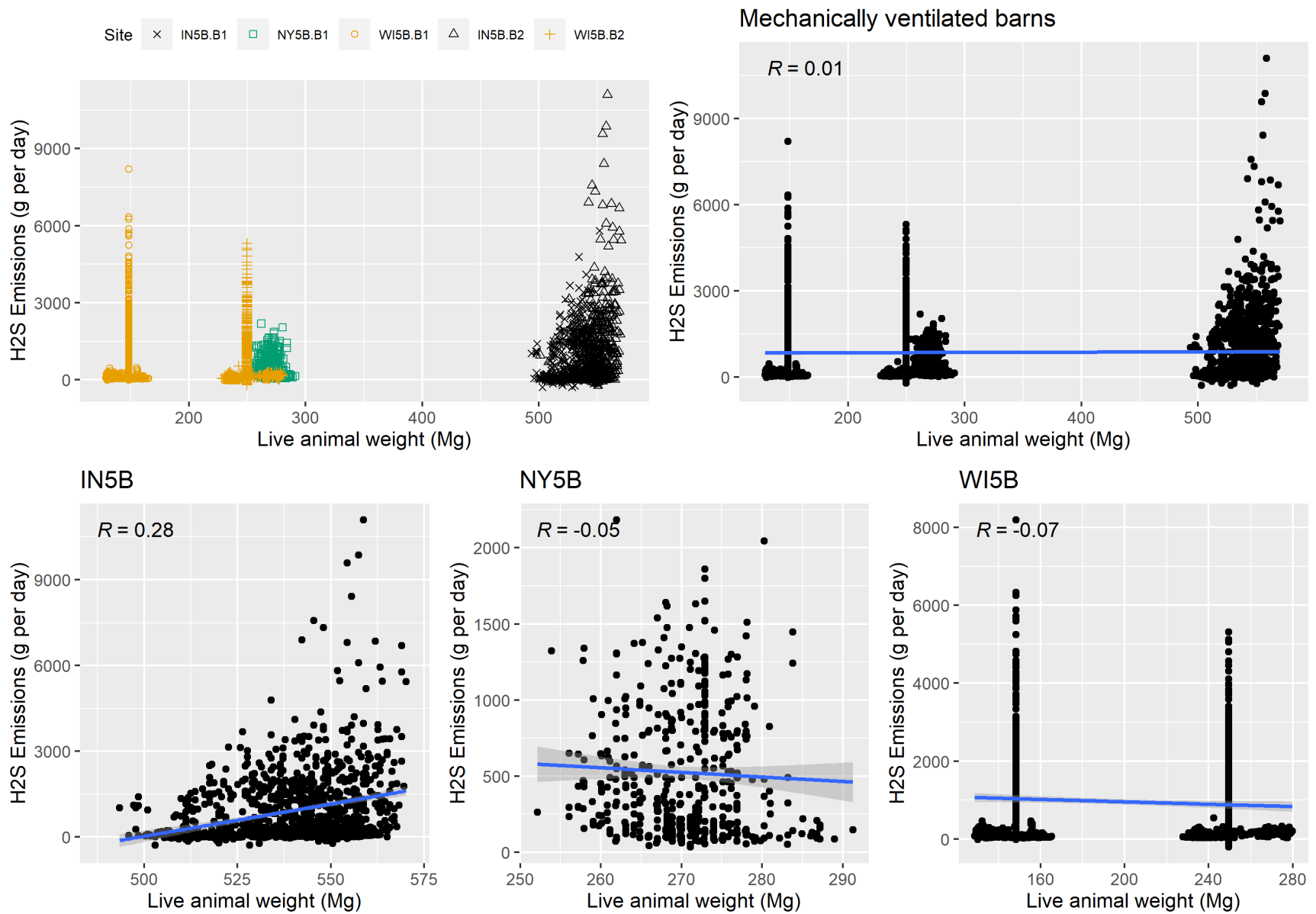
Figure F-12. Scatter plot of mechanically ventilated H 2 S emissions versus live animal weight and scatter plot with regression.
