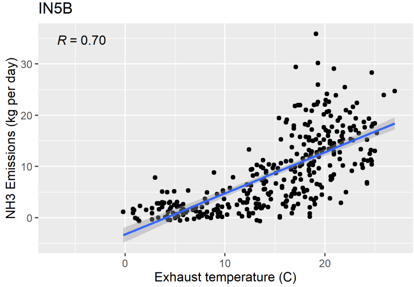
Figure F-56. Scatter plot of milking center NH 3 emissions versus exhaust temperature and scatter plot with regression.
