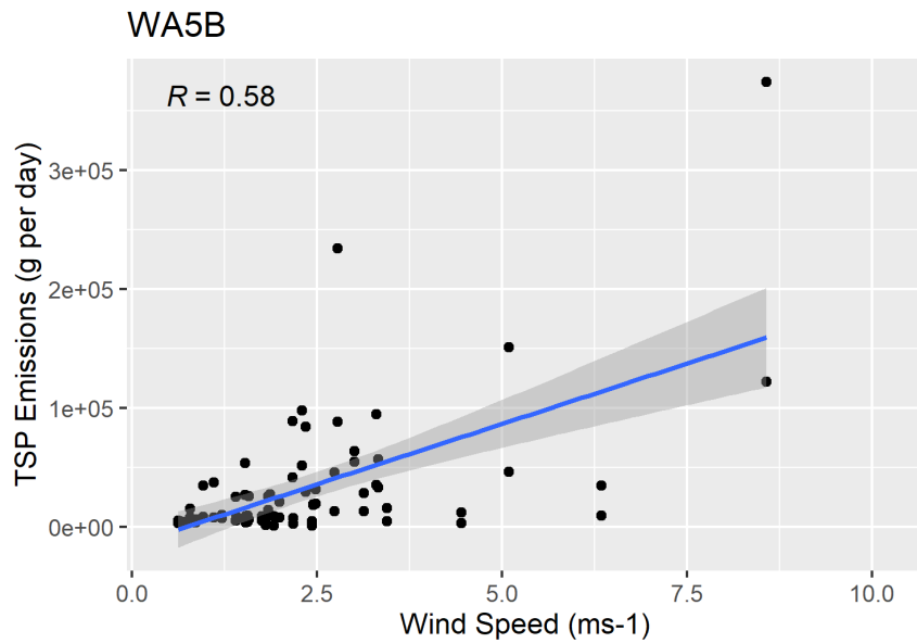
Figure F-125. Scatter plot of naturally ventilated barns TSP emissions versus wind speed and scatter plot with regression.
