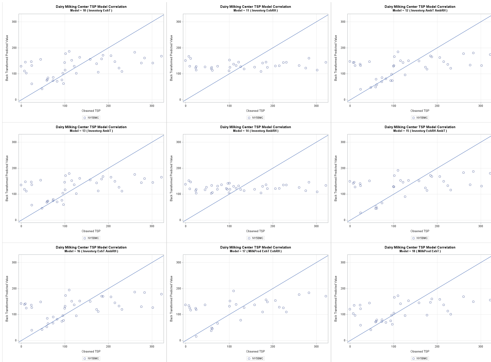
Figure G-54. Dairy milking center TSP one-to-one plots models 10 through 18, back transformed.
