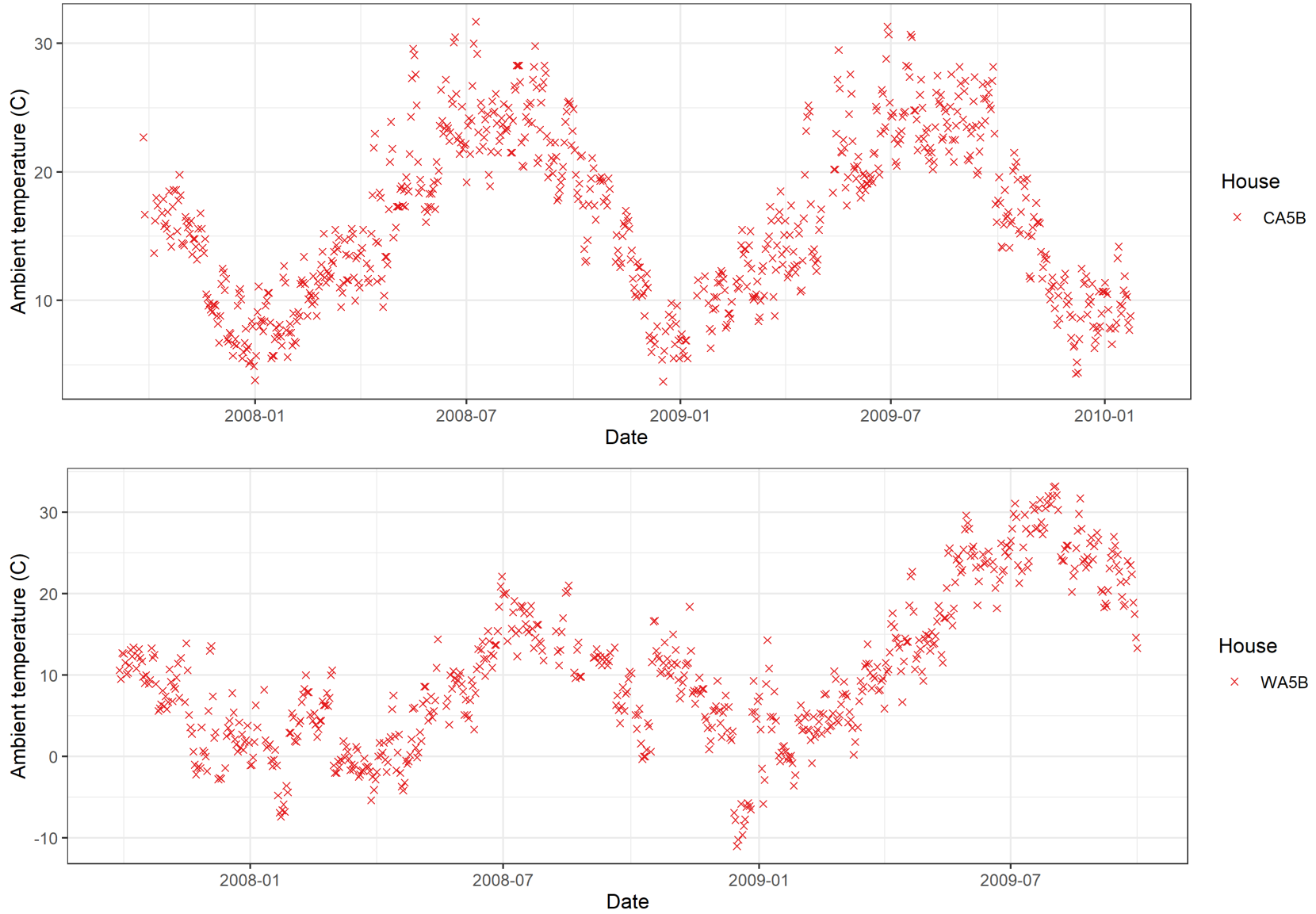
Figure E-40. Trends in ambient temperature at naturally ventilated barns, by site, during the NAEMS monitoring period.
