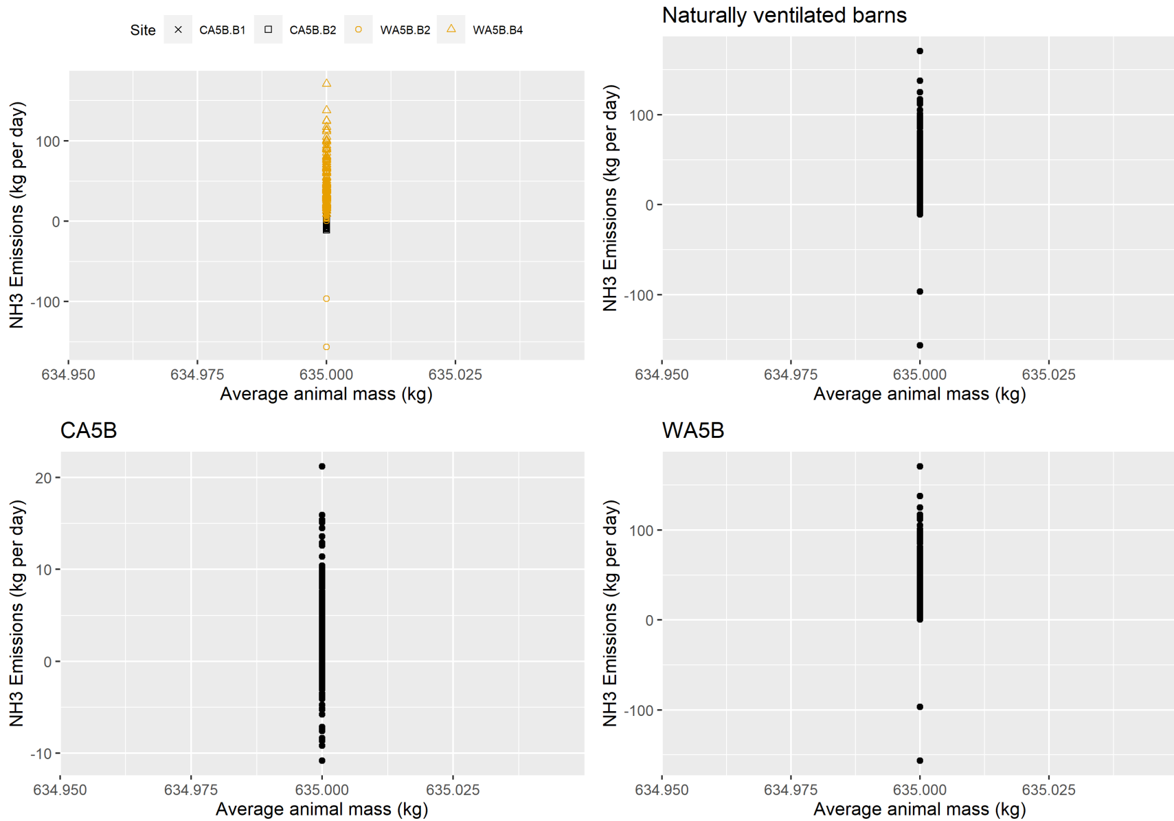
Figure F-86. Scatter plot of naturally ventilated barns NH 3 emissions versus average animal mass and scatter plot with regression.
