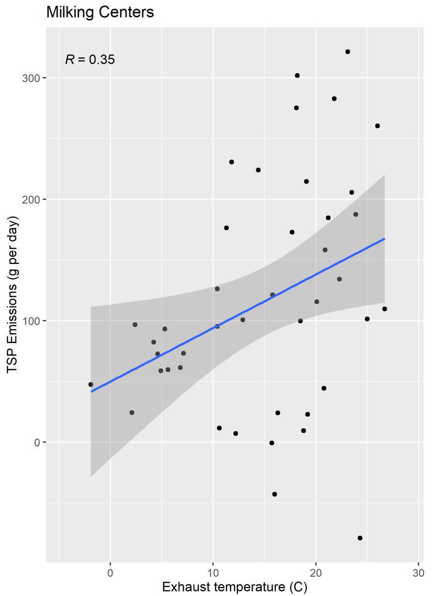
Figure F-60. Scatter plot of milking center TSP emissions versus exhaust temperature and scatter plot with regression.
