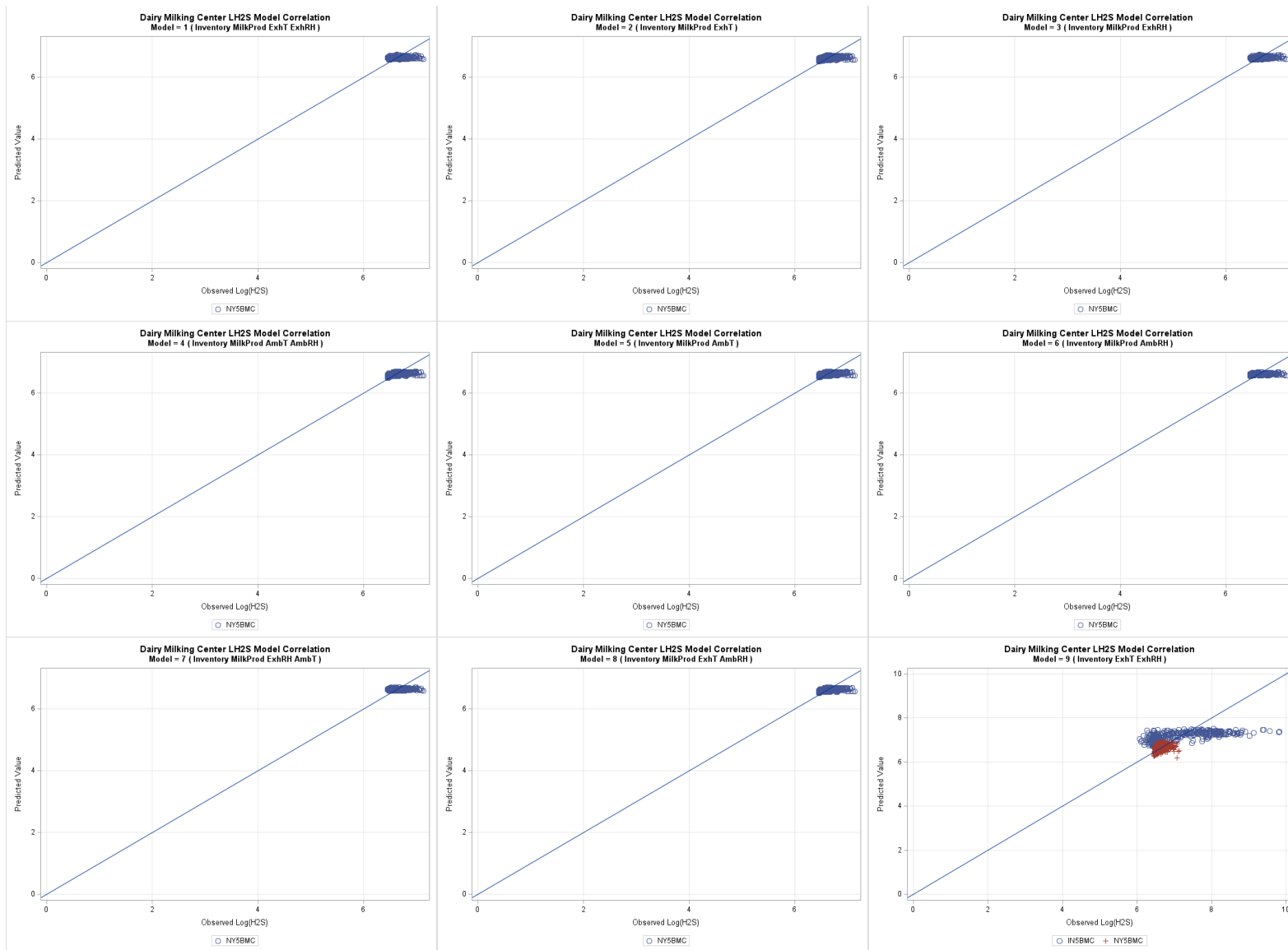
Figure G-25. Dairy milking center H 2 S one-to-one plots models 1 through 9, log transformed.
