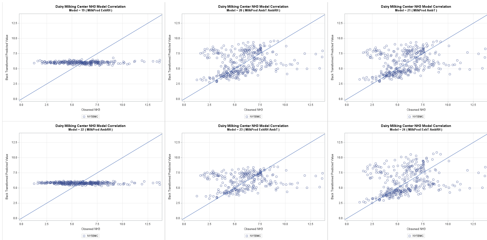
Figure G-23 Dairy milking center NH 3 one-to-one plots models 19 through 24, back transformed.
