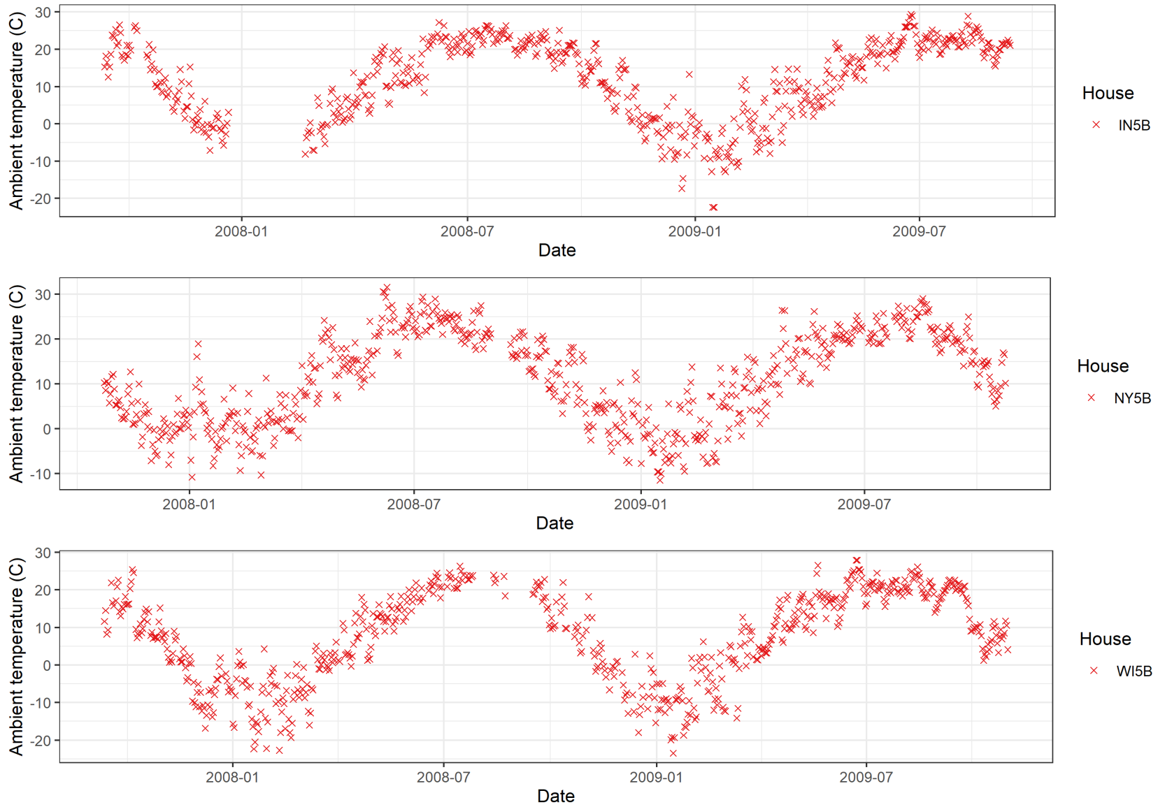
Figure E-12. Trends in ambient temperature at mechanically ventilated barns, by site, during the NAEMS monitoring period.
