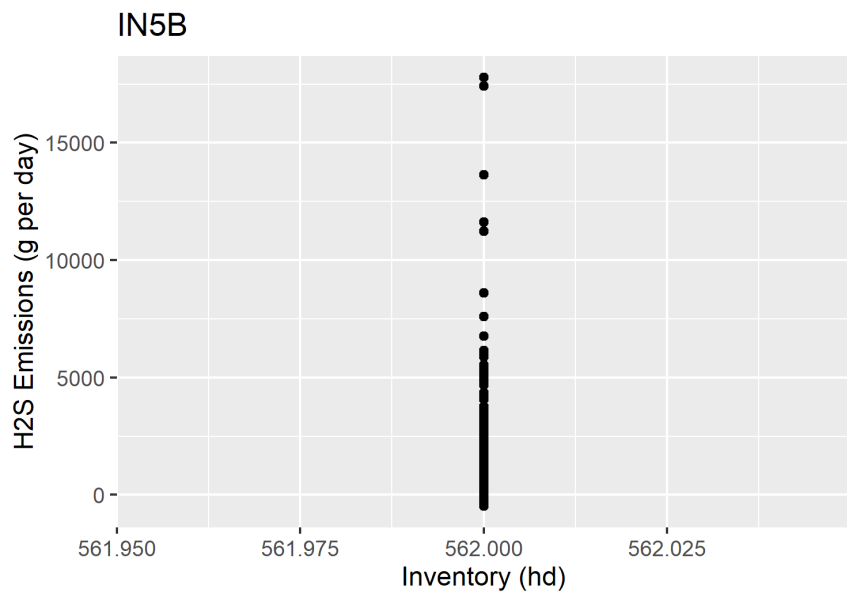
Figure F-42. Scatter plot of milking center H 2 S emissions versus inventory and scatter plot with regression.
