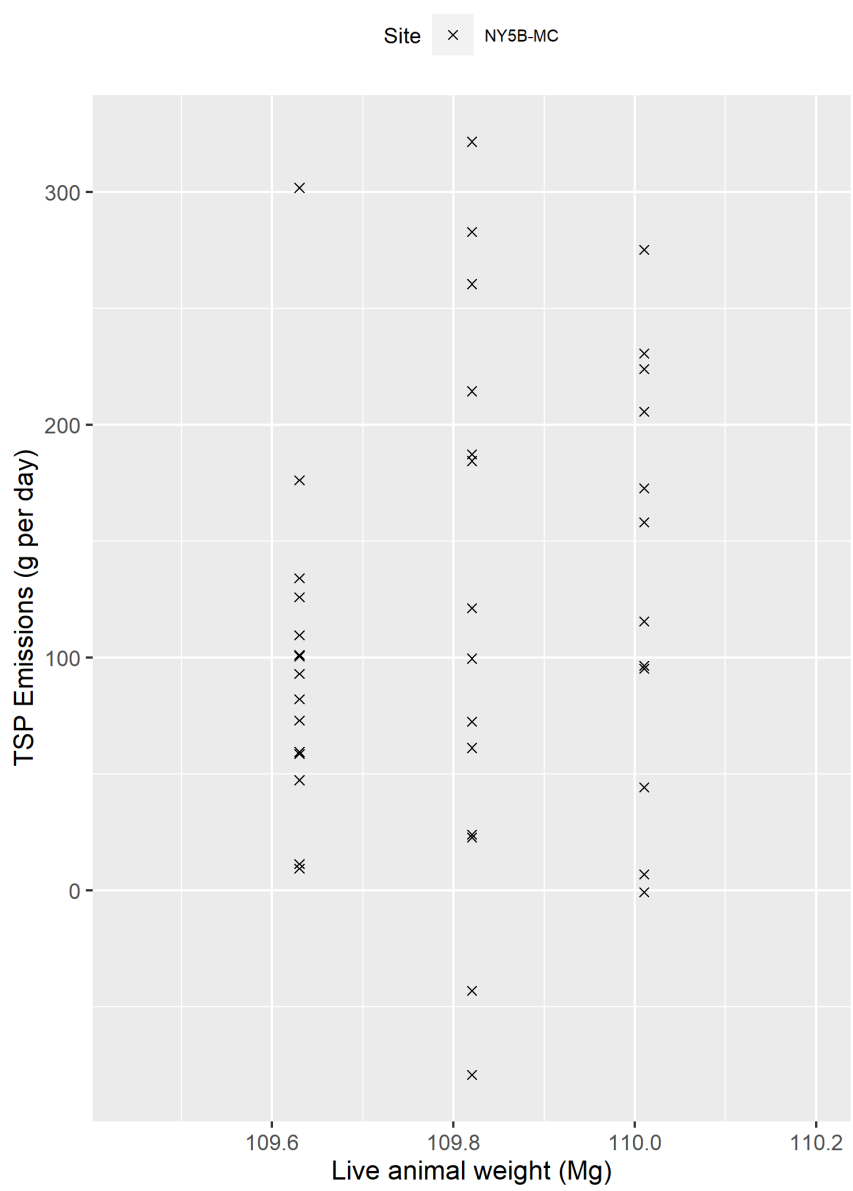
Figure F-55. Scatter plot of milking center TSP emissions versus live animal weight and scatter plot with regression.
