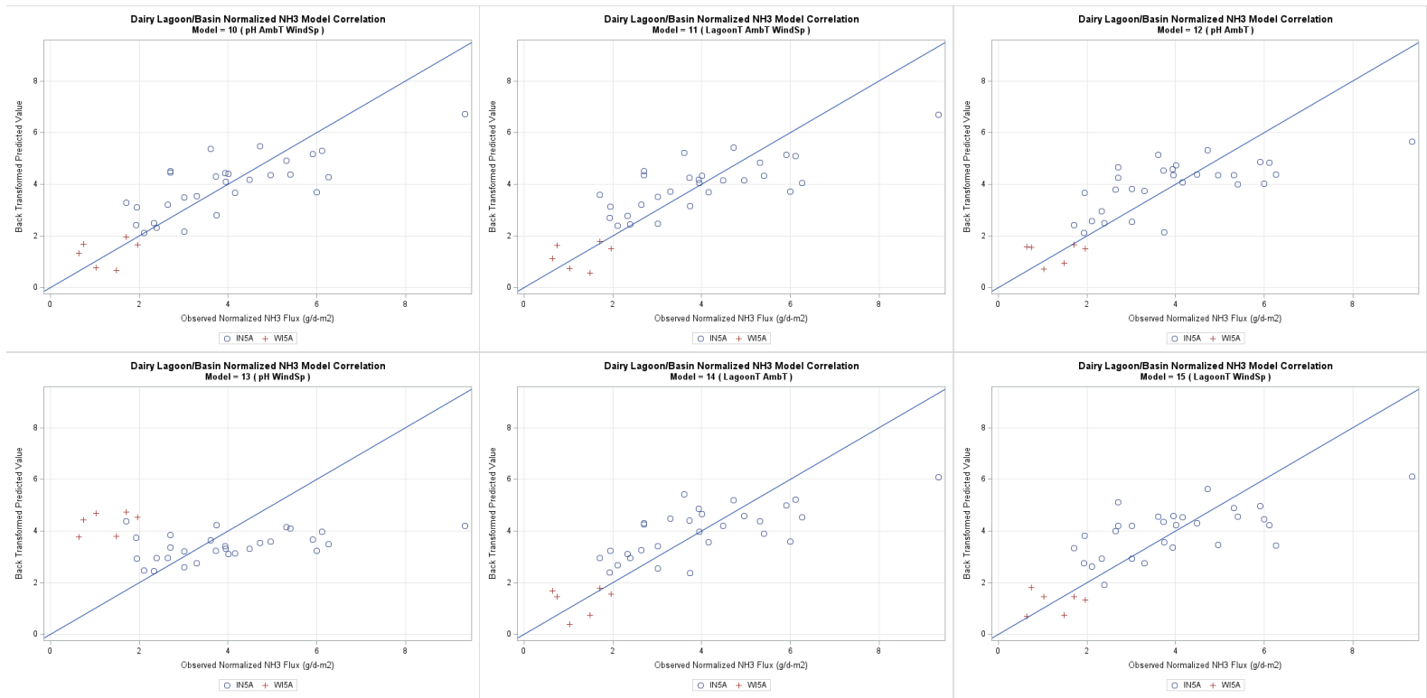
Figure G-70. Dairy lagoon NH 3 one-to-one plots models 10 through 15, back transformed.
