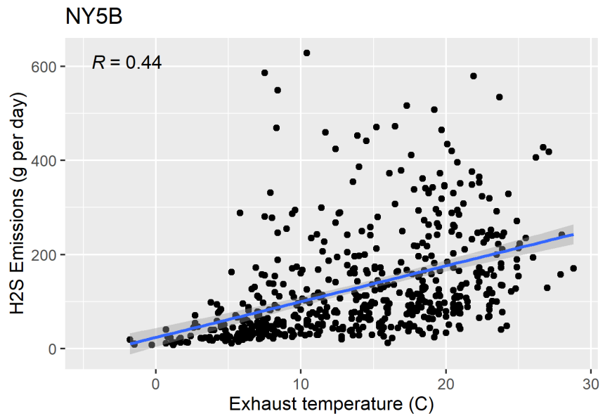
Figure F-57. Scatter plot of milking center H 2 S emissions versus exhaust temperature and scatter plot with regression.
