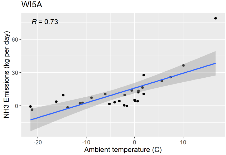
Figure F-130. Scatter plot of lagoon/basin NH 3 emissions versus ambient temperature and scatter plot with regression.
