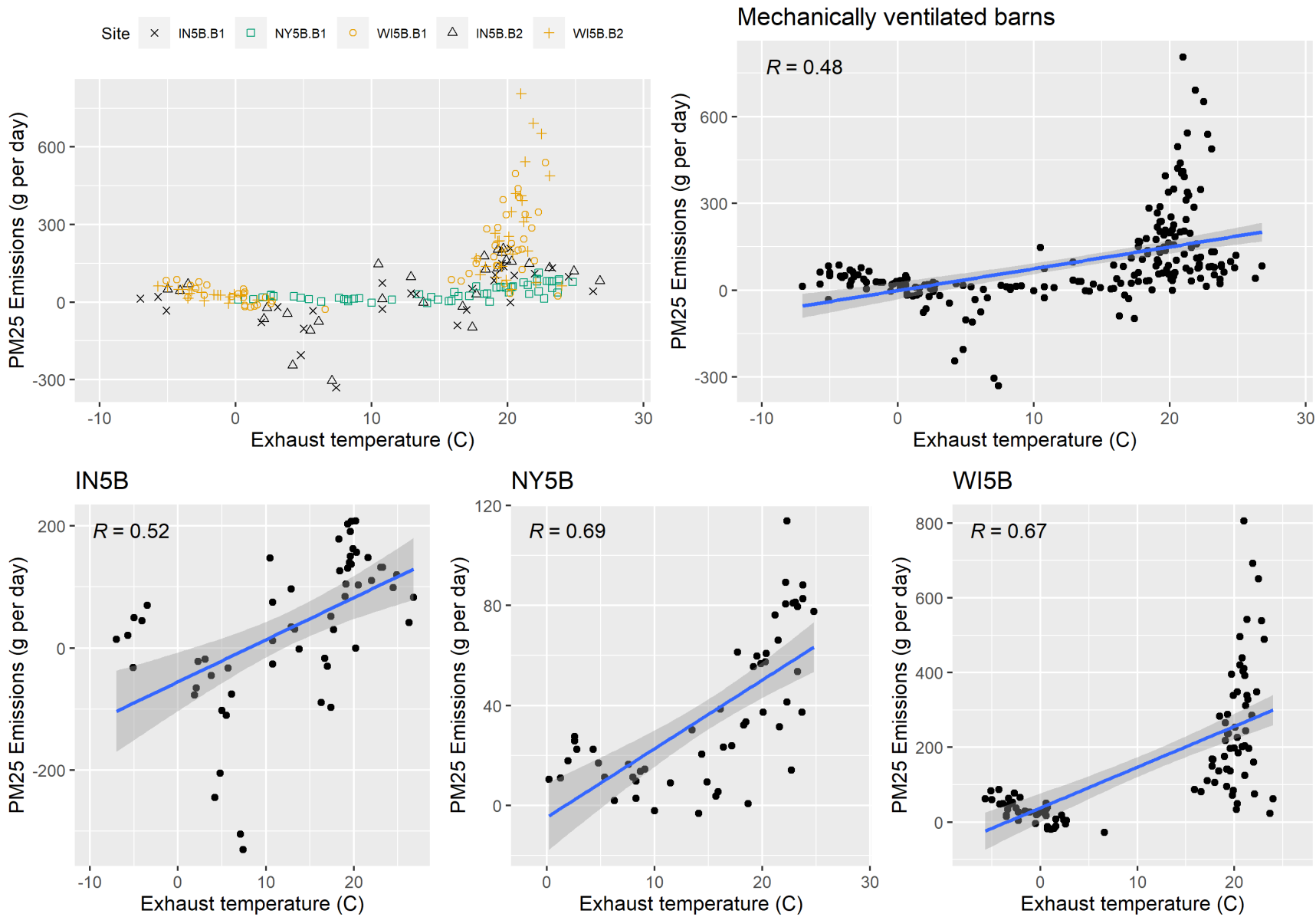
Figure F-19. Scatter plot of mechanically ventilated PM 2.5 emissions versus exhaust temperature and scatter plot with regression.
