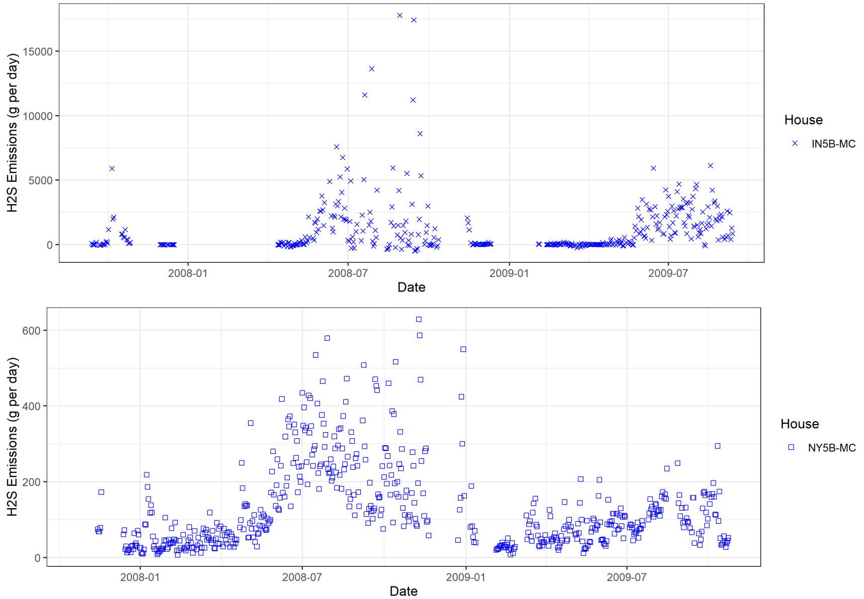
Figure E-15. NAEMS milking center H 2 S emission trends, by site.
