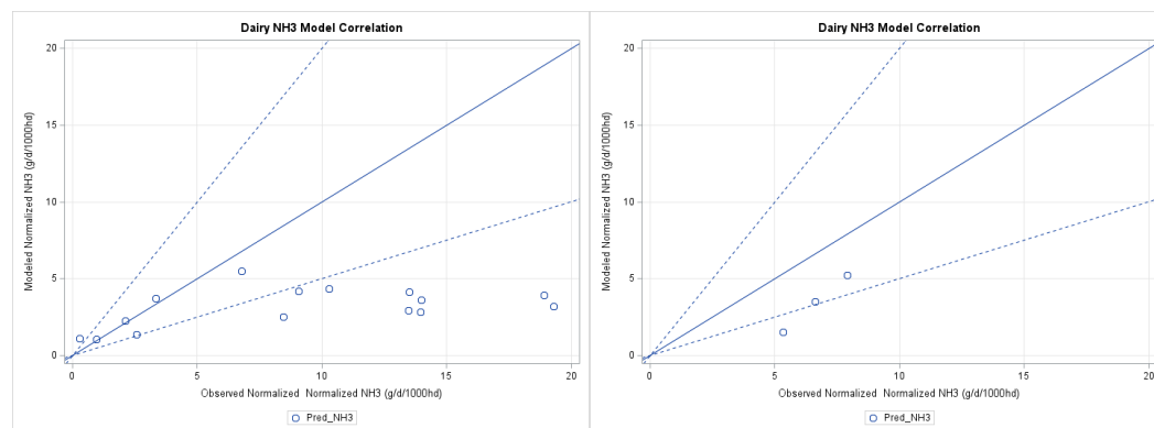
Figure 8-25. Scatter plot of the observed lagoon NH 3 emissions versus the emission model estimates.
