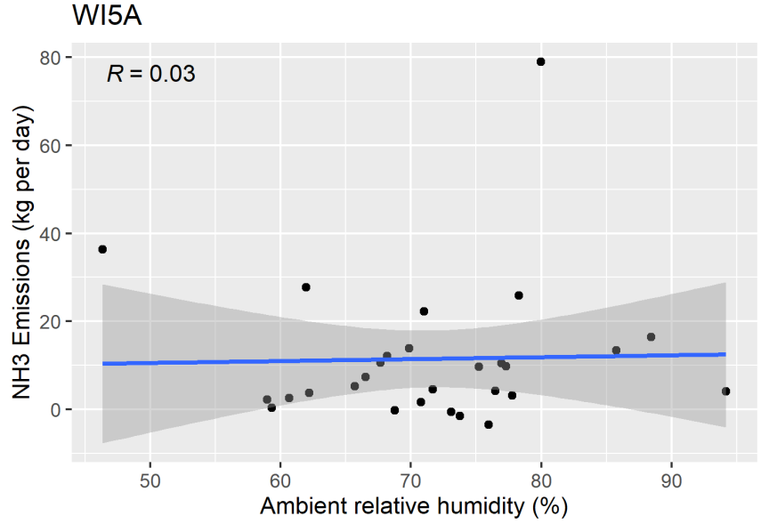
Figure F-132. Scatter plot of lagoon/basin NH 3 emissions versus ambient relative humidity and scatter plot with regression.
