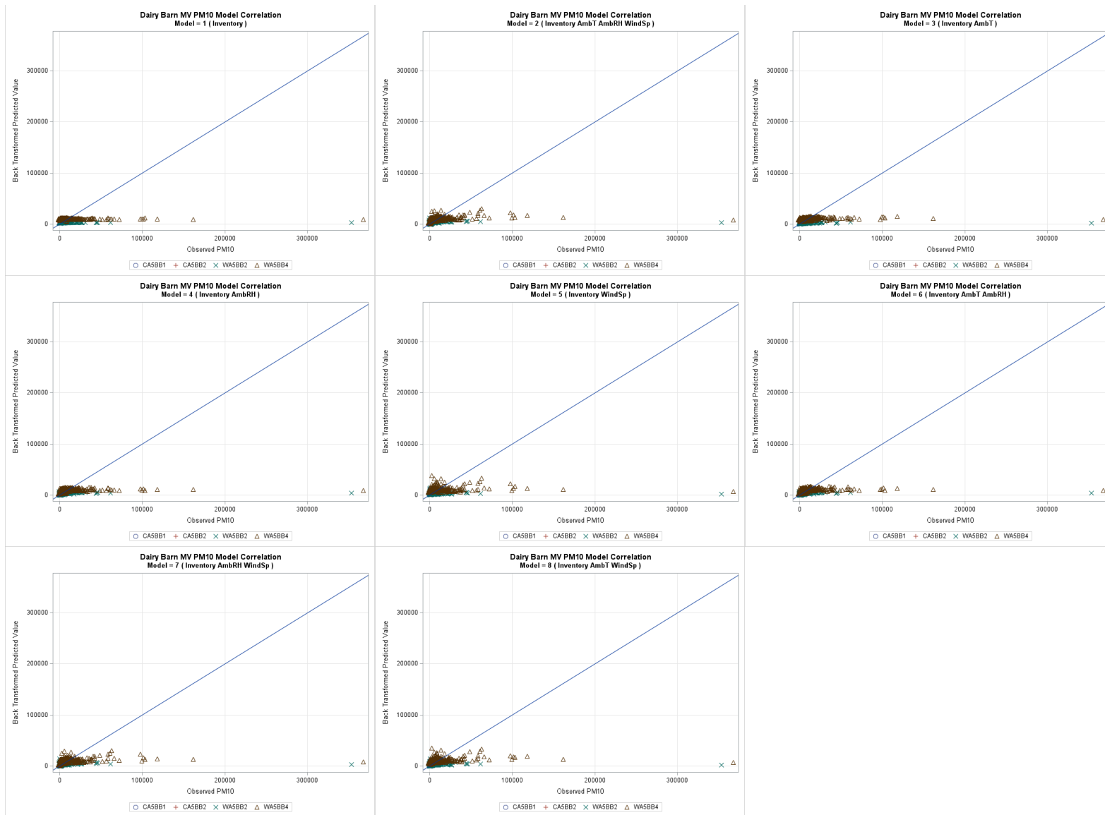
Figure G-62. Dairy naturally ventilated barn PM 10 one-to-one plots models 1 through 8, back transformed.
