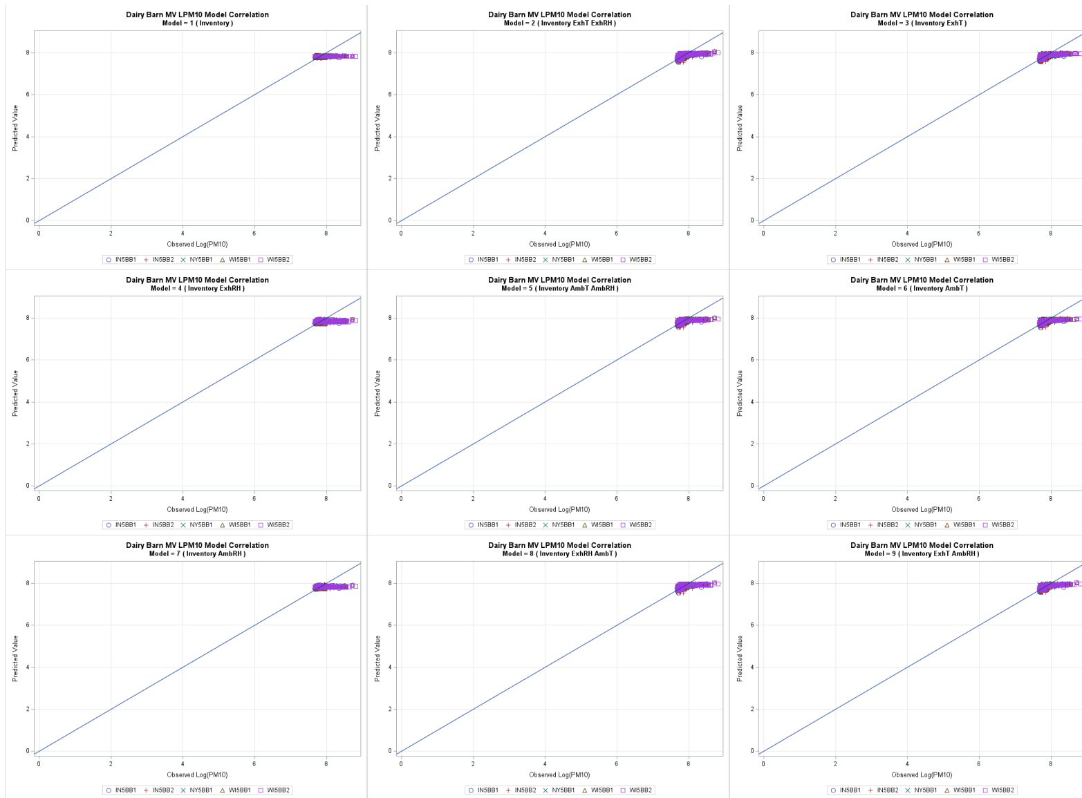
Figure G-5. Dairy mechanically ventilated barn PM 10 one-to-one plots models 1 through 9, log transformed.
