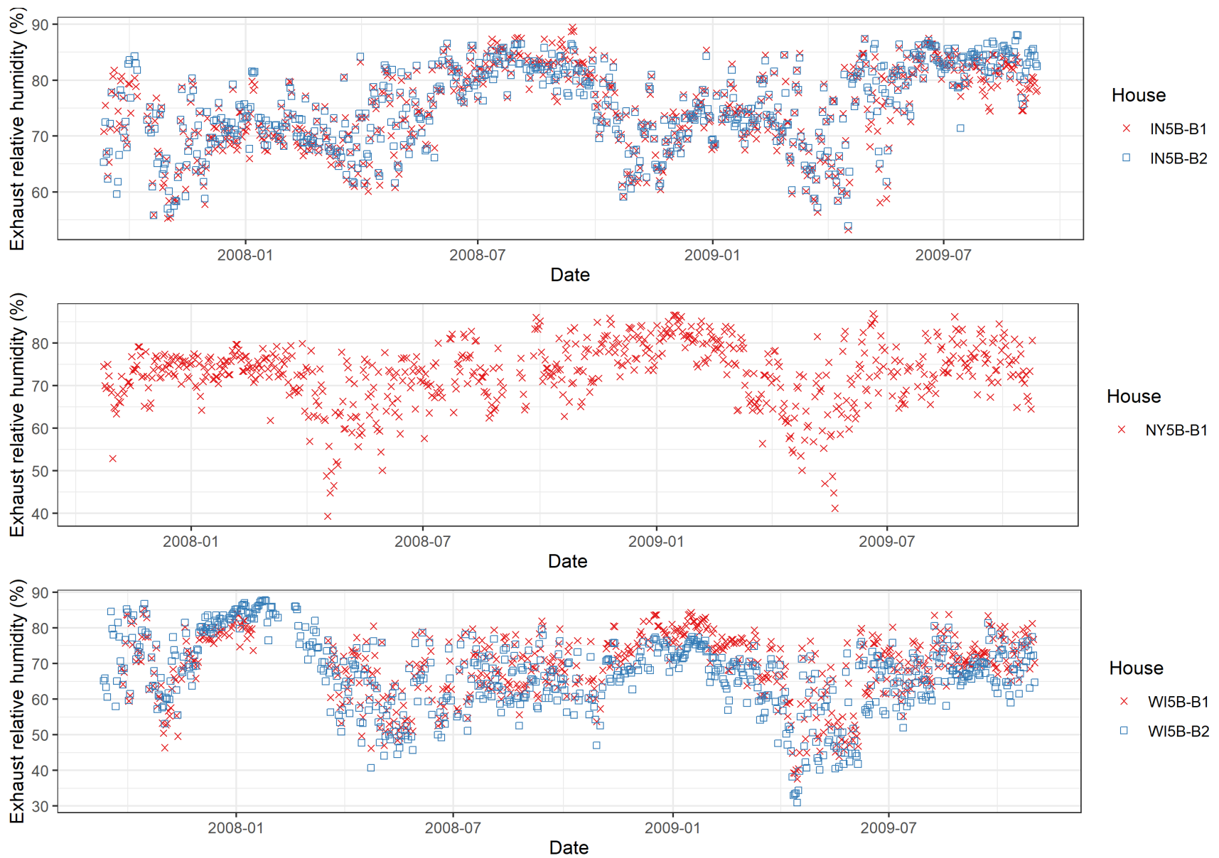
Figure E-10. Trends in exhaust relative humidity at mechanically ventilated barns, by site, during the NAEMS monitoring period.
