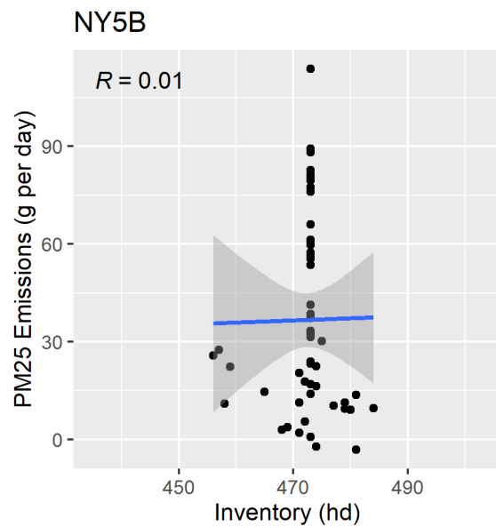
Figure F-4. Scatter plot of mechanically ventilated PM 2.5 emissions versus inventory and scatter plot with regression.
