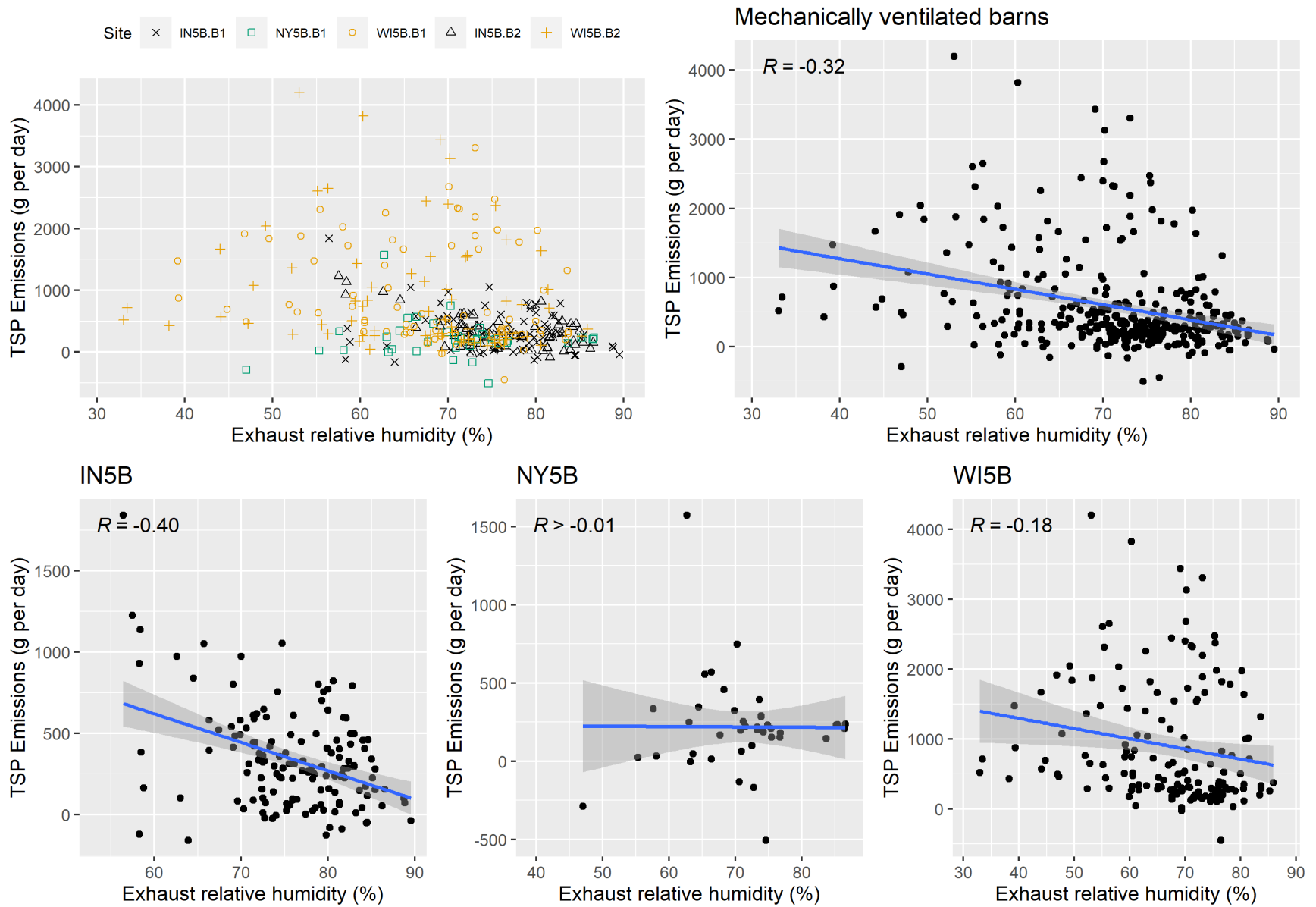
Figure F-25. Scatter plot of mechanically ventilated TSP emissions versus exhaust relative humidity and scatter plot with regression.
