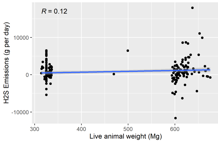
Figure F-92. Scatter plot of naturally ventilated barns H 2 S emissions versus live animal weight and scatter plot with regression.
