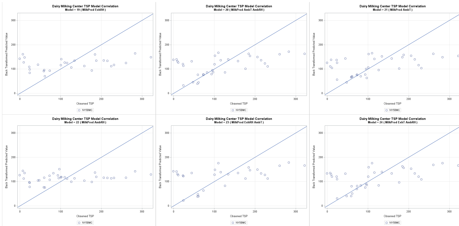
Figure G-55. Dairy milking center TSP one-to-one plots models 19 through 24, back transformed.
