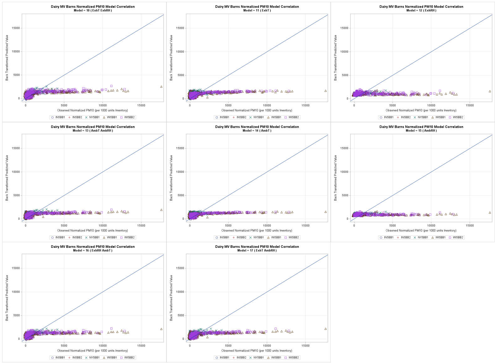
Figure G-8. Dairy mechanically ventilated barn PM 10 one-to-one plots models 10 through 17, back transformed.
