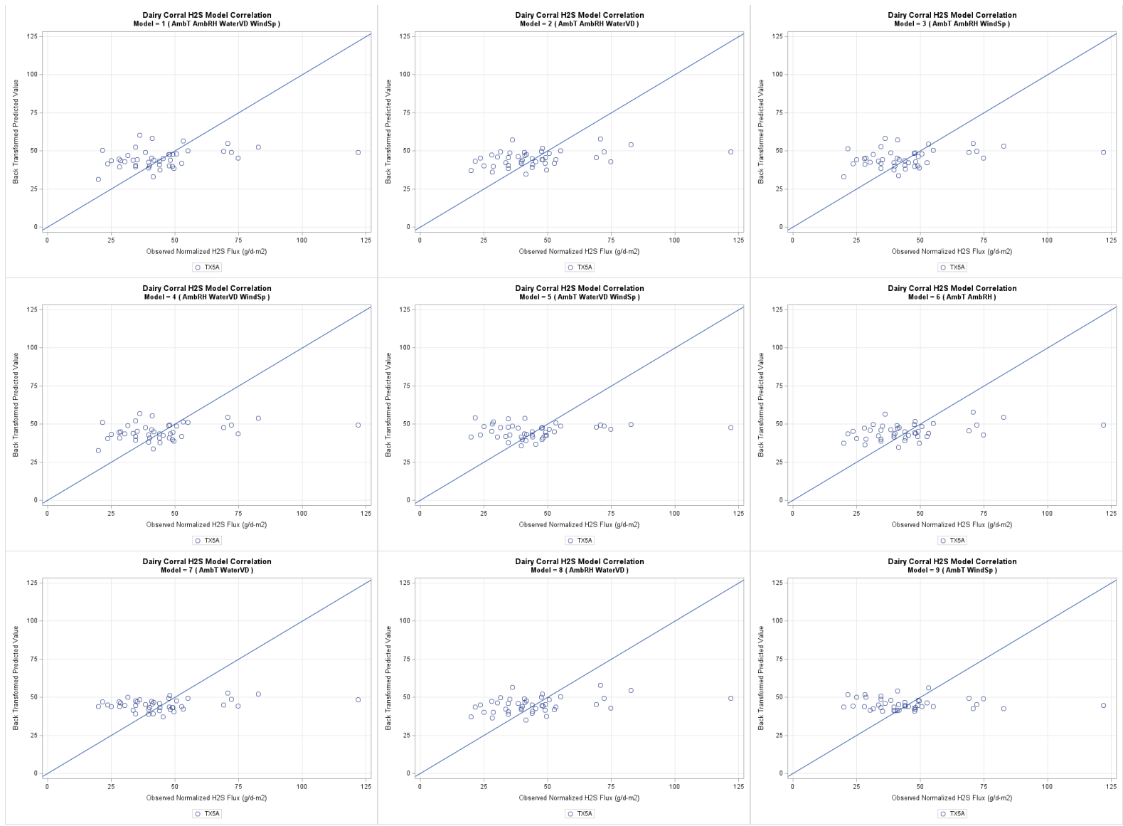
Figure G-87. Dairy corral H 2 S one-to-one plots models 1a through 9a, back transformed.
