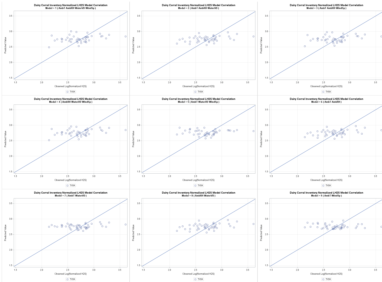
Figure G-85. Dairy corral H 2 S one-to-one plots models 1b through 9b, log transformed.
