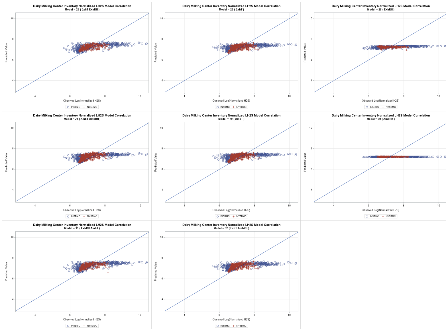
Figure G-28. Dairy milking center H 2 S one-to-one plots models 25 through 32, log transformed.
