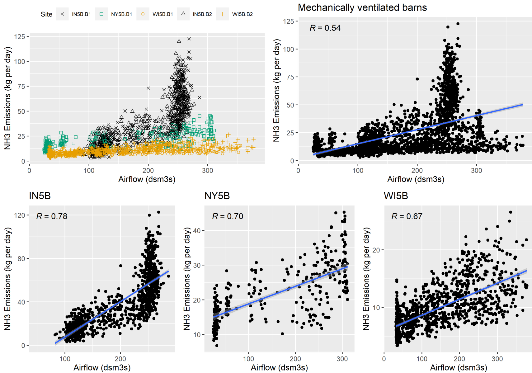
Figure F-26. Scatter plot of mechanically ventilated NH 3 emissions versus airflow and scatter plot with regression.
