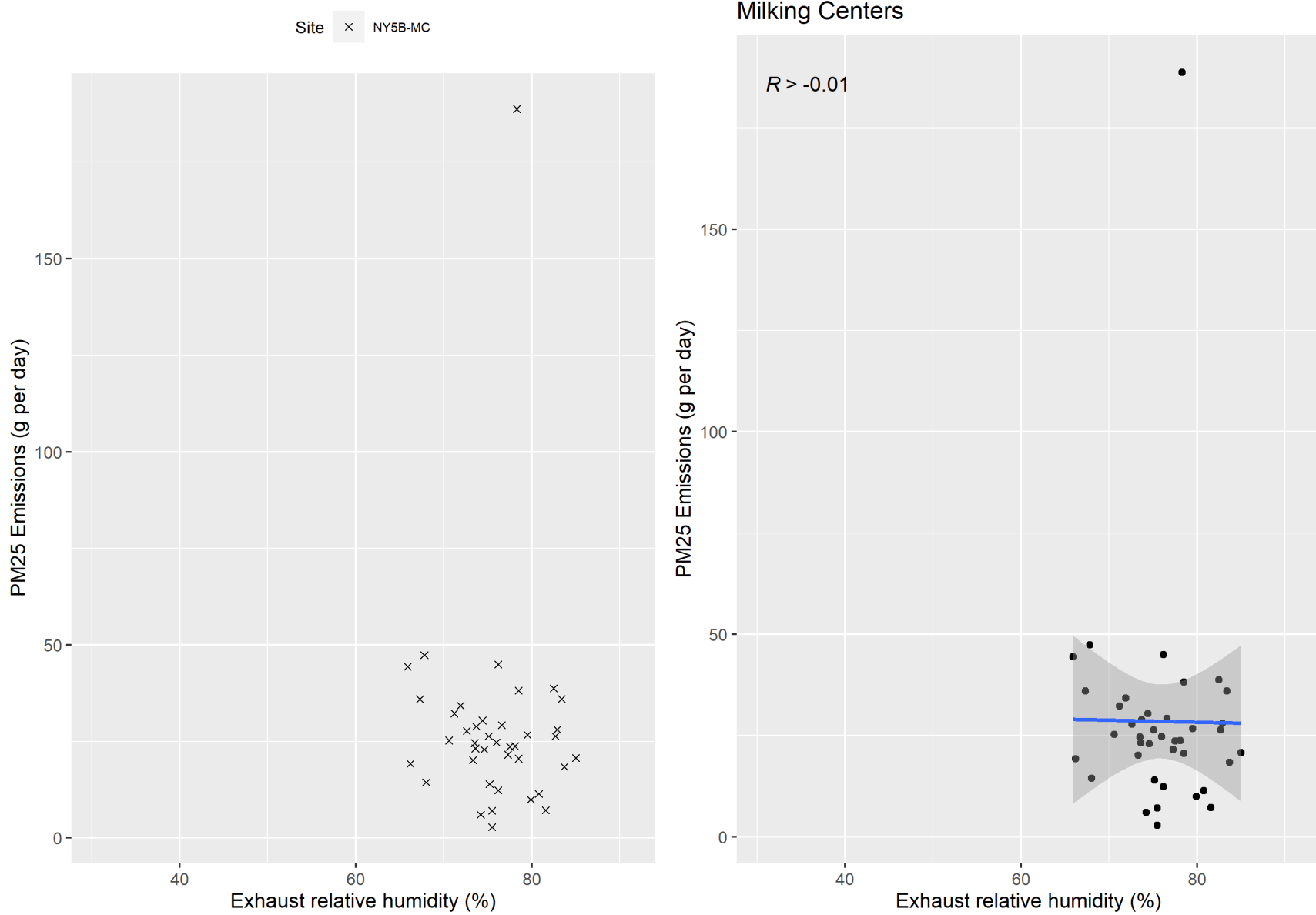
Figure F-64. Scatter plot of milking center PM 2.5 emissions versus exhaust relative humidity and scatter plot with regression.
