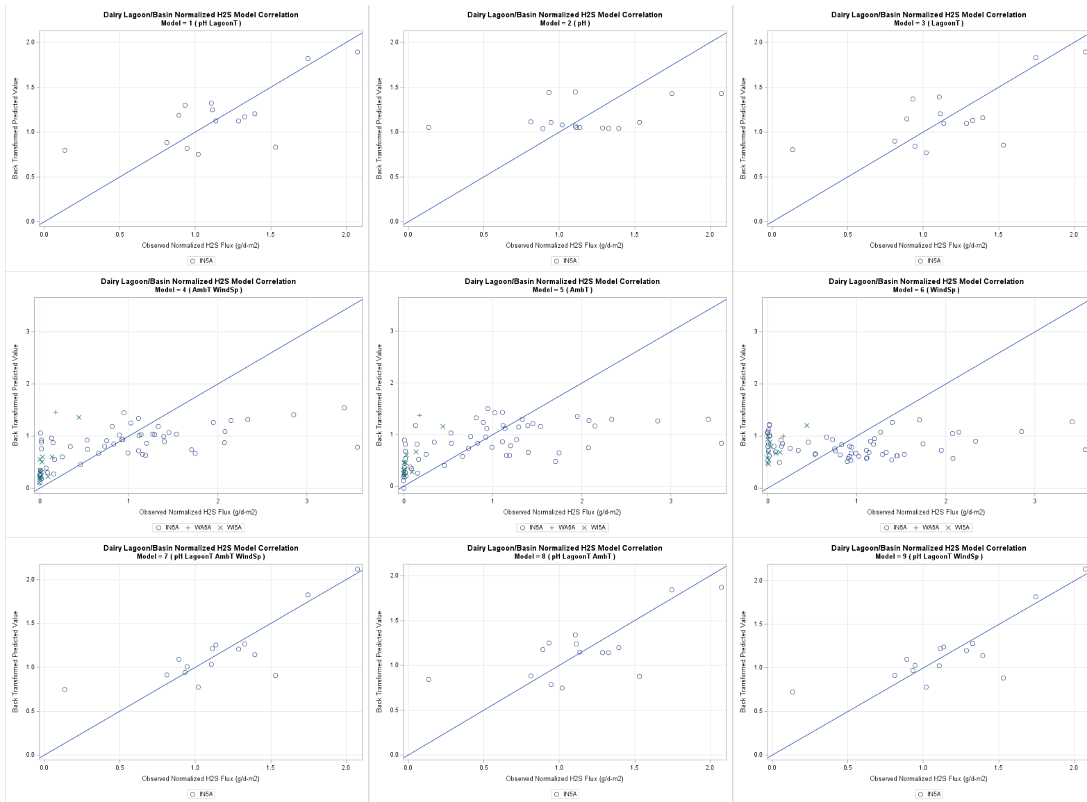
Figure G-73. Dairy lagoon H 2 S one-to-one plots models 1 through 9, back transformed.
