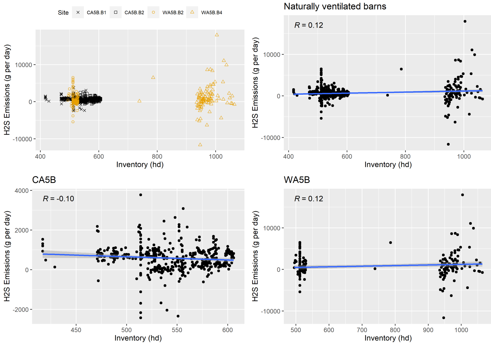
Figure F-82. Scatter plot of naturally ventilated barns H 2 S emissions versus inventory and scatter plot with regression.
