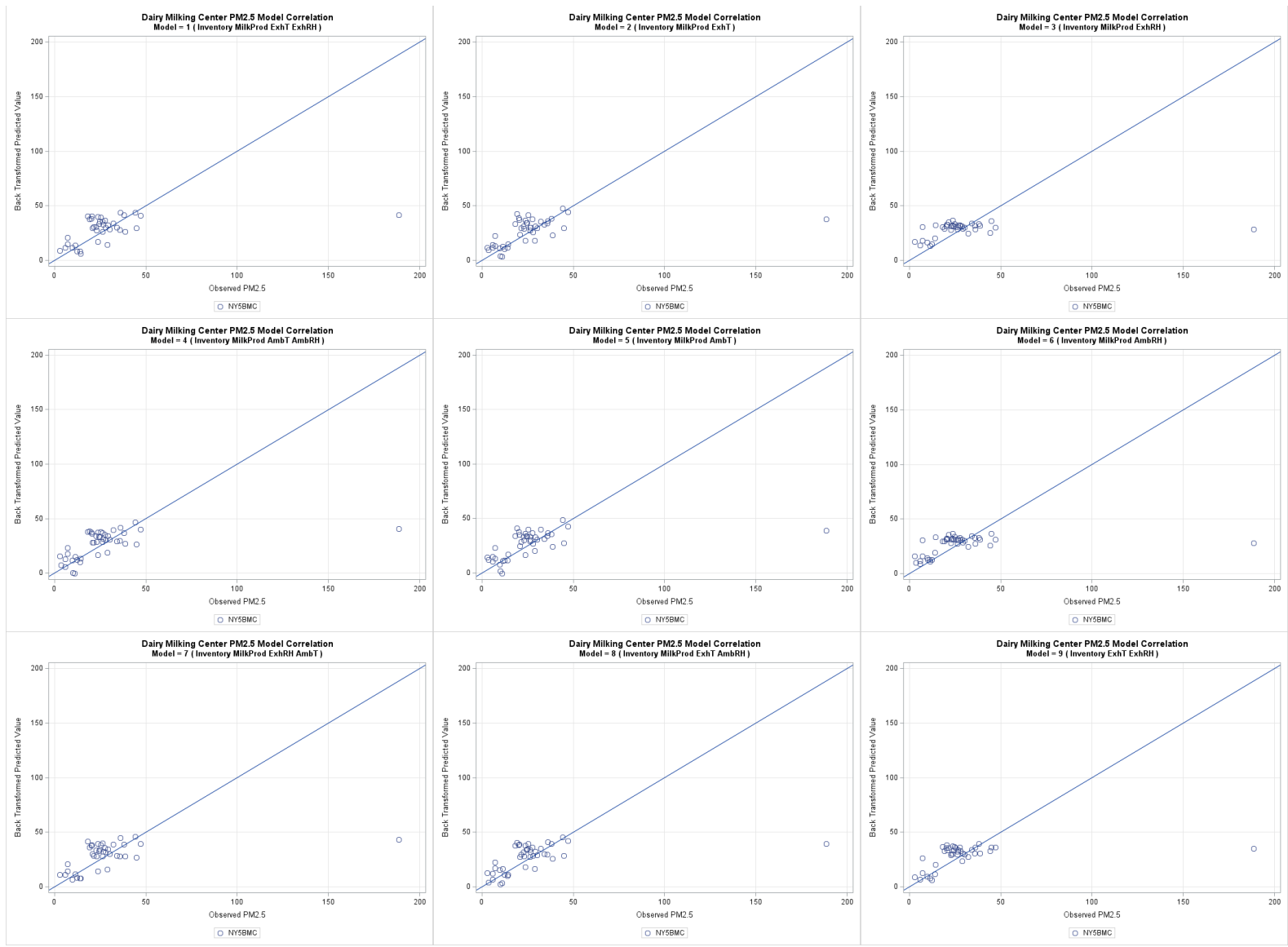
Figure G-45. Dairy milking center PM 2.5 one-to-one plots models 1 through 9, back transformed.
