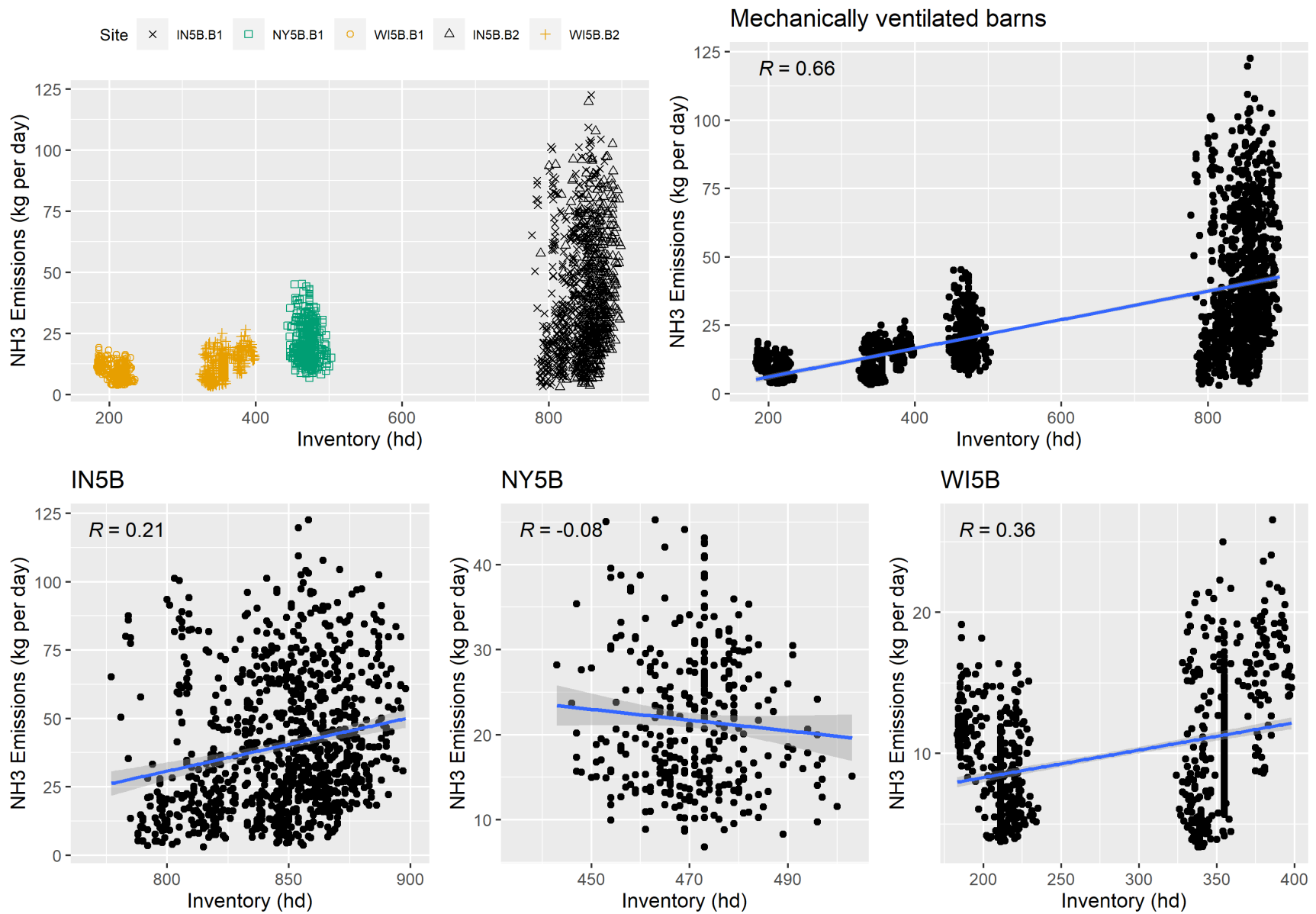
Figure F-1. Scatter plot of mechanically ventilated NH 3 emissions versus inventory and scatter plot with regression.
