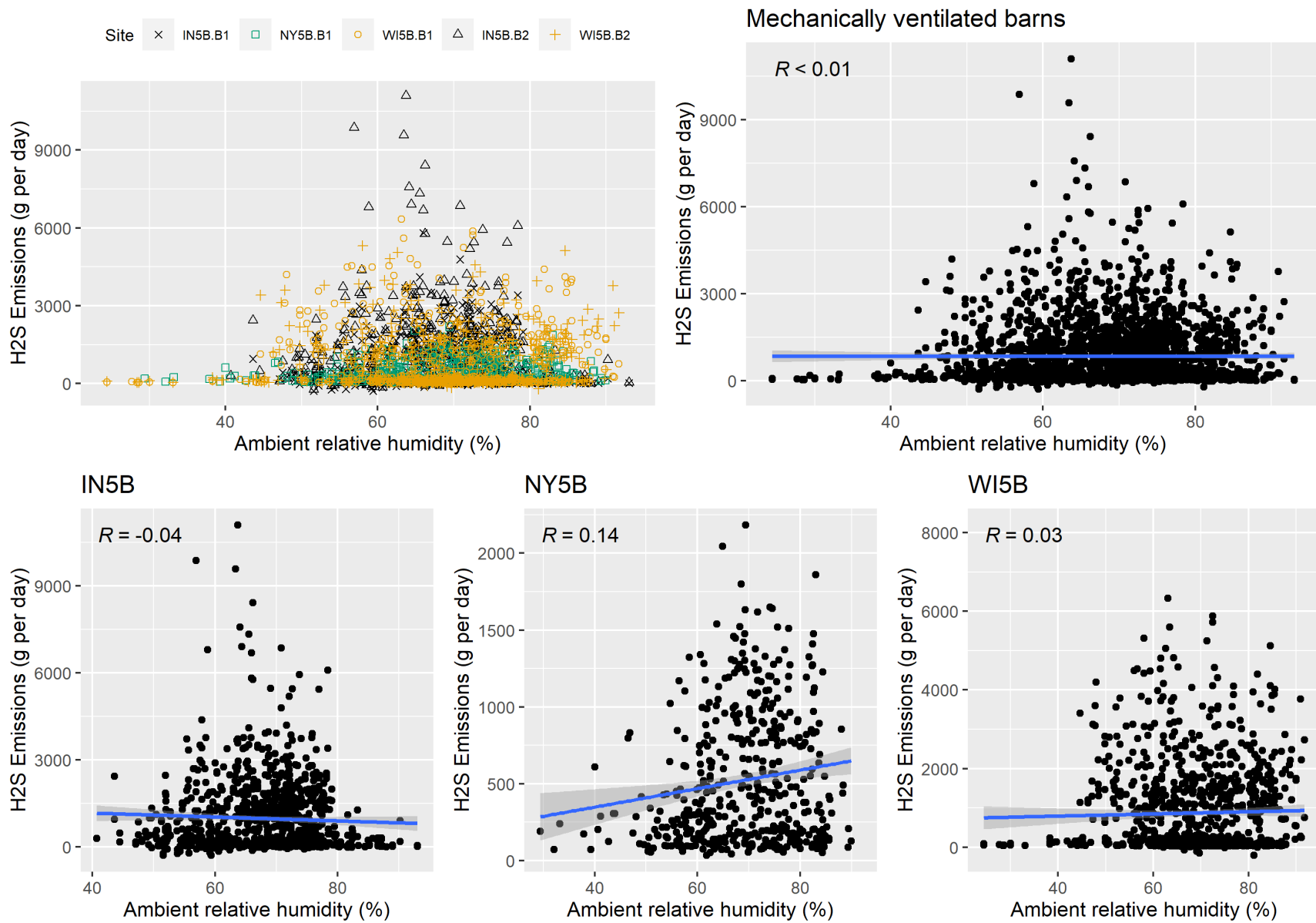
Figure F-37. Scatter plot of mechanically ventilated H 2 S emissions versus ambient relative humidity and scatter plot with regression.
