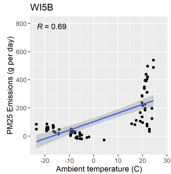
Figure F-34. Scatter plot of mechanically ventilated PM 2.5 emissions versus ambient temperature and scatter plot with regression.
