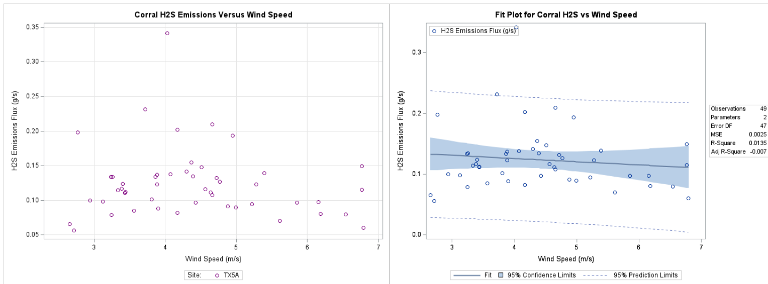
Figure F-141. Scatter plot of corral H 2 S emissions versus wind speed and scatter plot with regression.
