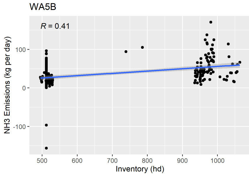
Figure F-81. Scatter plot of naturally ventilated barns NH 3 emissions versus inventory and scatter plot with regression.
