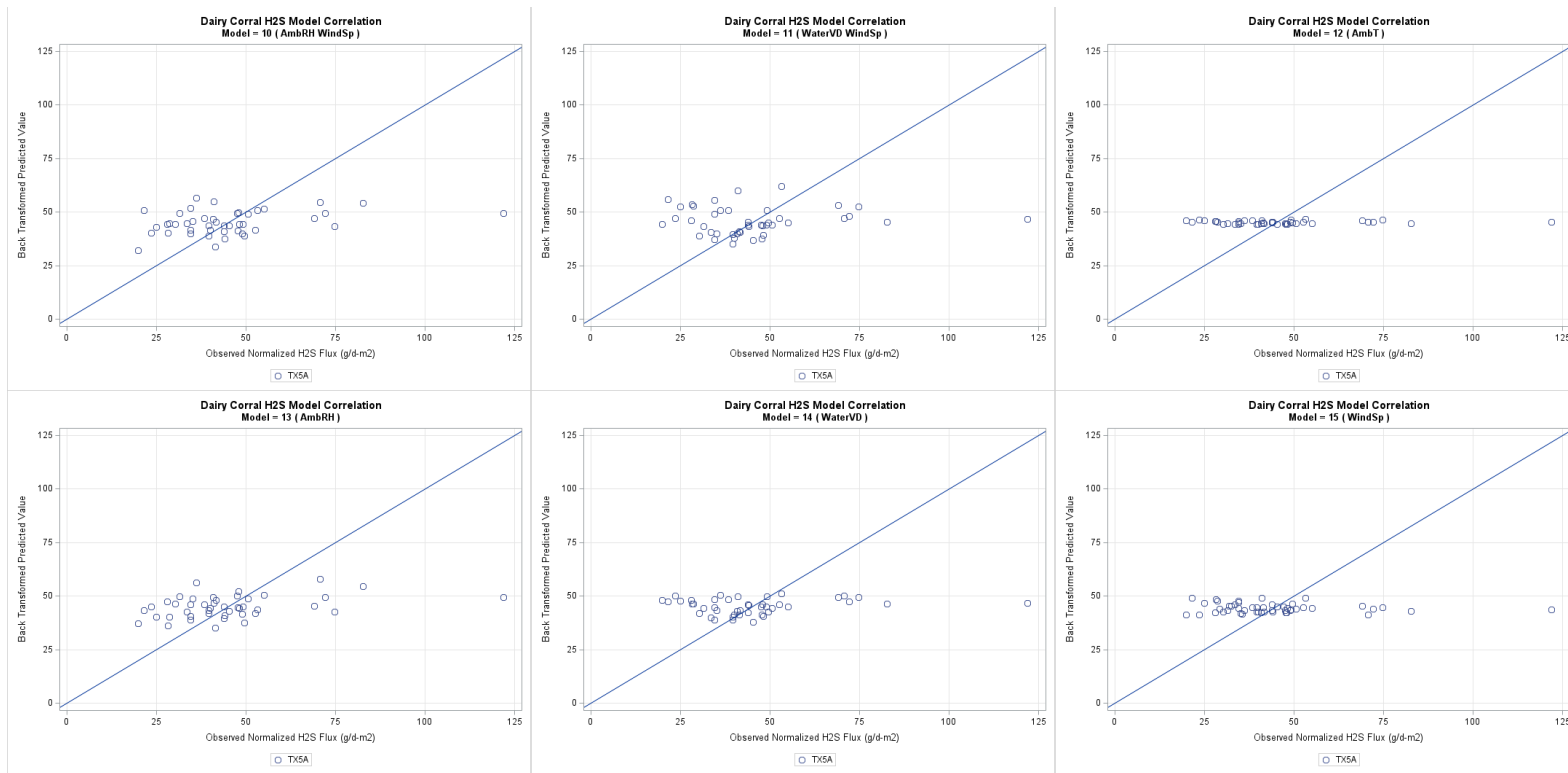
Figure G-88. Dairy corral H 2 S one-to-one plots models 10a through 15a, back transformed.
