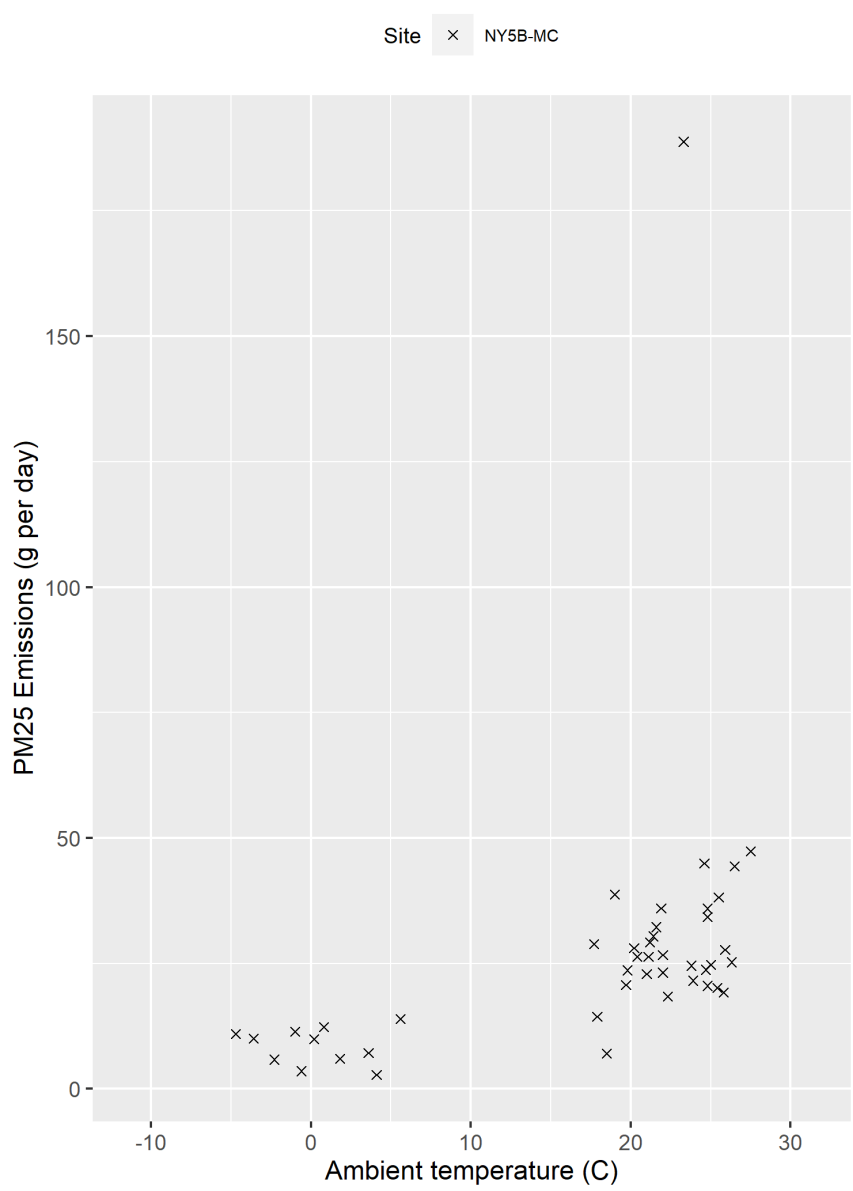
Figure F-74. Scatter plot of milking center PM 2.5 emissions versus ambient temperature and scatter plot with regression.
