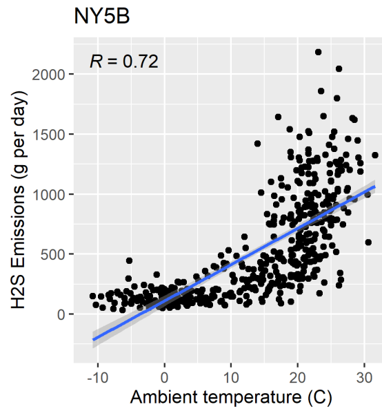
Figure F-32. Scatter plot of mechanically ventilated H 2 S emissions versus ambient temperature and scatter plot with regression.
