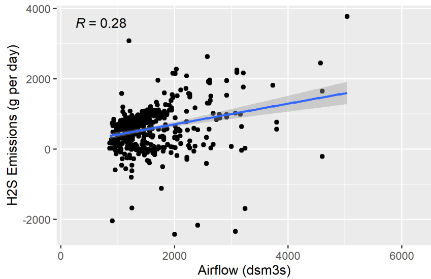
Figure F-107. Scatter plot of naturally ventilated barns H 2 S emissions versus airflow and scatter plot with regression.
