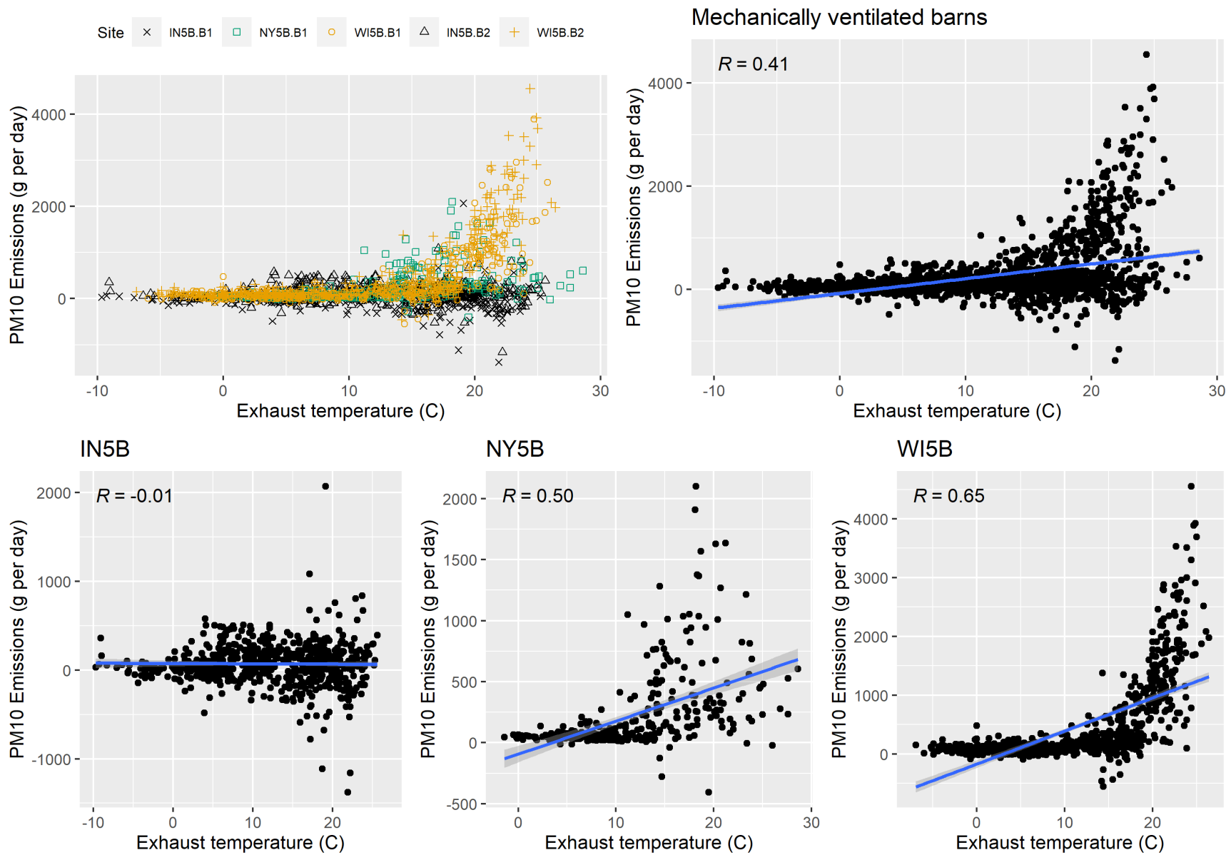
Figure F-18. Scatter plot of mechanically ventilated PM 10 emissions versus exhaust temperature and scatter plot with regression.
