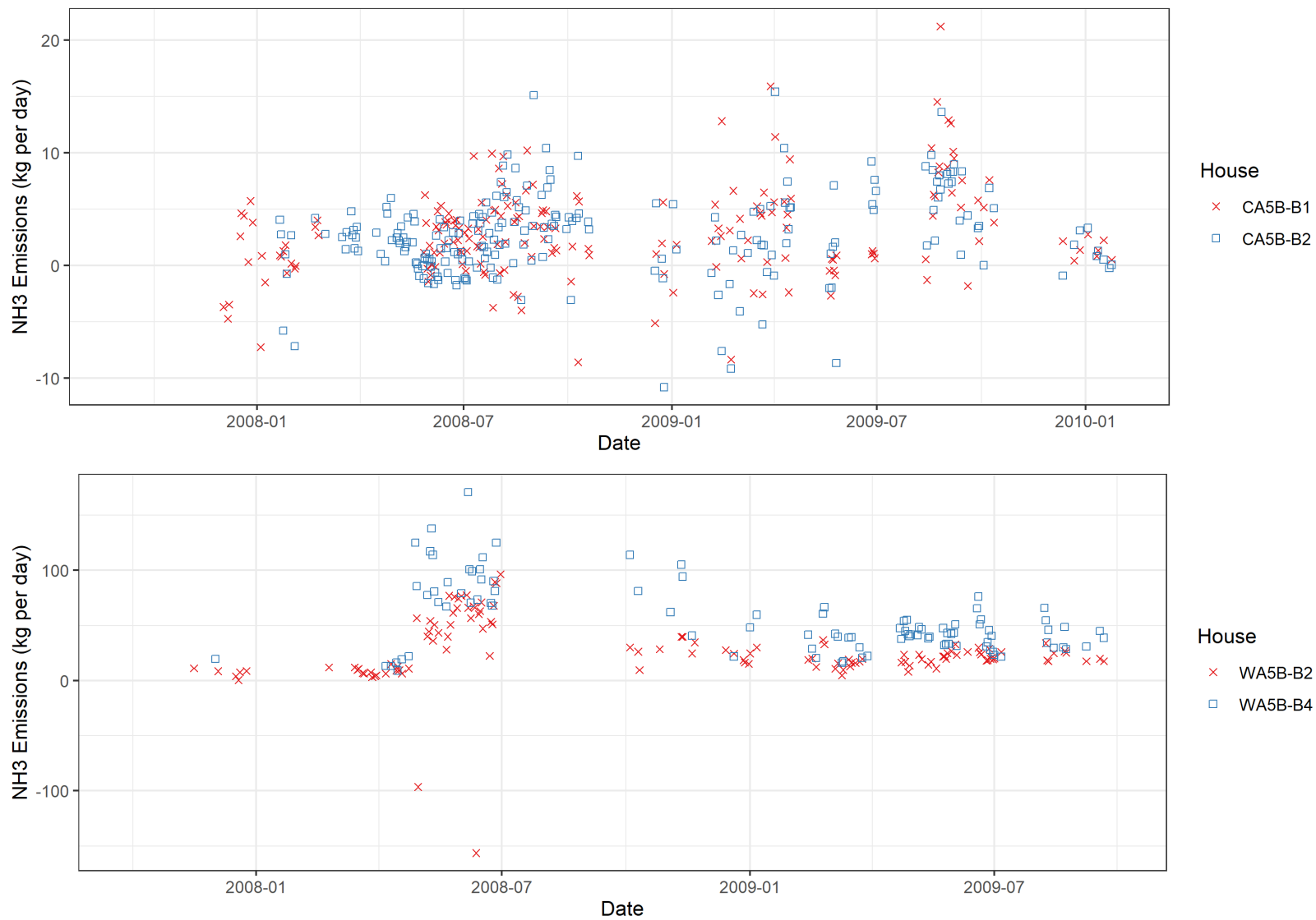
Figure E-29. Trends in NH 3 emissions at naturally ventilated barns, by site, during the NAEMS monitoring period.
