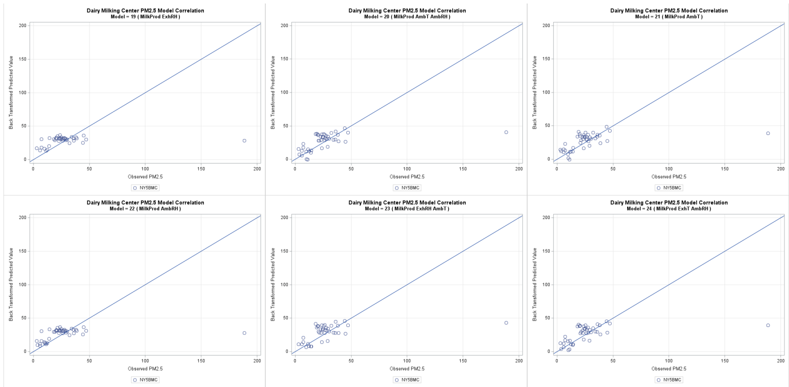
Figure G-47. Dairy milking center PM 2.5 one-to-one plots models 19 through 24, back transformed.
