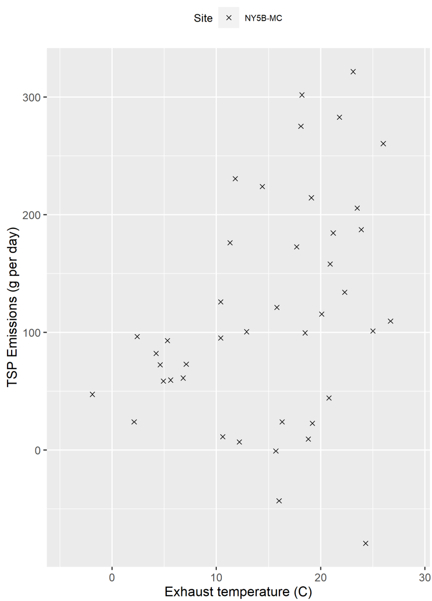
Figure F-60. Scatter plot of milking center TSP emissions versus exhaust temperature and scatter plot with regression.
