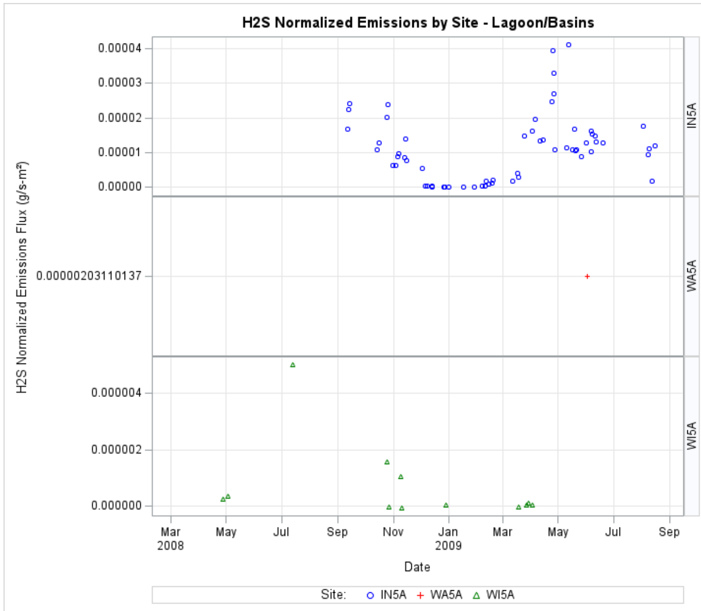
Figure E-46. Trends in H 2 S emissions normalized by surface area, by site, during the NAEMS monitoring period.
