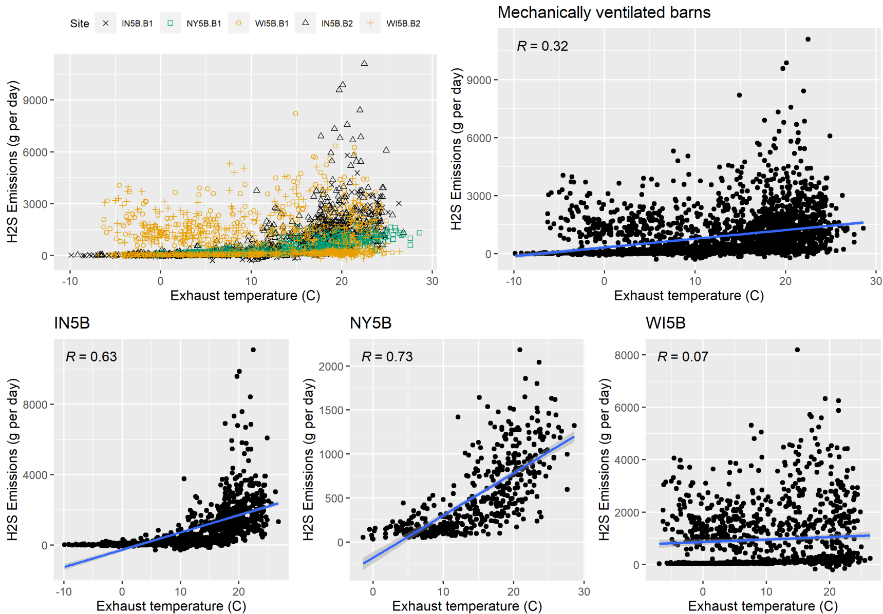
Figure F-17. Scatter plot of mechanically ventilated H 2 S emissions versus exhaust temperature and scatter plot with regression.
