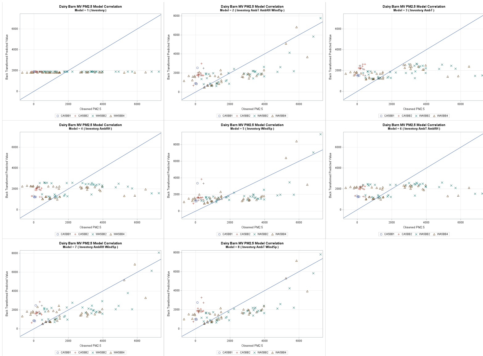
Figure G-64. Dairy naturally ventilated barn PM 2.5 one-to-one plots models 1 through 8, back transformed.
