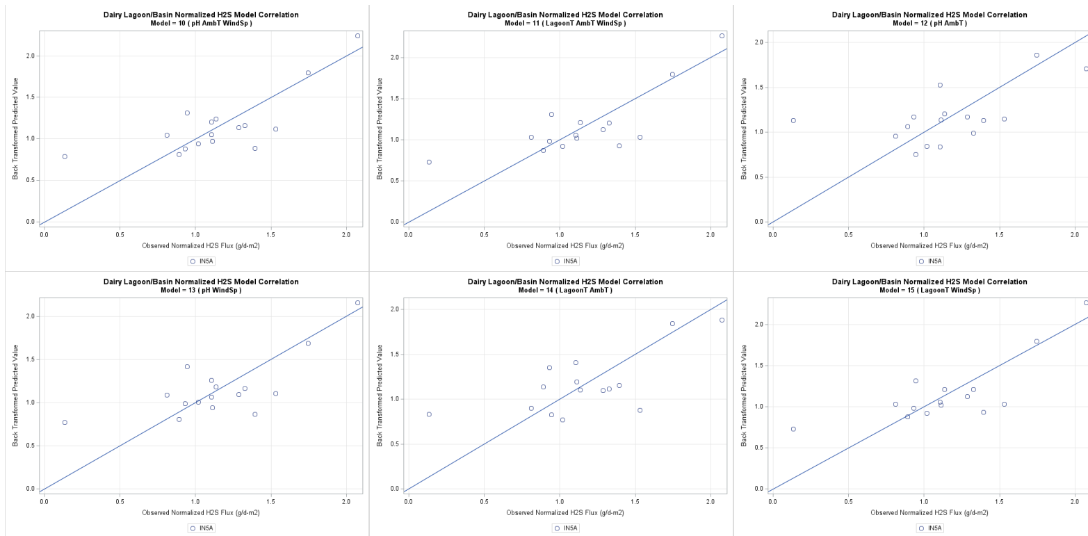
Figure G-74. Dairy lagoon H 2 S one-to-one plots models 10 through 15, back transformed.
