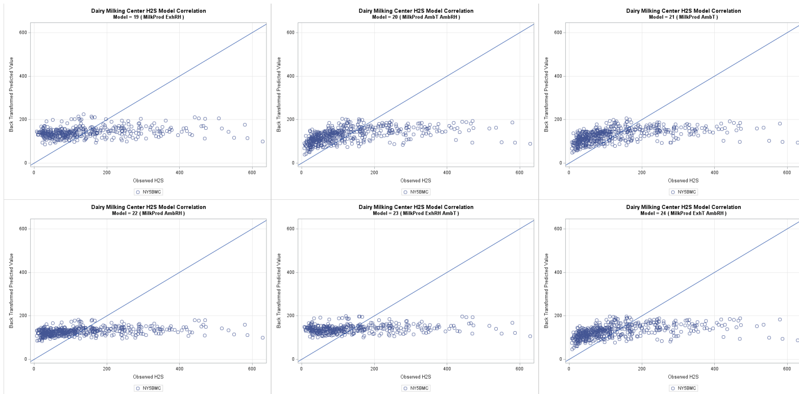
Figure G-31. Dairy milking center H 2 S one-to-one plots models 19 through 24, back transformed.
