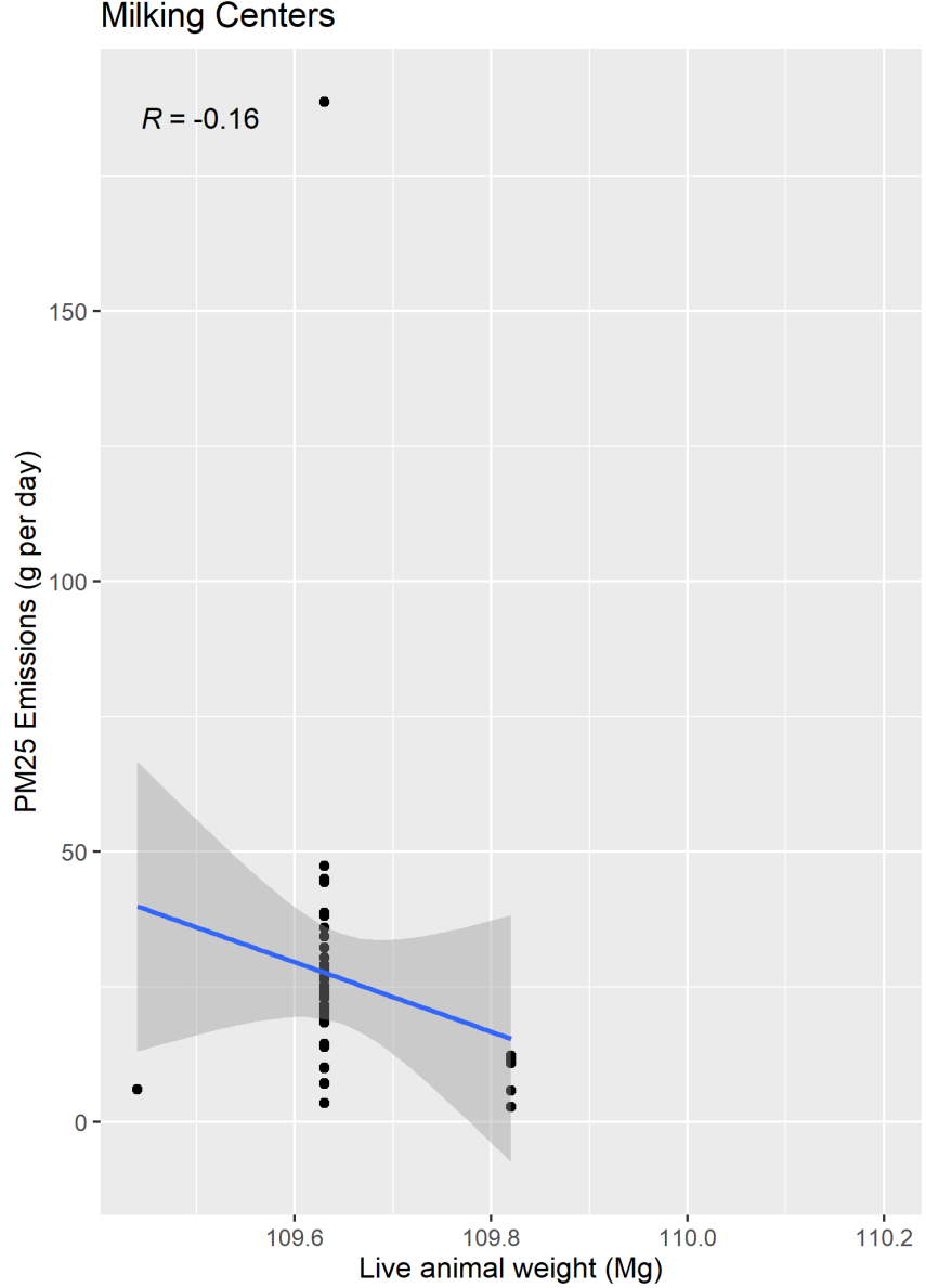
Figure F-54. Scatter plot of milking center PM 2.5 emissions versus live animal weight and scatter plot with regression.
