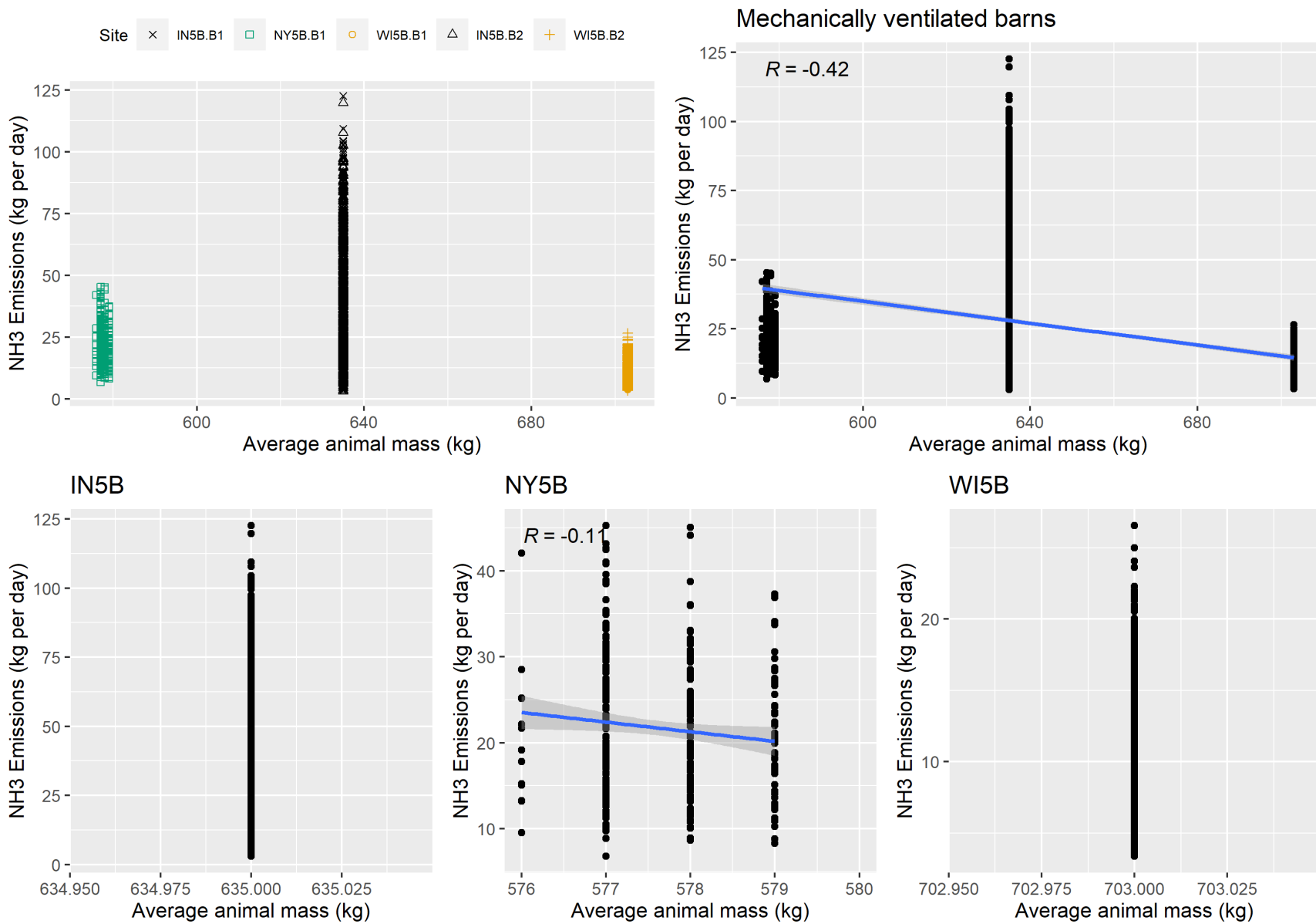
Figure F-6. Scatter plot of mechanically ventilated NH 3 emissions versus average animal mass and scatter plot with regression.
