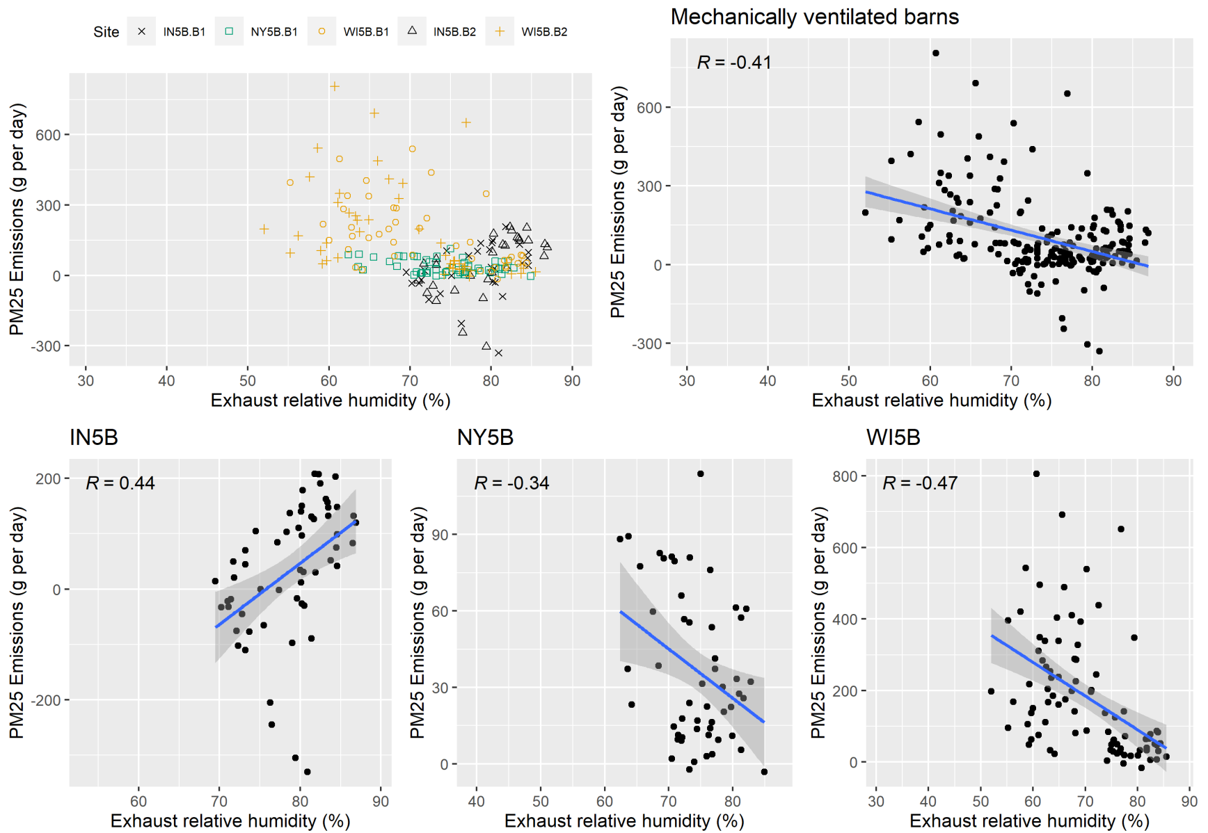
Figure F-24. Scatter plot of mechanically ventilated PM2.5 emissions versus exhaust relative humidity and scatter plot with regression.
