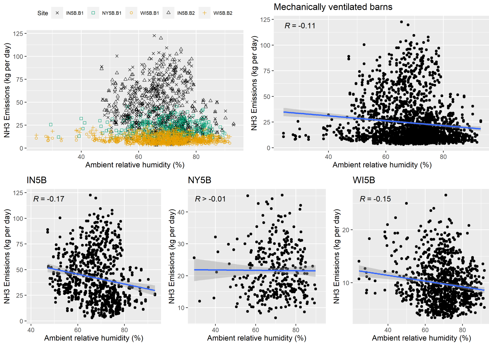
Figure F-36. Scatter plot of mechanically ventilated NH 3 emissions versus ambient relative humidity and scatter plot with regression.
