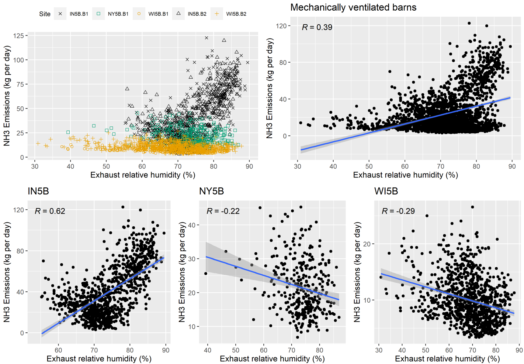
Figure F-21. Scatter plot of mechanically ventilated NH 3 emissions versus exhaust relative humidity and scatter plot with regression.
