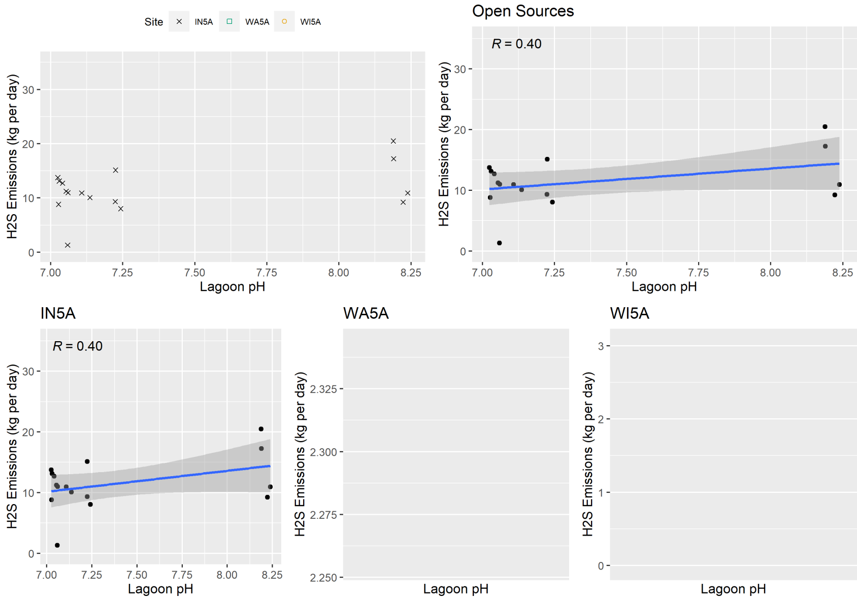
Figure F-129. Scatter plot of lagoon/basin H 2 S emissions versus lagoon pH and scatter plot with regression.
