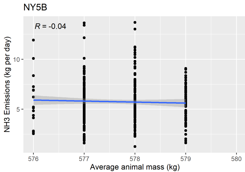
Figure F-46. Scatter plot of milking center NH 3 emissions versus average animal mass and scatter plot with regression.
