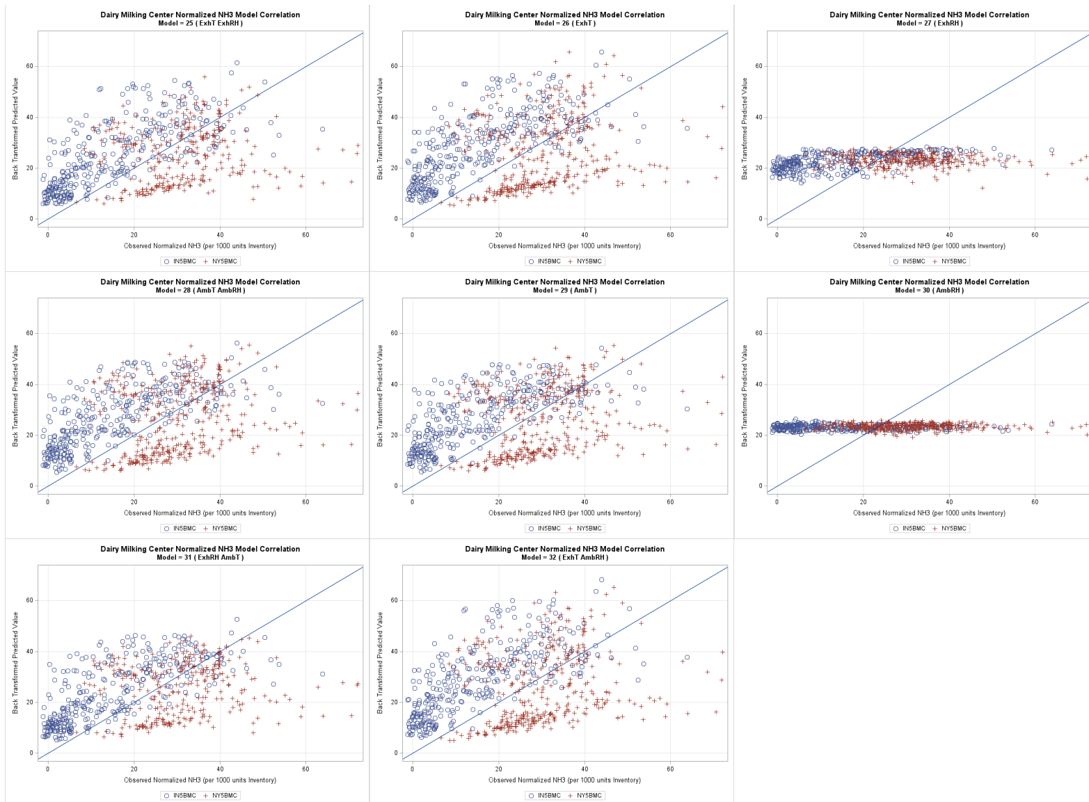
Figure G-24 Dairy milking center NH 3 one-to-one plots models 25 through 32, back transformed.
