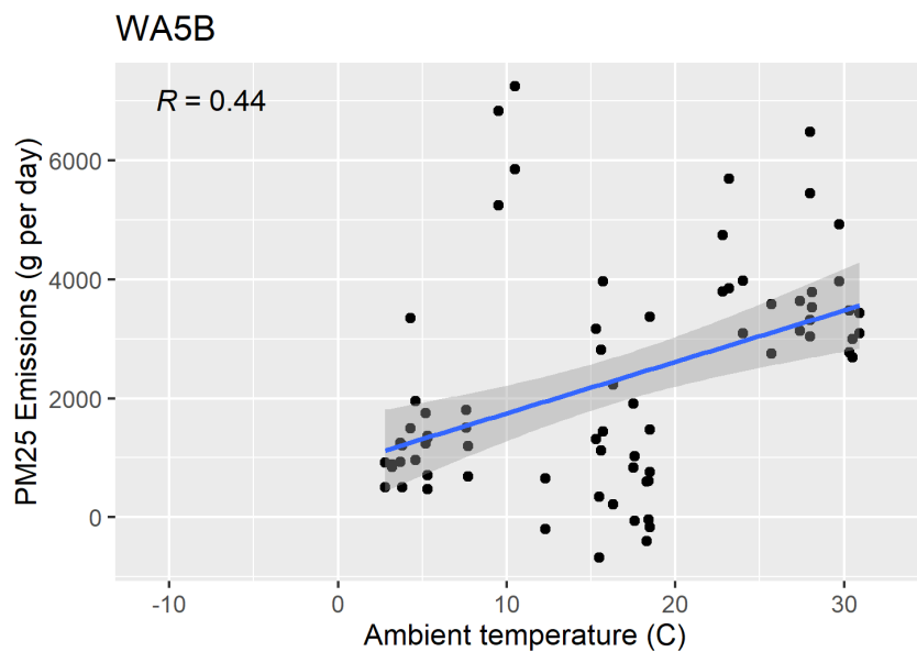
Figure F-114. Scatter plot of naturally ventilated barns PM 2.5 emissions versus ambient temperature and scatter plot with regression.
