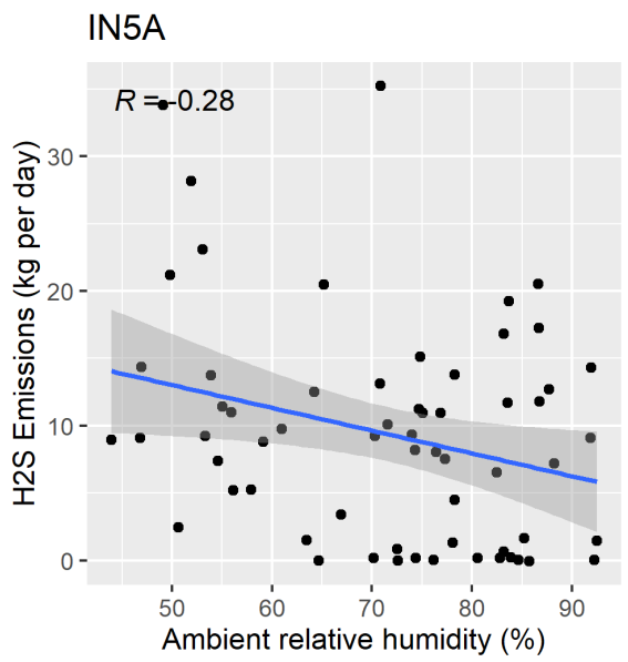
Figure F-133. Scatter plot of lagoon/basin H 2 S emissions versus ambient relative humidity and scatter plot with regression.
