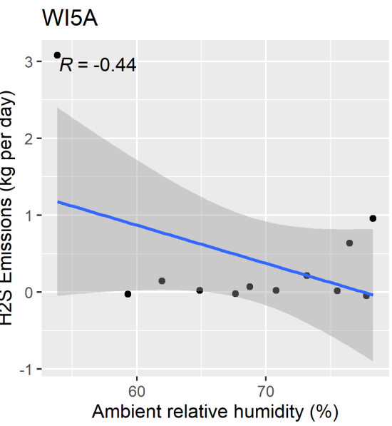
Figure F-133. Scatter plot of lagoon/basin H 2 S emissions versus ambient relative humidity and scatter plot with regression.
