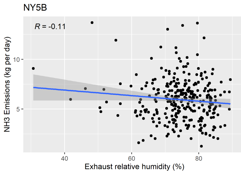
Figure F-61. Scatter plot of milking center NH 3 emissions versus exhaust relative humidity and scatter plot with regression.
