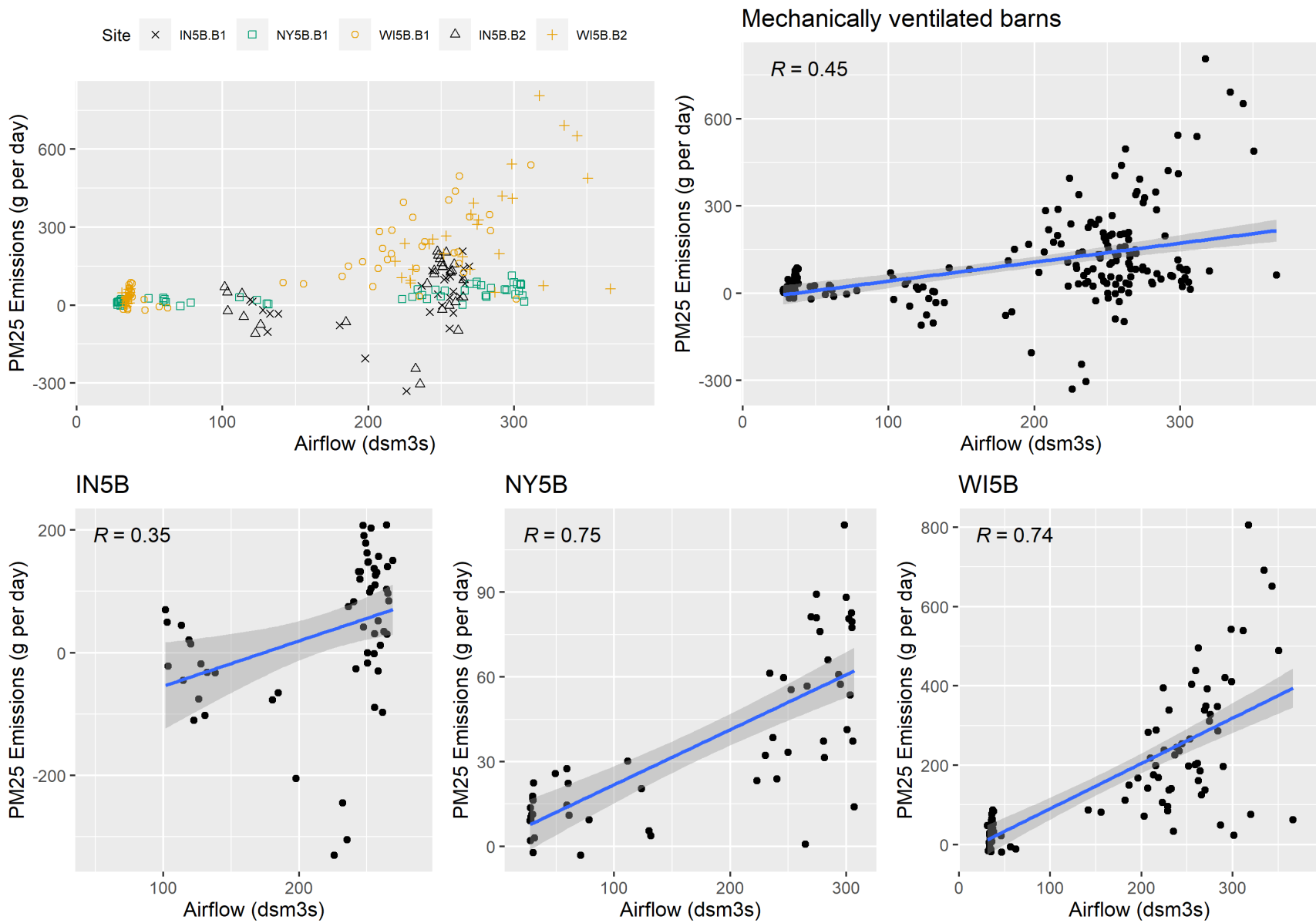
Figure F-29. Scatter plot of mechanically ventilated PM2.5 emissions versus airflow and scatter plot with regression.
