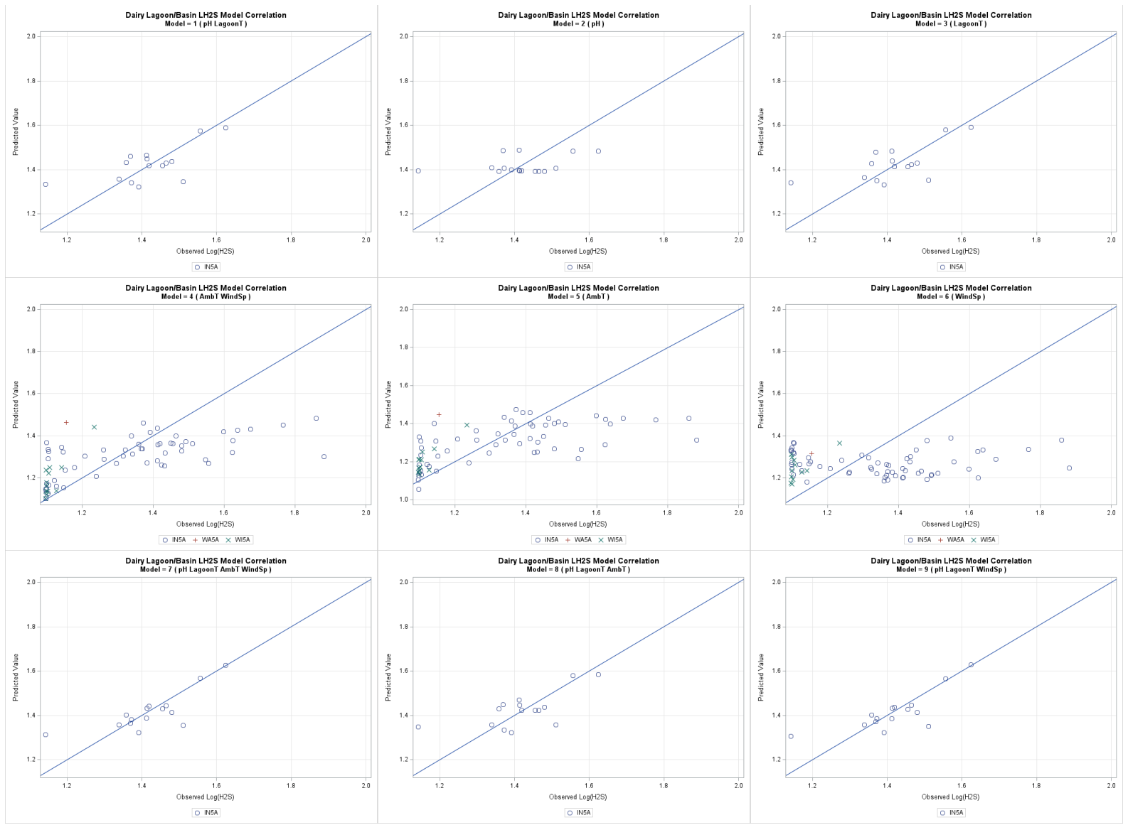
Figure G-71. Dairy lagoon H 2 S one-to-one plots models 1 through 9, log transformed.
