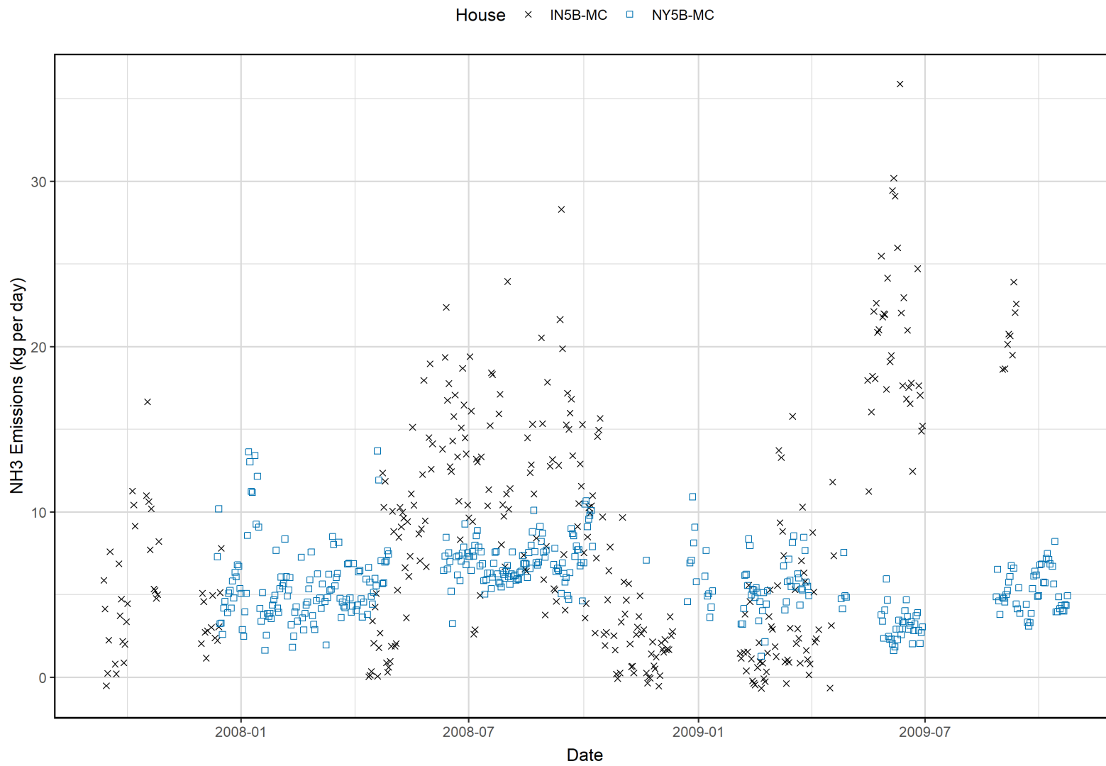
Figure E-14. NAEMS milking center NH 3 emission trends, by site.
