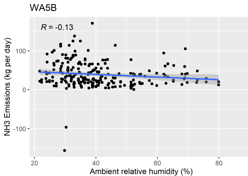
Figure F-116. Scatter plot of naturally ventilated barns NH 3 emissions versus ambient relative humidity and scatter plot with regression.
