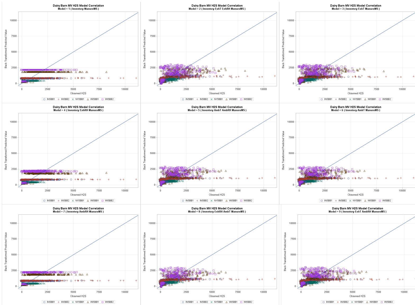
Figure G-4. Dairy mechanically ventilated barn H 2 S one-to-one plots models 1 through 9, back transformed.
