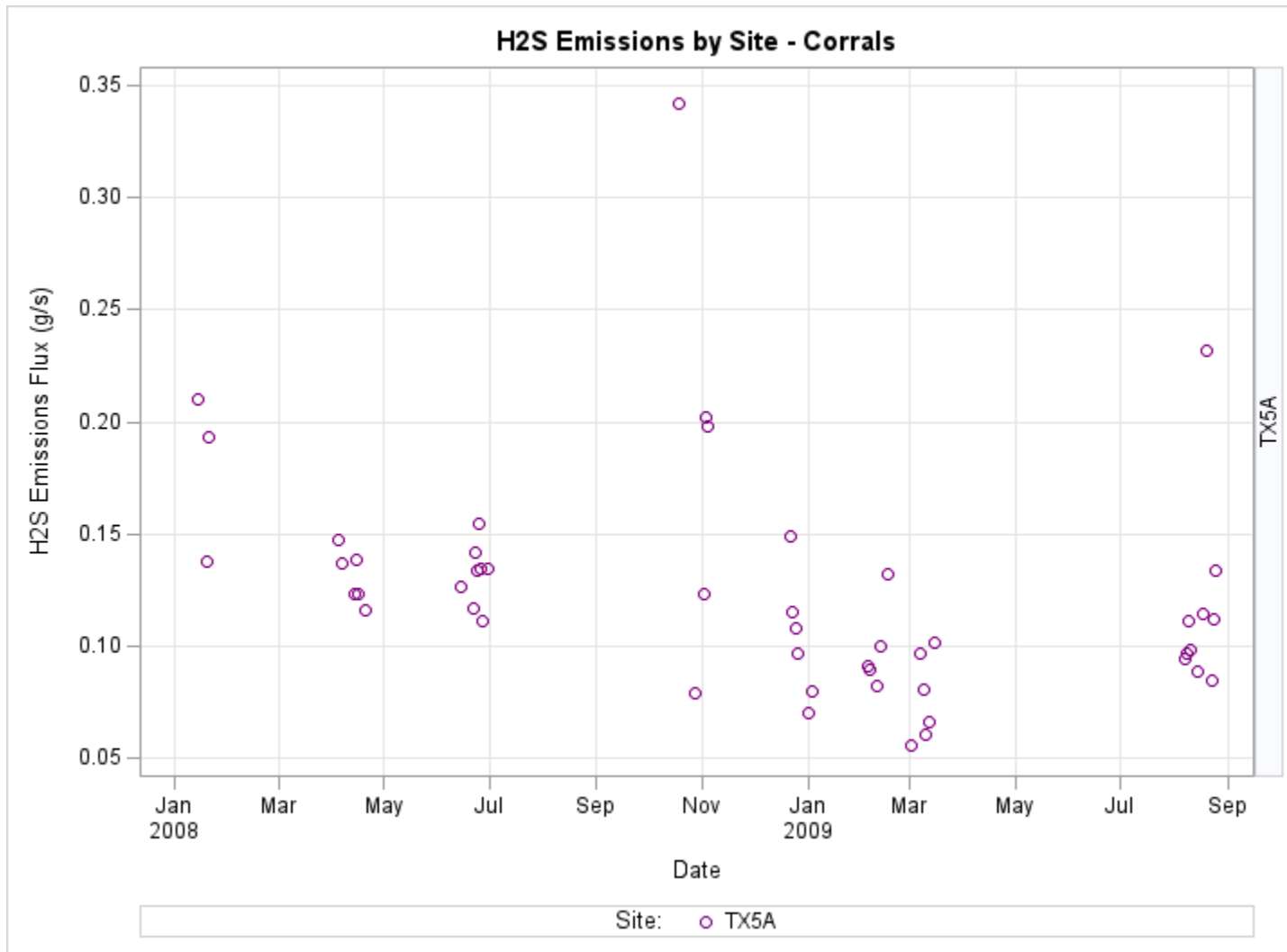
Figure E-53. Trends in corral H 2 S emissions, during the NAEMS monitoring period.
