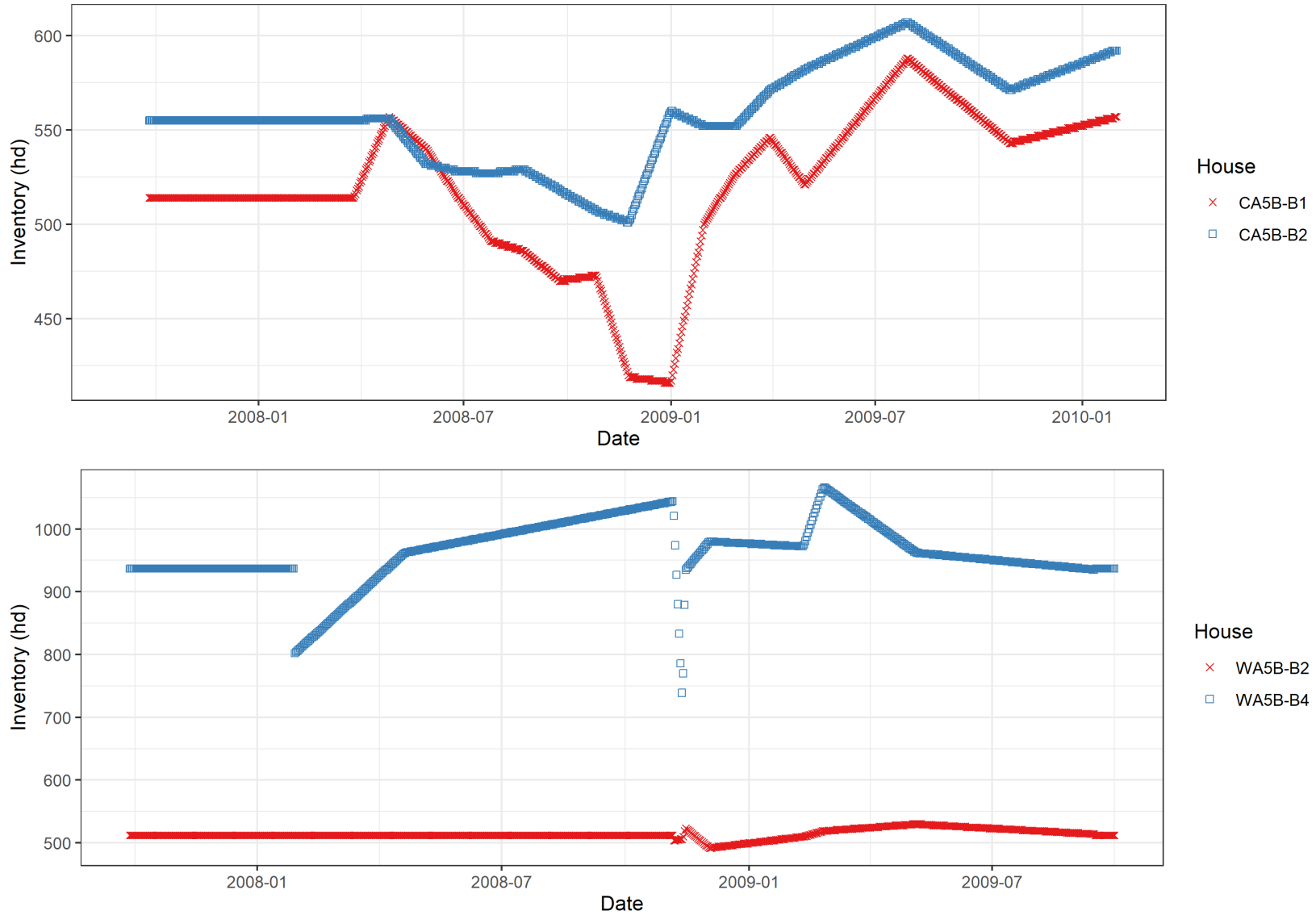
Figure E-34. Trends in Inventory at naturally ventilated barns, by site, during the NAEMS monitoring period.
