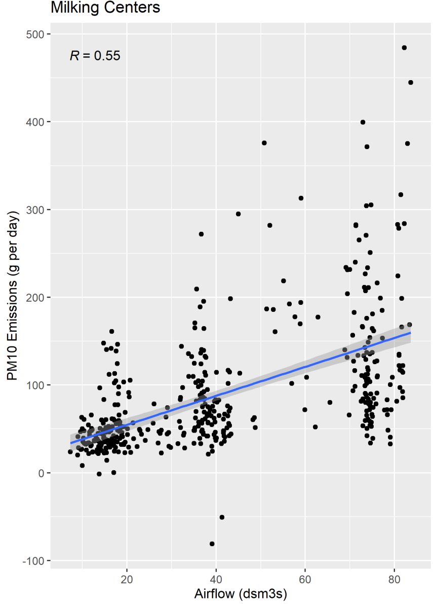
Figure F-68. Scatter plot of milking center PM 10 emissions versus airflow and scatter plot with regression.
