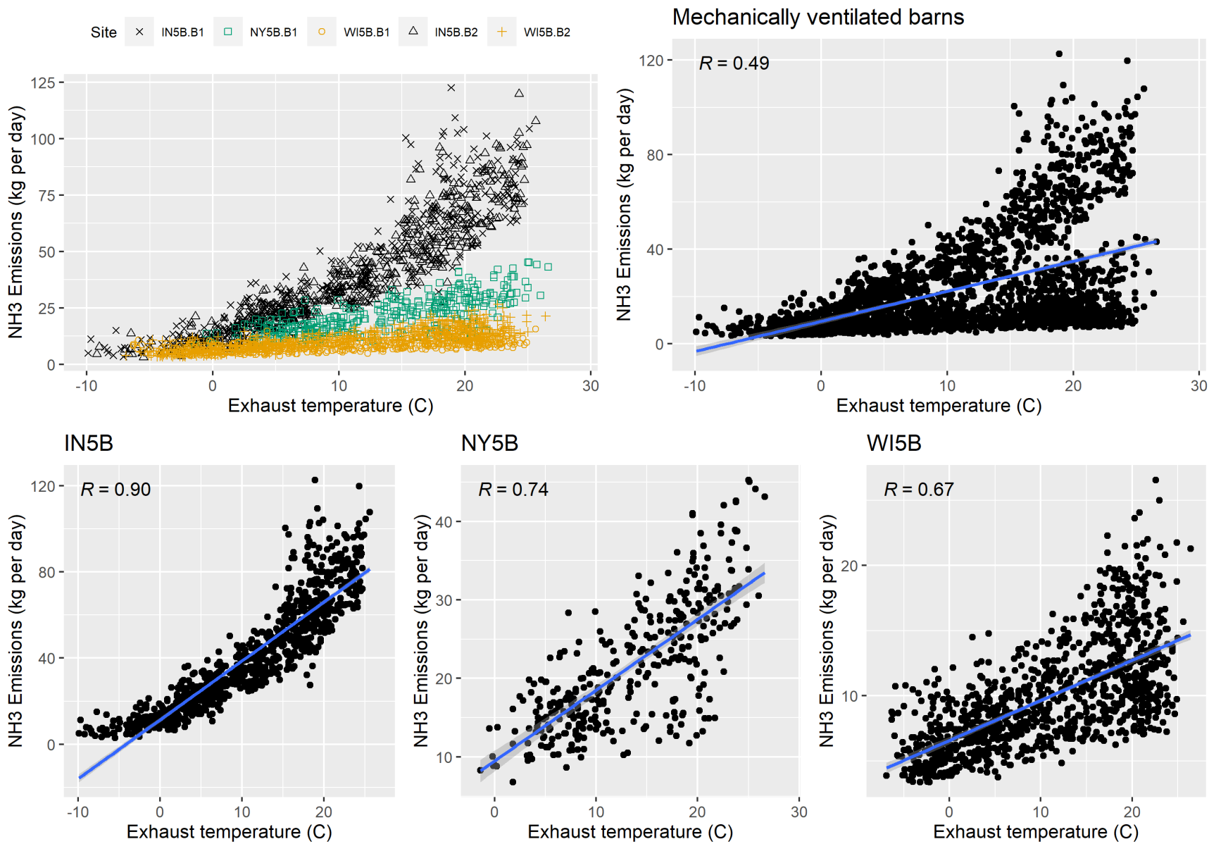
Figure F-16. Scatter plot of mechanically ventilated NH 3 emissions versus exhaust temperature and scatter plot with regression.
