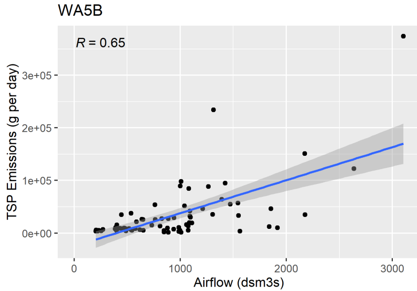
Figure F-110. Scatter plot of naturally ventilated barns TSP emissions versus airflow and scatter plot with regression.
