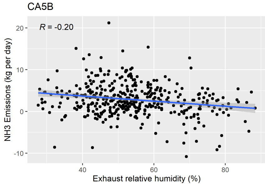
Figure F-101. Scatter plot of naturally ventilated barns NH 3 emissions versus exhaust relative humidity and scatter plot with regression.
