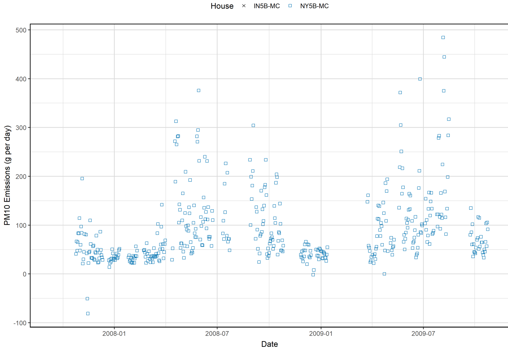
Figure E-16. NAEMS milking center PM 10 emission trends, by site.
