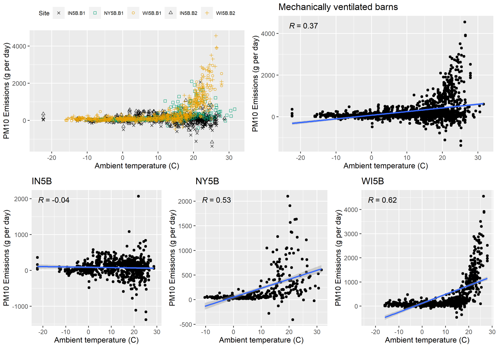
Figure F-33. Scatter plot of mechanically ventilated PM 10 emissions versus ambient temperature and scatter plot with regression.
