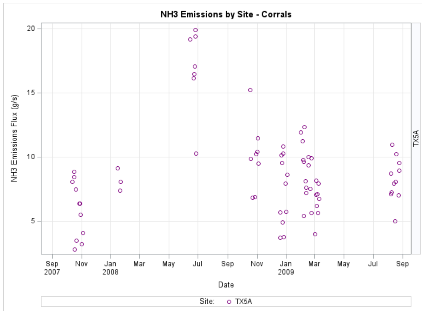
Figure E-52. Trends in corral NH 3 emissions, during the NAEMS monitoring period.
