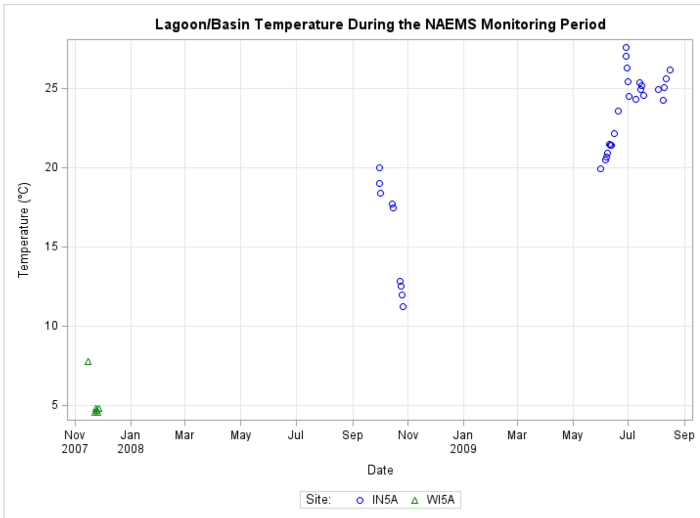
Figure E-47. Trends in lagoon/basin temperature, by open source site, during the NAEMS monitoring period.
