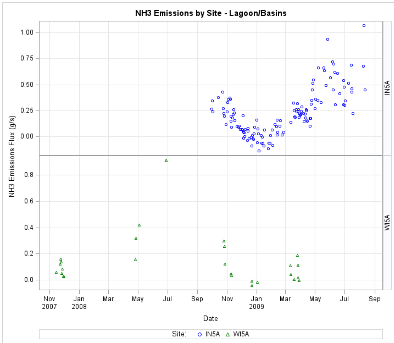
Figure E-43. Trends in NH 3 emissions at dairy lagoons, by site, during the NAEMS monitoring period.
