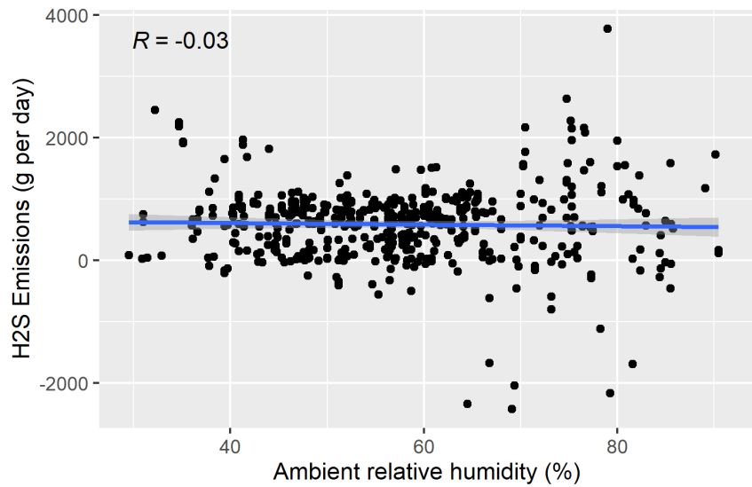
Figure F-117. Scatter plot of naturally ventilated barns H 2 S emissions versus ambient relative humidity and scatter plot with regression.
