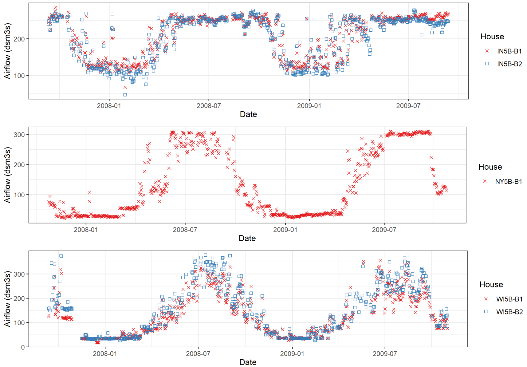
Figure E-11. Trends in airflow at mechanically ventilated barns, by site, during the NAEMS monitoring period.
