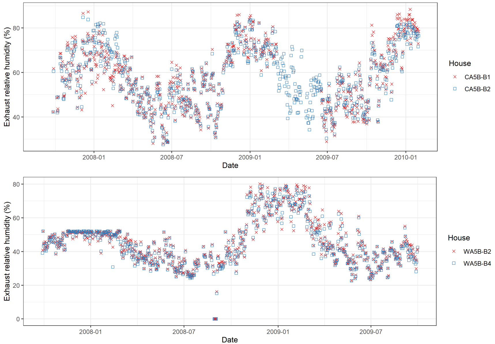
Figure E-38. Trends in exhaust relative humidity at naturally ventilated barns, by site, during the NAEMS monitoring period.
