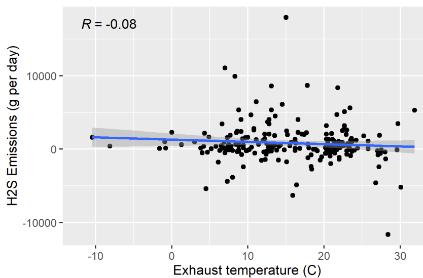
Figure F-97. Scatter plot of naturally ventilated barns H 2 S emissions versus exhaust temperature and scatter plot with regression.
