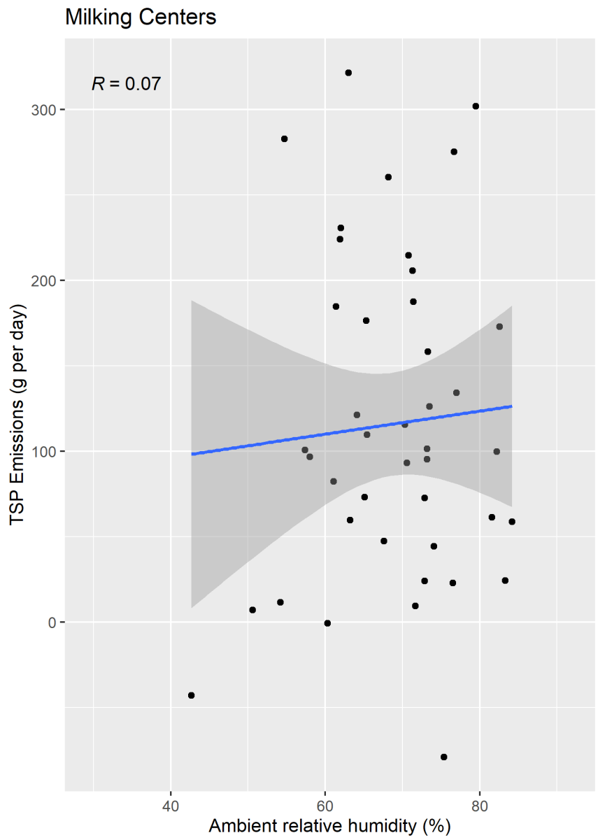
Figure F-80. Scatter plot of milking center TSP emissions versus ambient relative humidity and scatter plot with regression.
