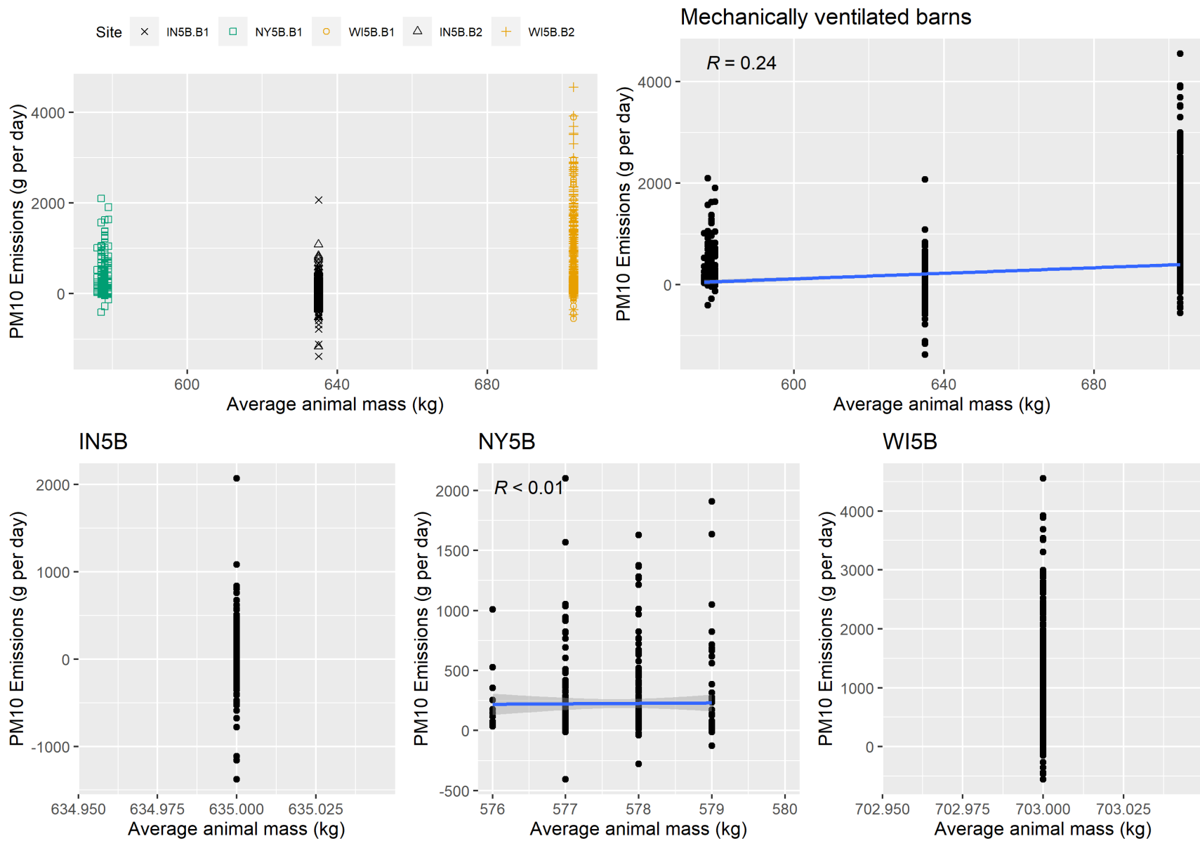
Figure F-8. Scatter plot of mechanically ventilated PM 10 emissions versus average animal mass and scatter plot with regression.
