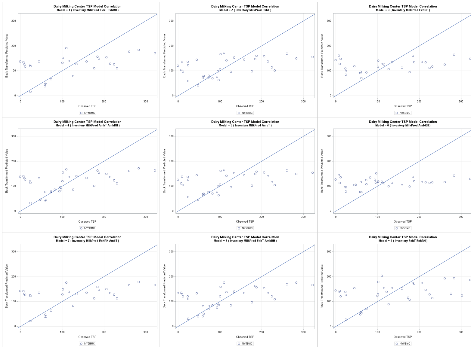
Figure G-53. Dairy milking center TSP one-to-one plots models 1 through 9, back transformed.
