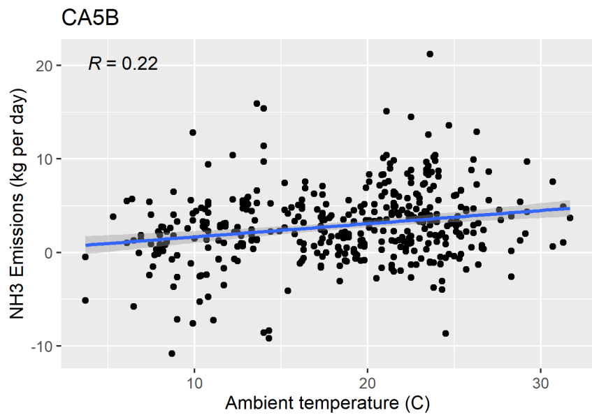
Figure F-111. Scatter plot of naturally ventilated barns NH 3 emissions versus ambient temperature and scatter plot with regression.
