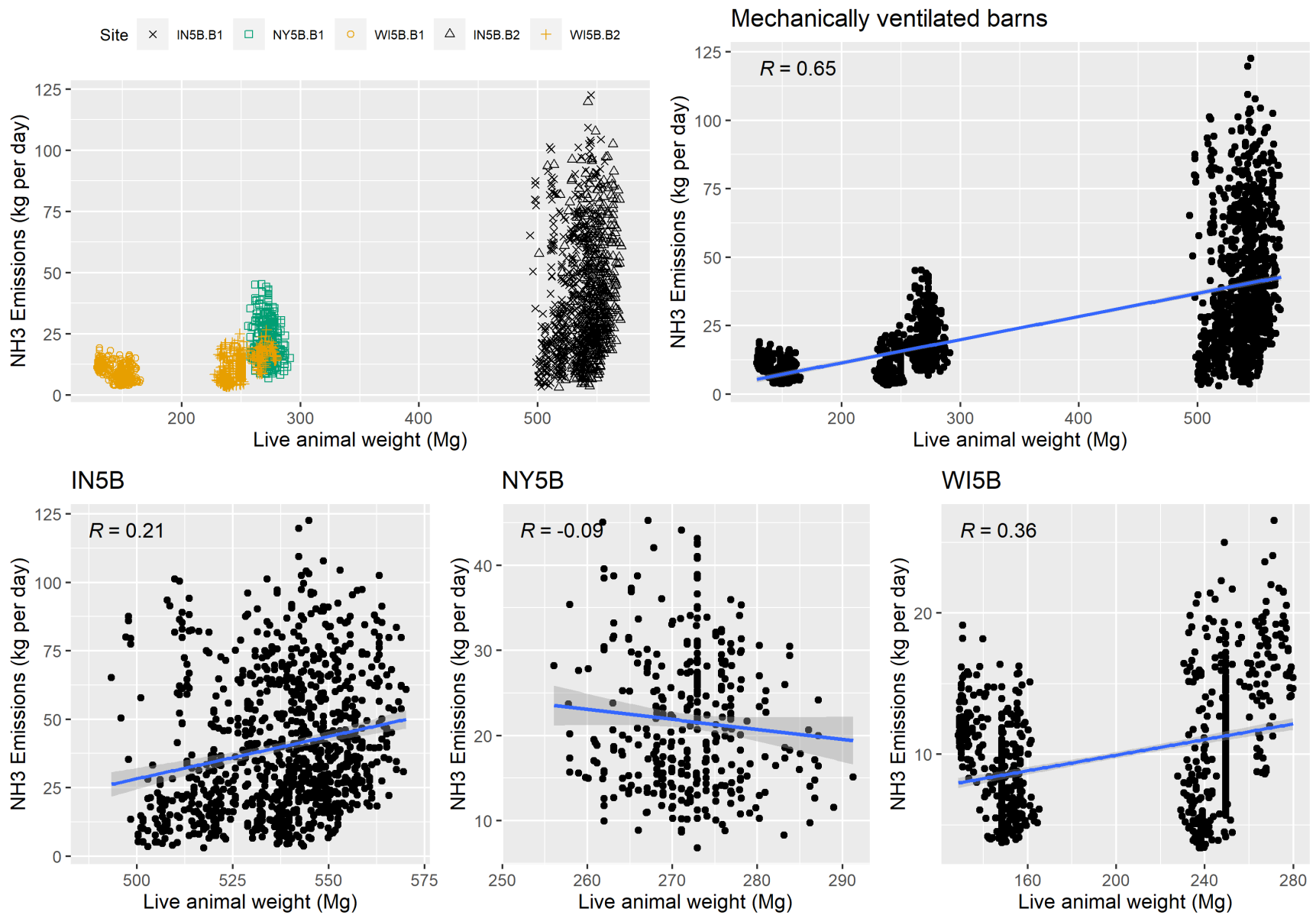
Figure F-11. Scatter plot of mechanically ventilated NH 3 emissions versus live animal weight and scatter plot with regression.
