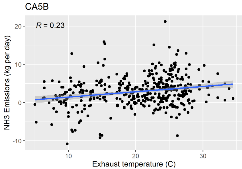
Figure F-96. Scatter plot of naturally ventilated barns NH 3 emissions versus exhaust temperature and scatter plot with regression.
