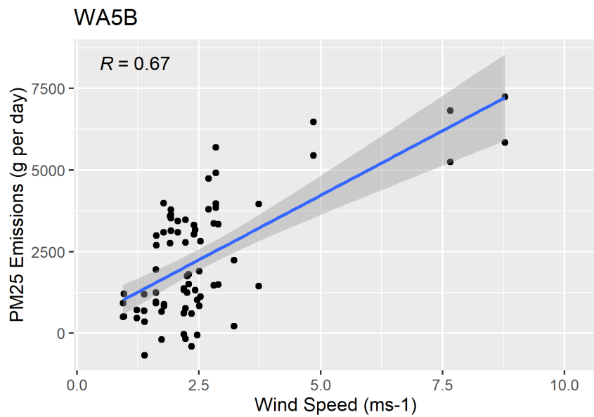
Figure F-124. Scatter plot of naturally ventilated barns PM 2.5 emissions versus wind speed and scatter plot with regression.
