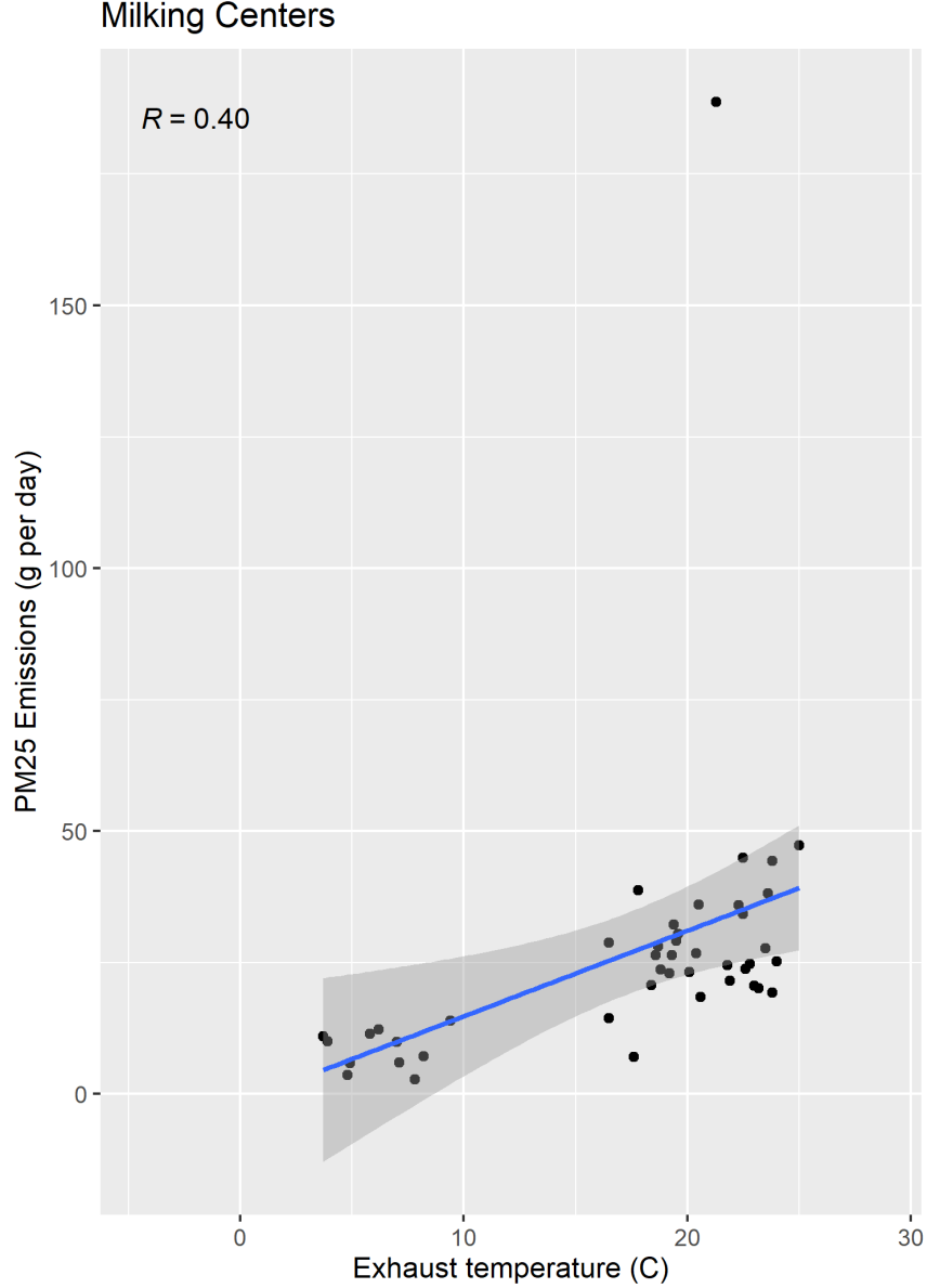
Figure F-59. Scatter plot of milking center PM 2.5 emissions versus exhaust temperature and scatter plot with regression.
