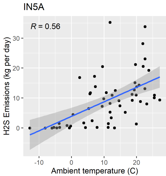
Figure F-131. Scatter plot of lagoon/basin H 2 S emissions versus ambient temperature and scatter plot with regression.
