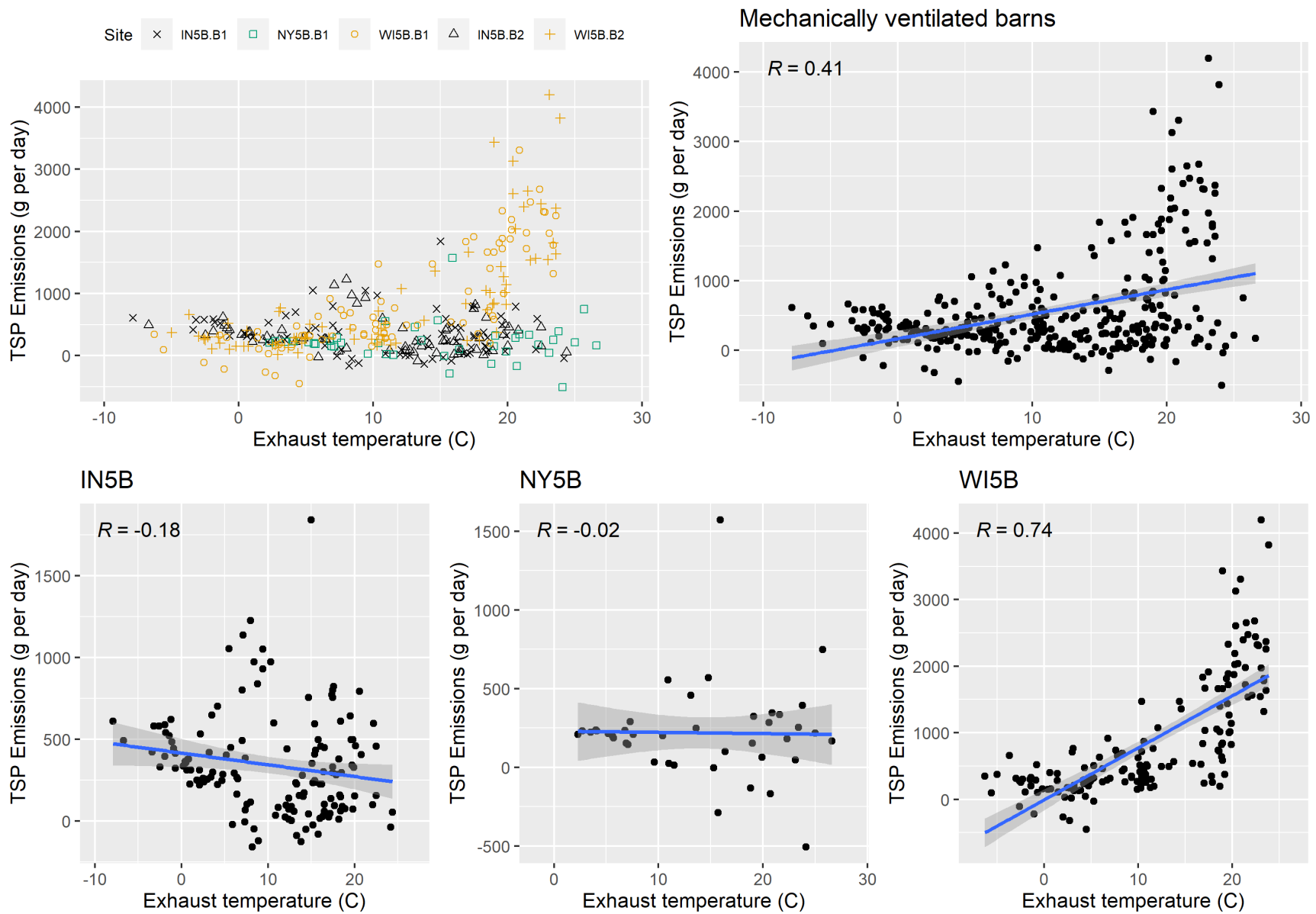
Figure F-20. Scatter plot of mechanically ventilated TSP emissions versus exhaust temperature and scatter plot with regression.
