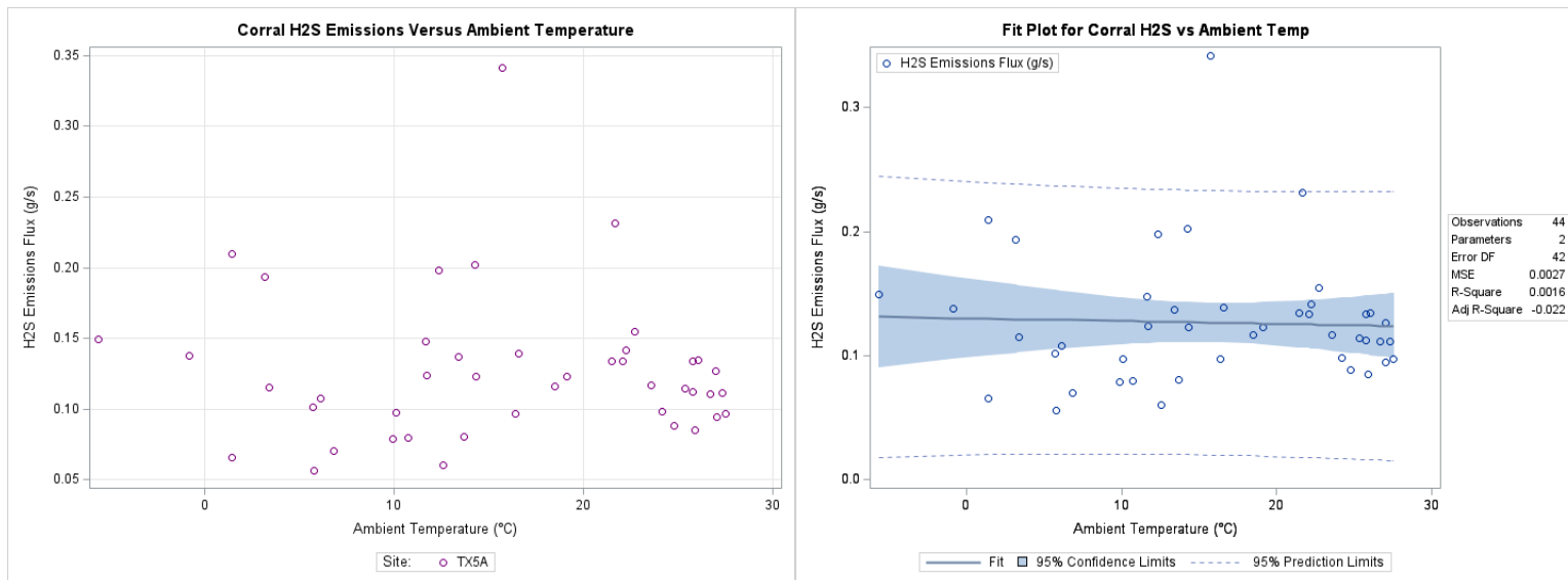
Figure F-137. Scatter plot of corral H 2 S emissions versus ambient temperature and scatter plot with regression.
