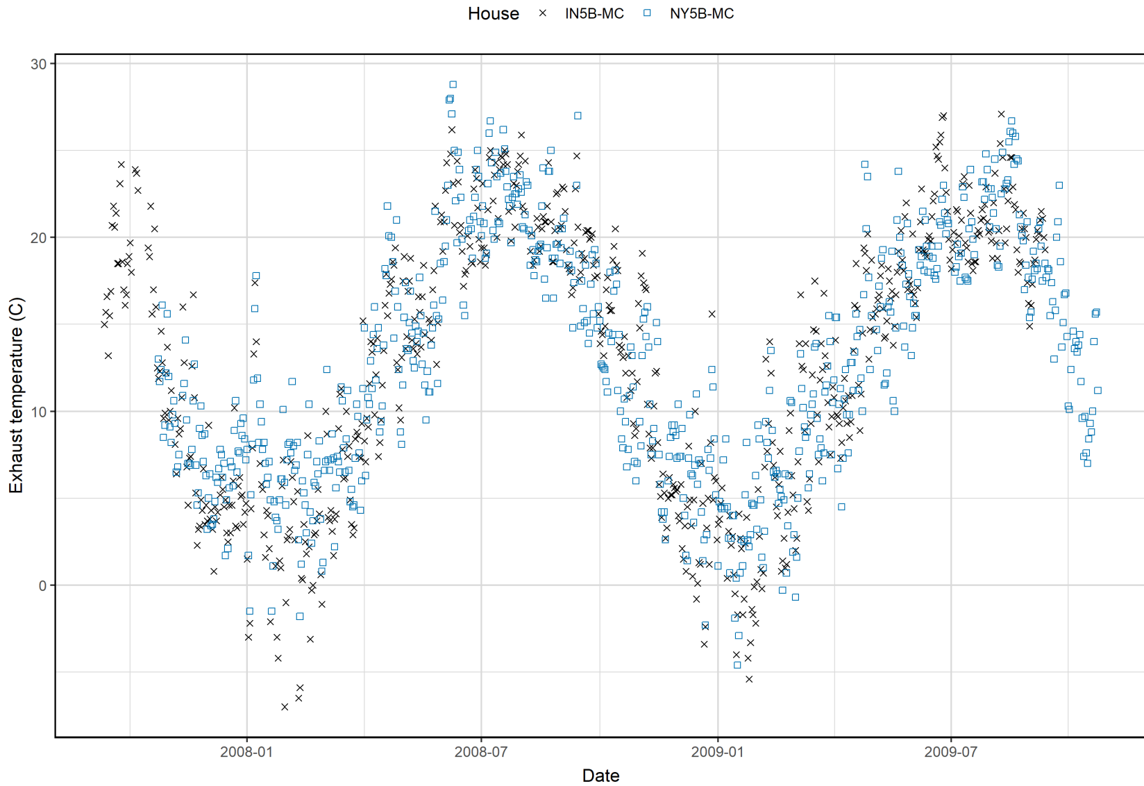
Figure E-22. Trends in exhaust temperature at milking centers, by site, during the NAEMS monitoring period.
