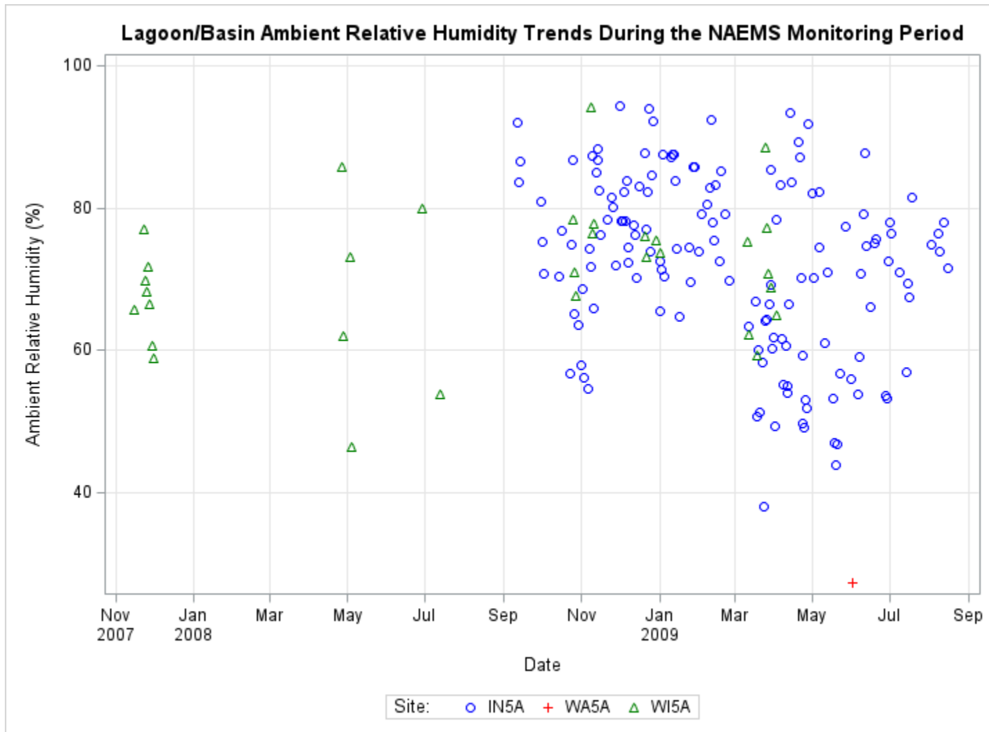
Figure E-50. Trends in ambient relative humidity, by open source site, during the NAEMS monitoring period.
