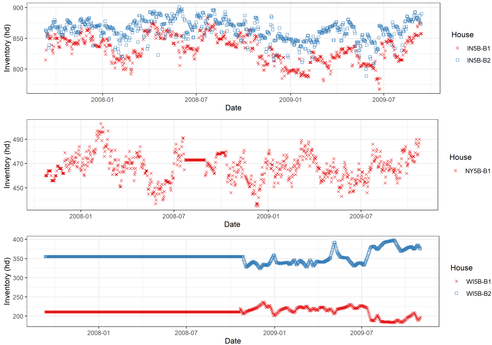
Figure E-6. Trends in inventory at mechanically ventilated barns, by site, during the NAEMS monitoring period.
