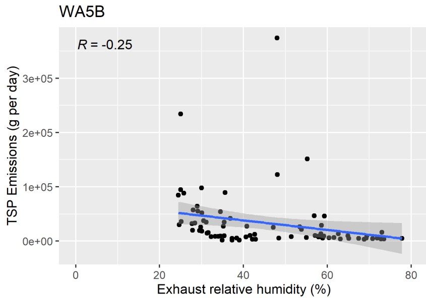
Figure F-105. Scatter plot of naturally ventilated barns TSP emissions versus exhaust relative humidity and scatter plot with regression.
