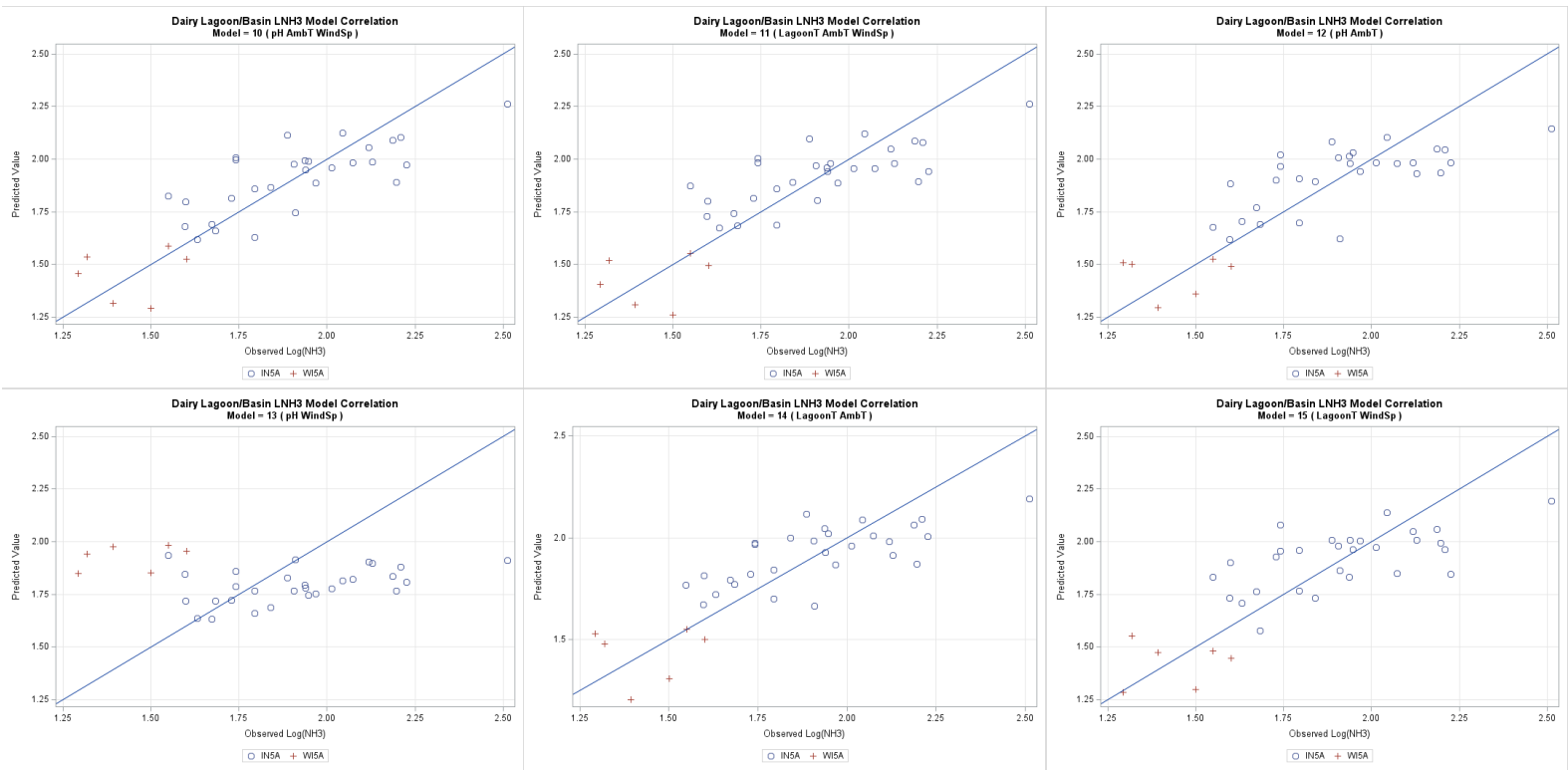
Figure G-68. Dairy lagoon NH 3 one-to-one plots models 10 through 15, log transformed.
