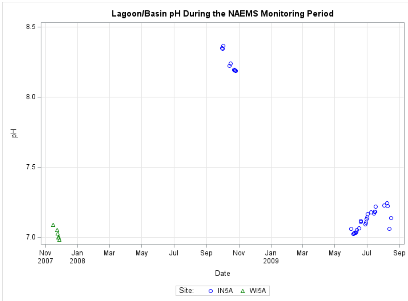
Figure E-48. Trends in pH, by open source site, during the NAEMS monitoring period.
