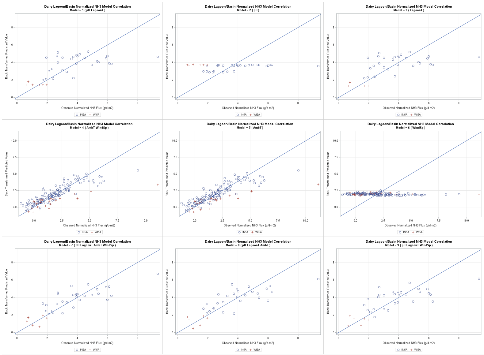
Figure G-69. Dairy lagoon NH 3 one-to-one plots models 1 through 9, back transformed.
