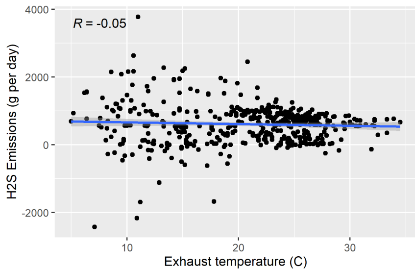
Figure F-97. Scatter plot of naturally ventilated barns H 2 S emissions versus exhaust temperature and scatter plot with regression.
