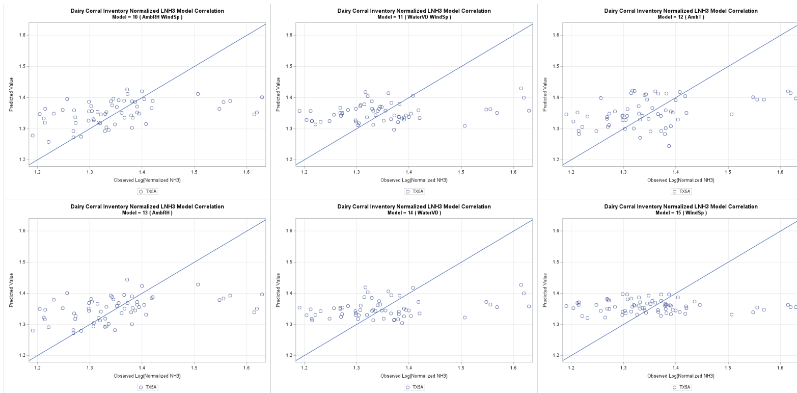
Figure G-78. Dairy corral NH 3 one-to-one plots models 10b through 15b, log transformed.
