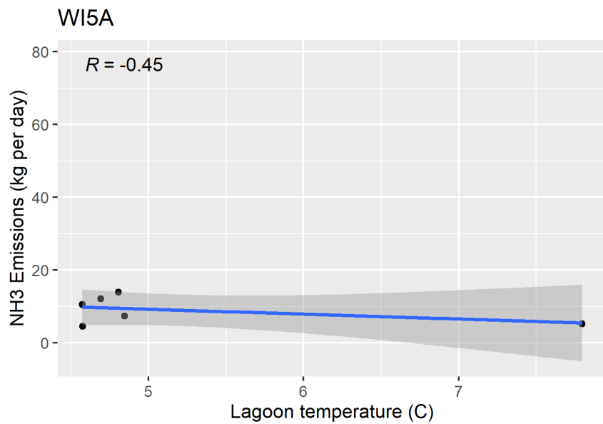
Figure F-126. Scatter plot of lagoon/basin NH 3 emissions versus lagoon temperature and scatter plot with regression.
