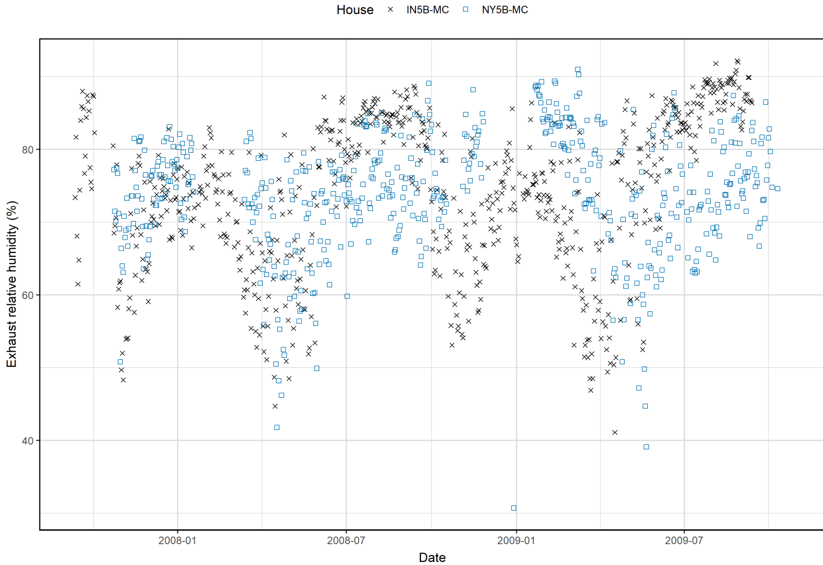
Figure E-23. Trends in exhaust relative humidity at milking centers, by site, during the NAEMS monitoring period.
