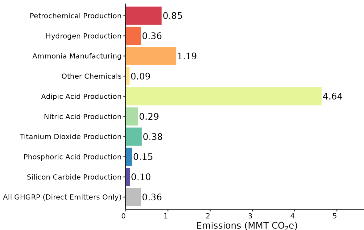
Figure 5: Average Emissions per Reporter from the Chemicals Sector (2021)
