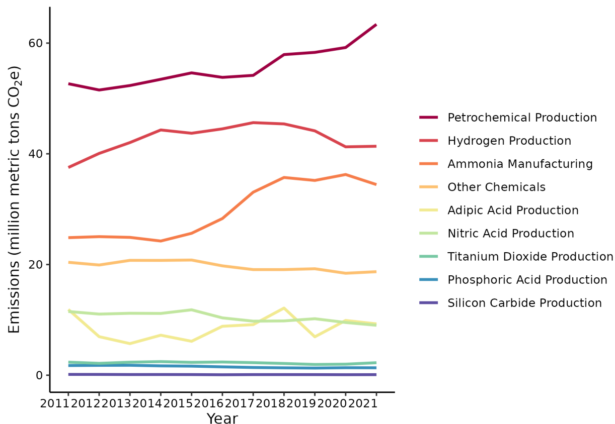
Figure 4: Annual Reported Direct Emissions from the Chemicals Sector, by Subsector (2011-2021)
