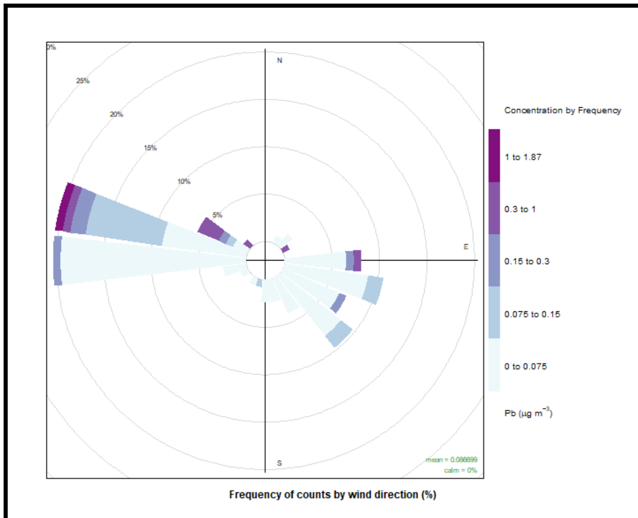
Figure 6: Pollution Rose for Pb Concentrations from Republic Steel Ambient Air Monitoring Site (AQS Site No. 39-151-0024), Canton, Stark County, Ohio
