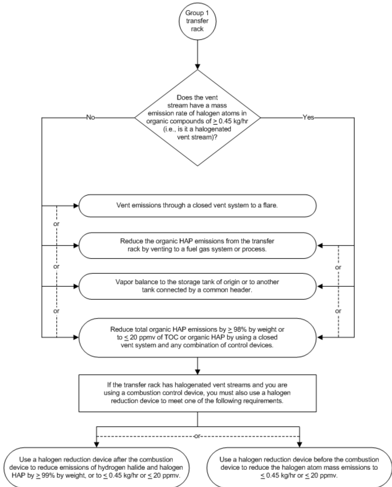
Figure 7-2. Emission limits and work practice standards for Group 1 transfer racks.
