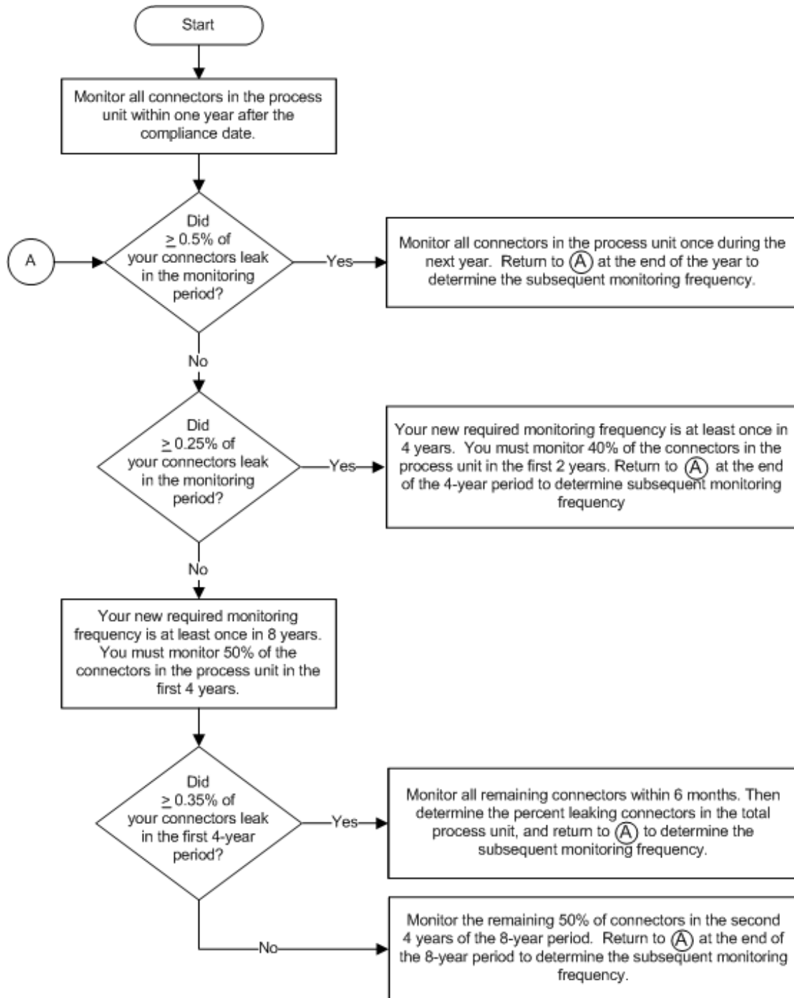
Figure 6-2. Flowchart of monitoring frequencies for connectors in gas/vapor service or light liquid service under subpart UU and the CAR.
