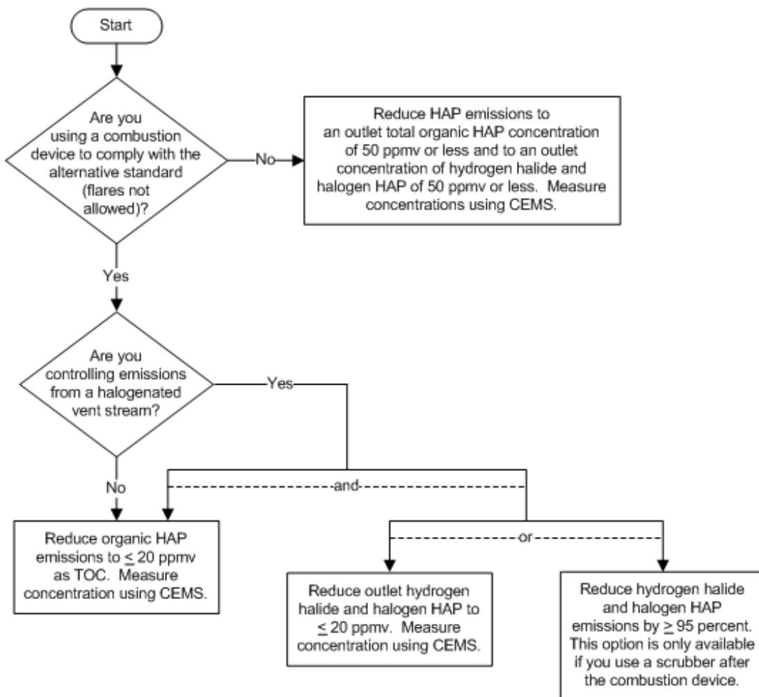
Figure 11-1. Alternative standard for process vents or storage tanks.
