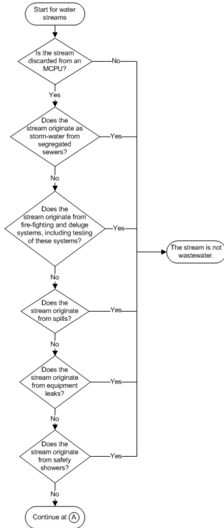
Figure 5-1. Applicability for wastewater.
