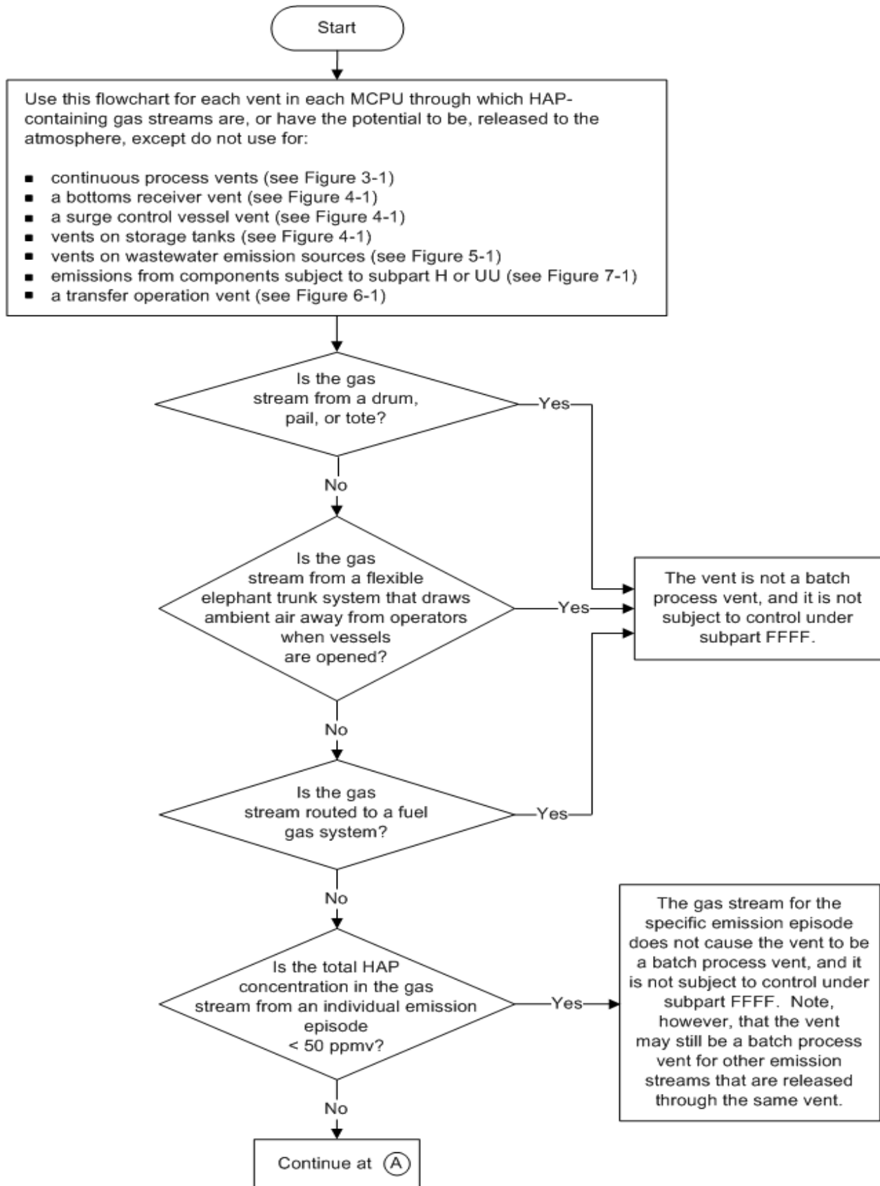
Figure 3-2. Applicability for batch process vents.
