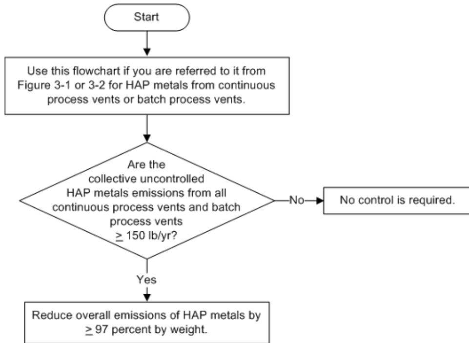
Figure 3-5. Applicability and control requirements for HAP metals emissions from process vents at new sources.
