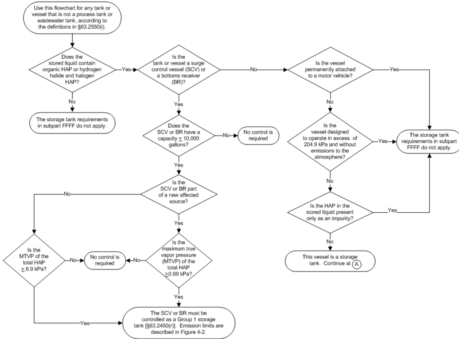
Figure 4-1. Applicability for storage tanks, surge control vessels, and bottoms receivers.
