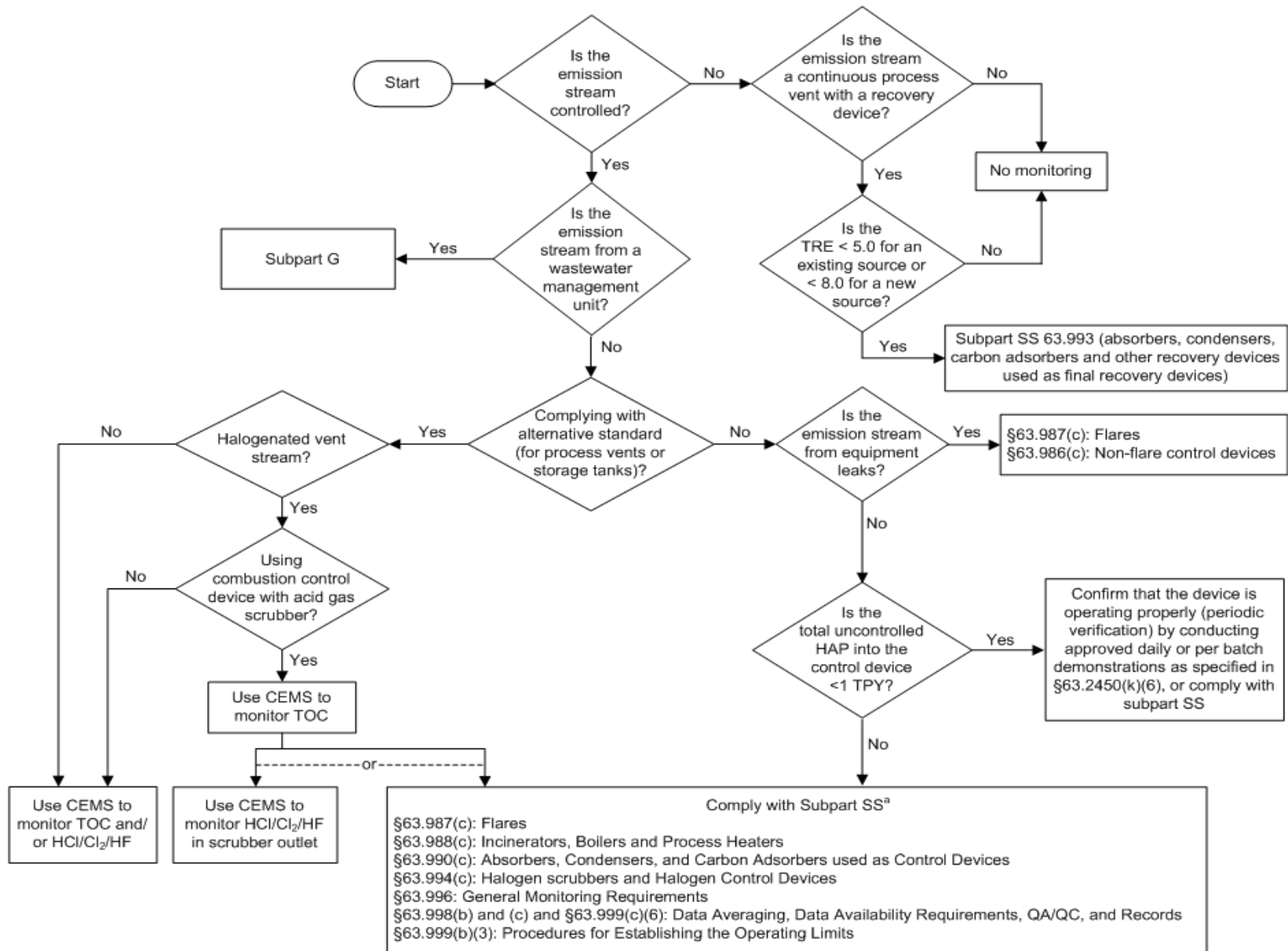
Figure C-2. Monitoring of vent streams.
