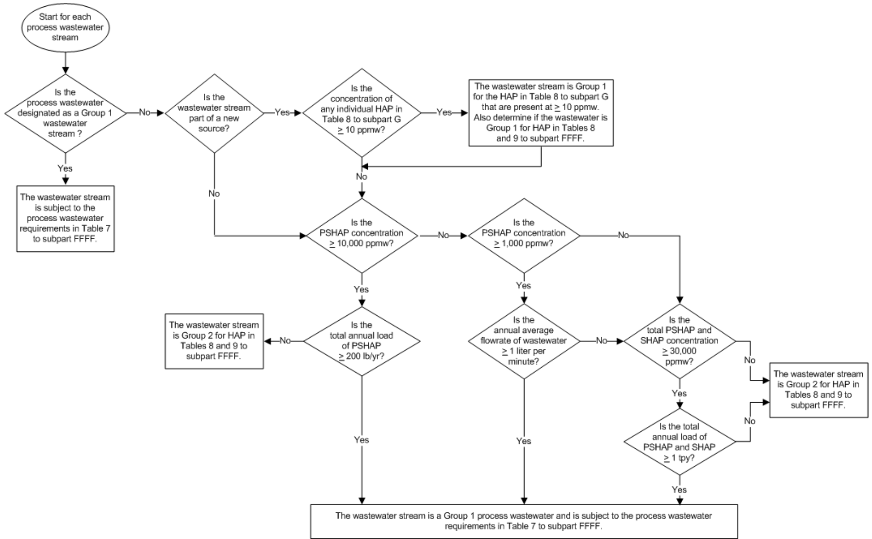
Figure 5-3. Determination of group status for process wastewater streams.
