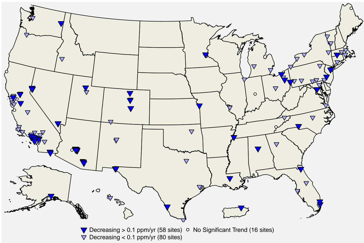
Figure 7: Site-level trends in 8-hour CO design values based on data from 2000 through 2023. Source: AQS, trends computed using R statistical software.
