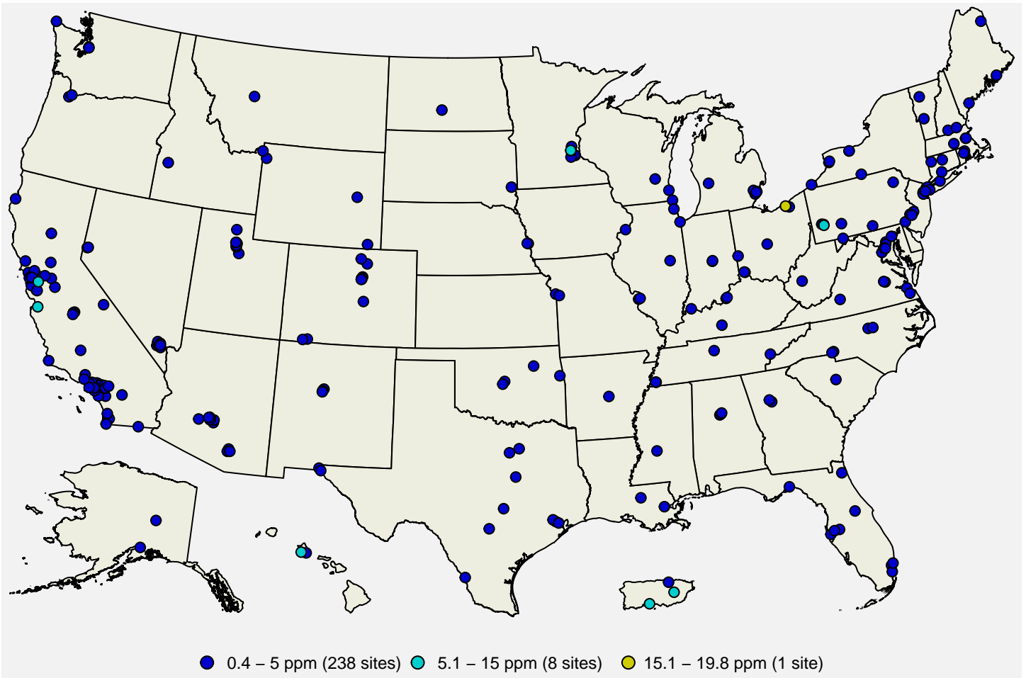
Figure 6: 1-hour CO design values in ppm for the 2022-2023 period. Source: AQS.
