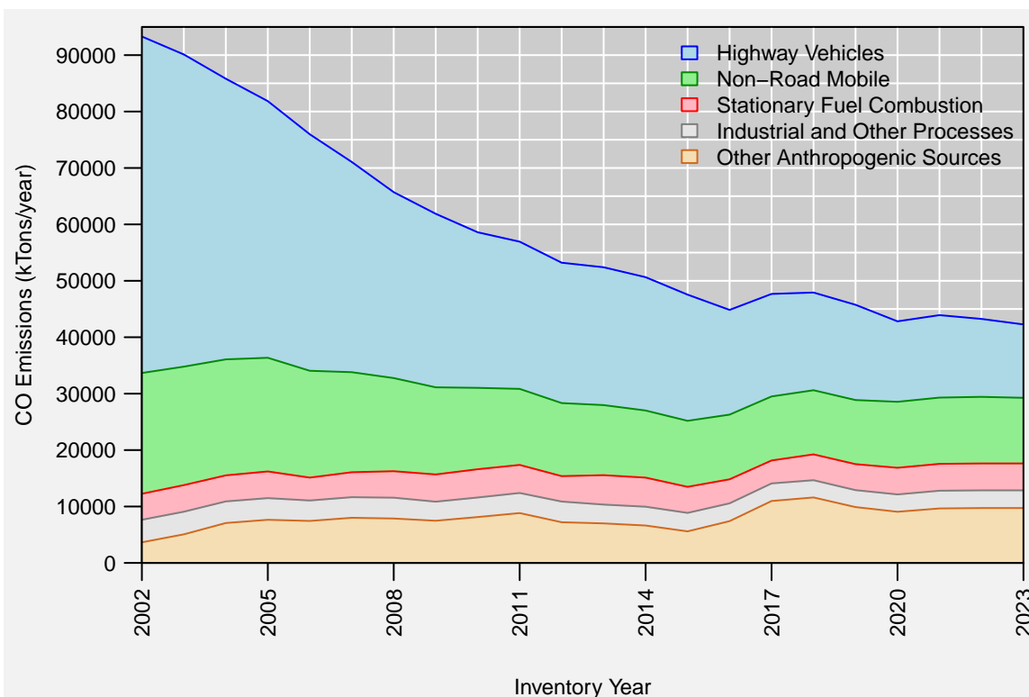
Figure 3. U.S. anthropogenic CO emissions trend, 2002-2023. Source: EPA's Air Pollutant Emissions Trends Data
