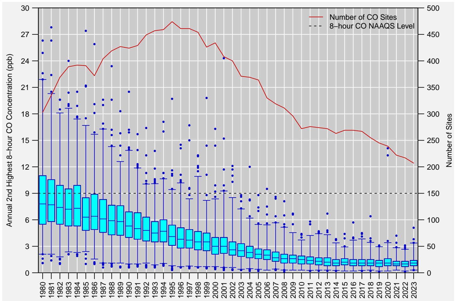
Figure 10: Distribution of annual 2nd highest 8-hour CO concentrations measured at U.S. monitoring sites, 1980 to 2023. Boxes represent the median and interquartile range, whiskers extend to the 1st and 99th percentiles, and values outside this range are shown as circles. The red line shows the number of CO monitoring sites reporting data to EPA in each year. Source: AQS.
