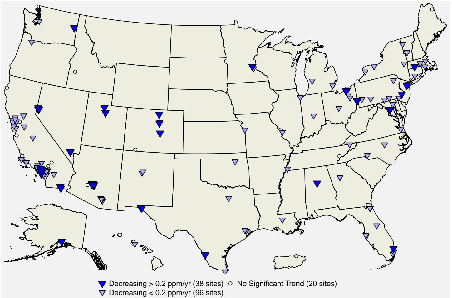
Figure 8: Site-level trends in 1-hour CO design values based on data from 2000 through 2023. Source: AQS, trends computed using R statistical software
