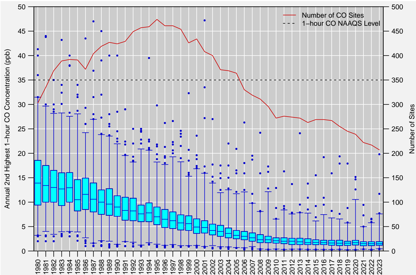
Figure 11: Distribution of annual 2nd highest 1-hour CO concentrations measured at U.S. monitoring sites, 1980 to 2023. Boxes represent the median and interquartile range, whiskers extend to the 1st and 99th percentiles, and values outside this range are shown as circles. The red line shows the number of CO monitoring sites reporting data to EPA in each year. Source: AQS.
