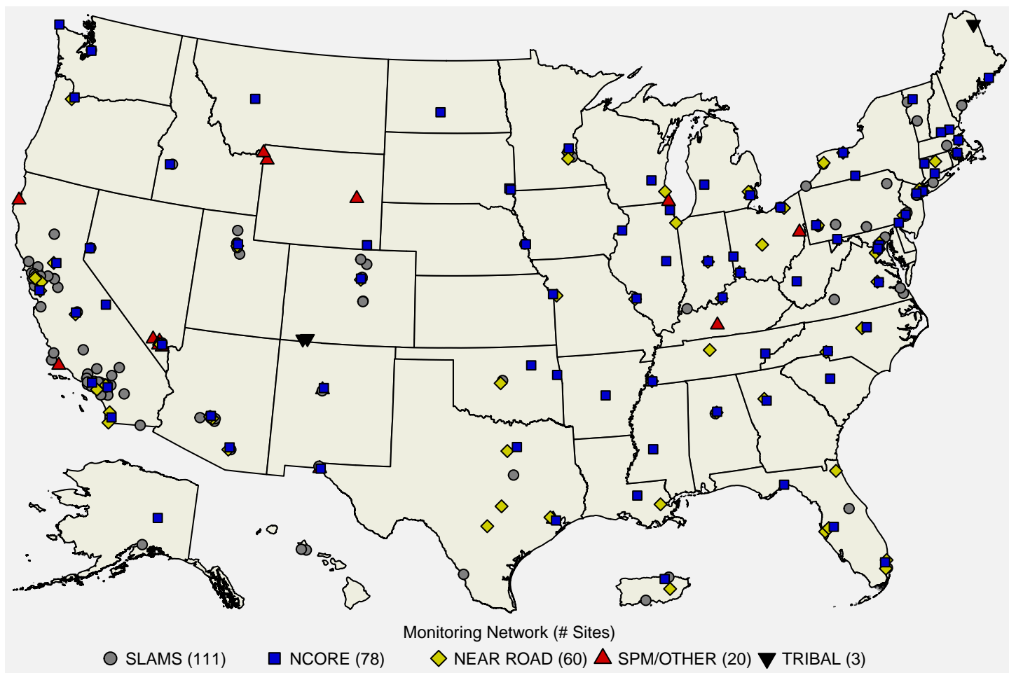
Figure 4: Map of U.S. CO monitoring sites reporting data to the EPA during the 2021-2023 period. Source: AQS.
