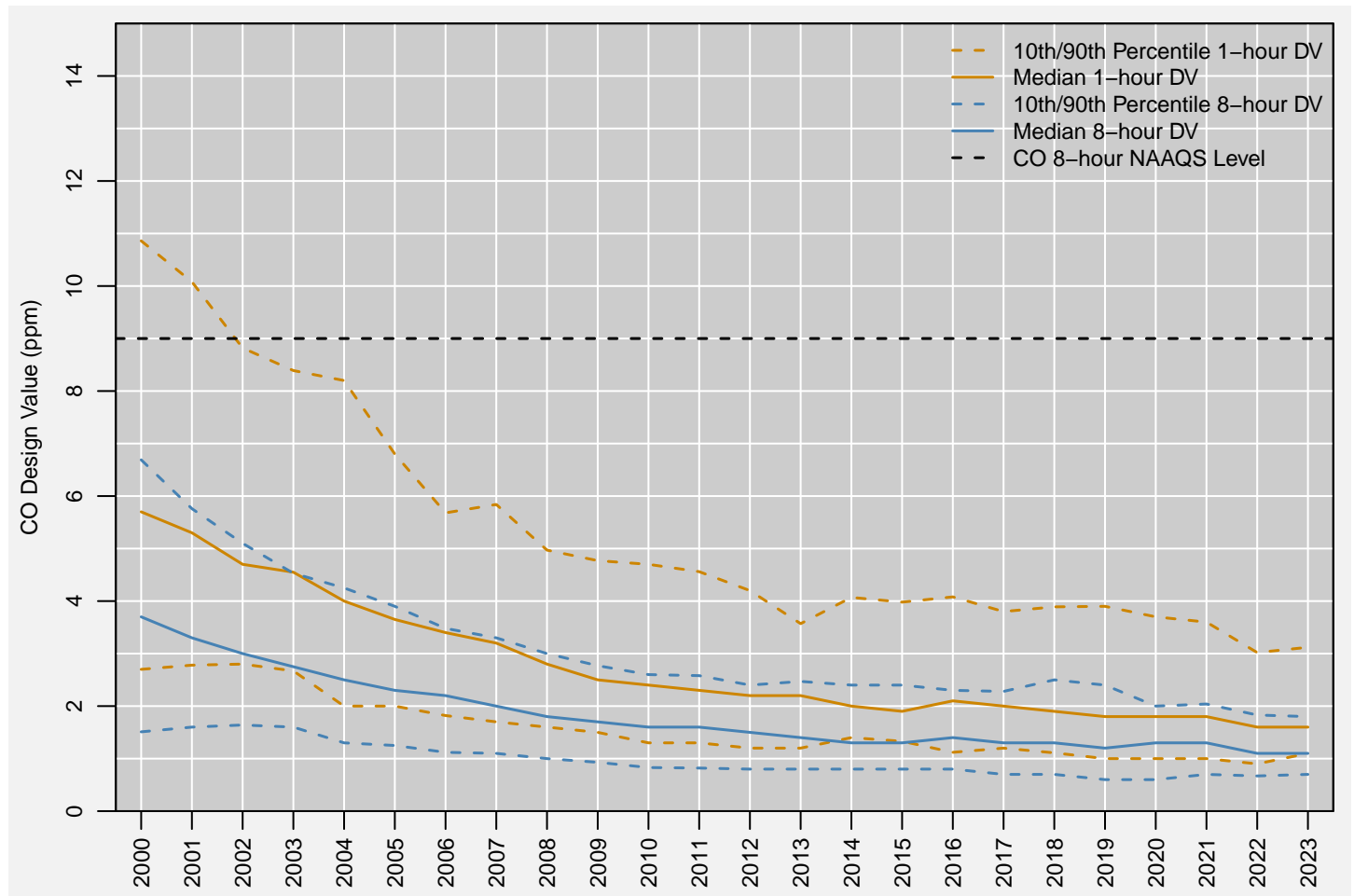
Figure 9: National trends in CO design values in ppm, 2000 to 2023. Source: AQS.
