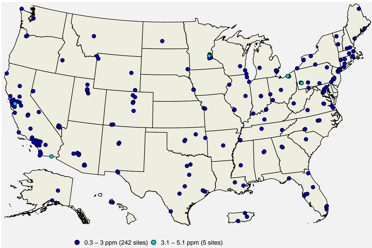
Figure 5: 8-hour CO design values in ppm for the 2022-2023 period. Source: AQS.
